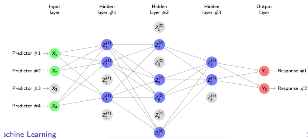
Figure 35: Dropout during training: at each update a random subset of input and hidden units (grey) is dropped, and only the remaining blue sub-network is used to propagate the signal and update the parameters.
