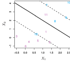
Figure 16: Soft-margin classifier with slack variables \epsilon_i and total budget b .
