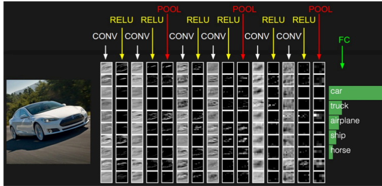
Figure 40: Several convolutional (CONV + ReLU + POOL) layers stacked before a final fully connected classifier.
