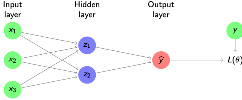
Figure 31: Forward pass for one training example (x, y) : the input is propagated through the hidden layer to the output and the loss L(\theta) is computed.
