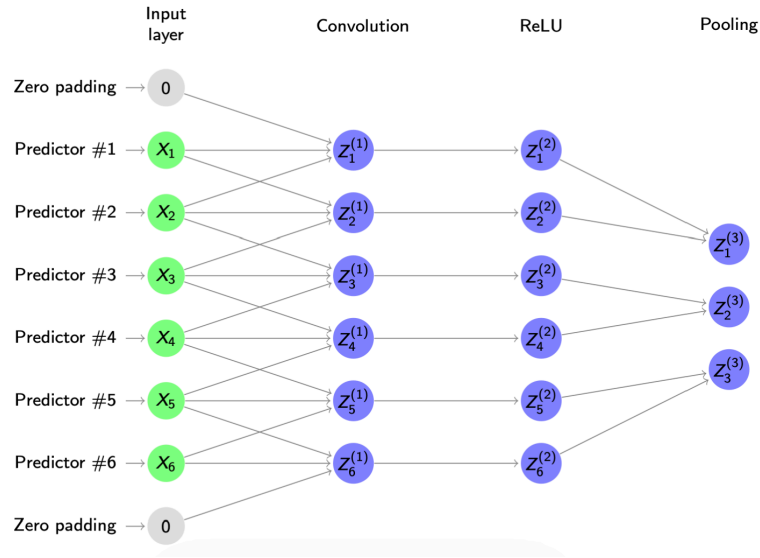
Figure 44: 1D toy example of a convolutional layer with zero-padding, convolution, ReLU and pooling, illustrating weight sharing and the small number of parameters.
