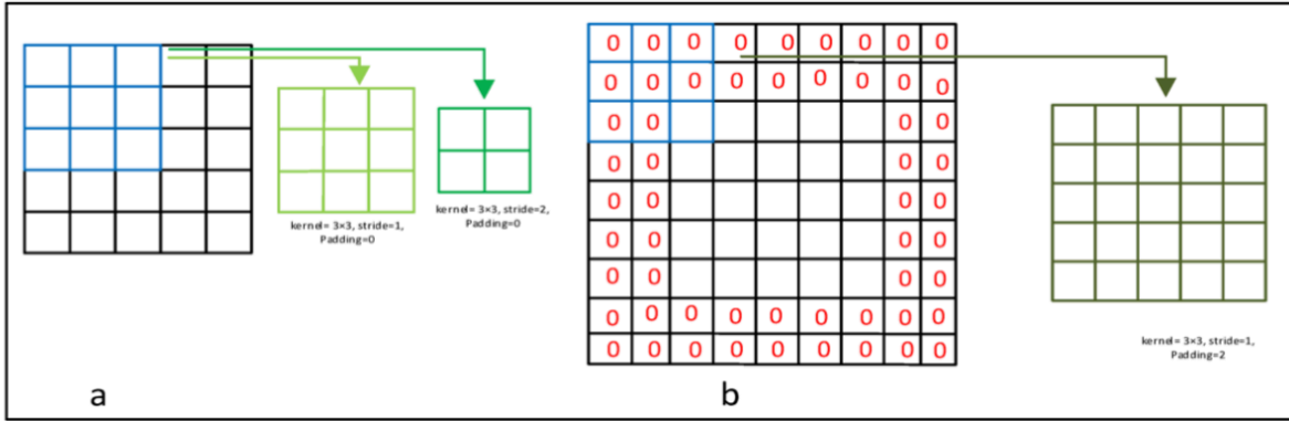
Figure 38: Convolution hyperparameters: (a) effect of stride on output size; (b) zero-padding to keep input and output sizes the same.
