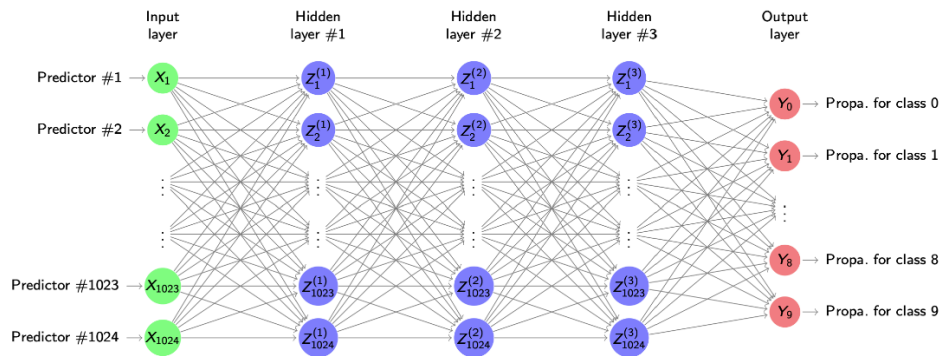
Figure 35: Dense fully connected neural network for CIFAR-10 classification
