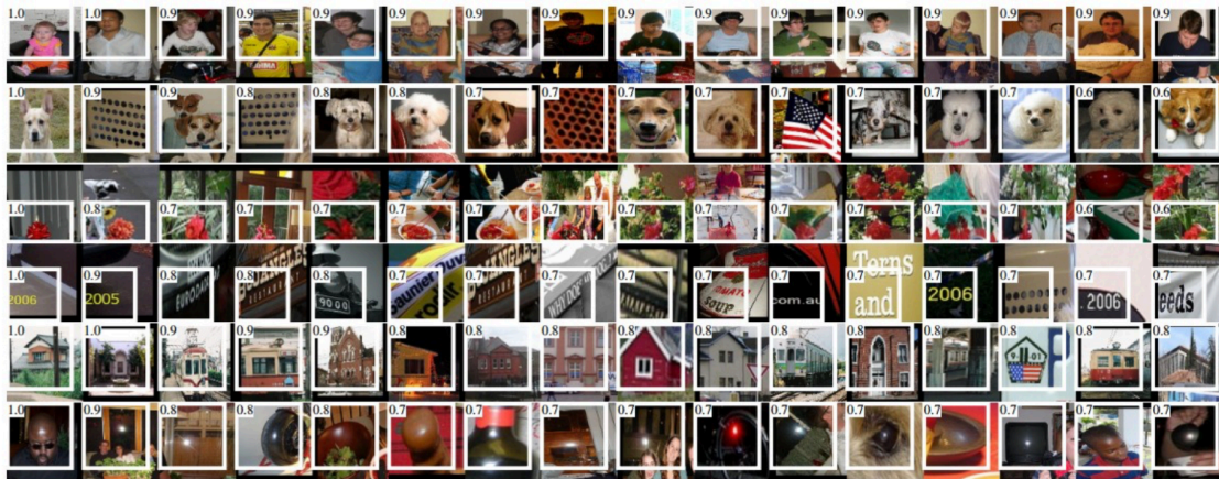
Figure 49: Images that maximally activate six neurons in a deep pooling layer of AlexNet, showing specialisation to faces, dogs, text, houses and other high-level patterns.
