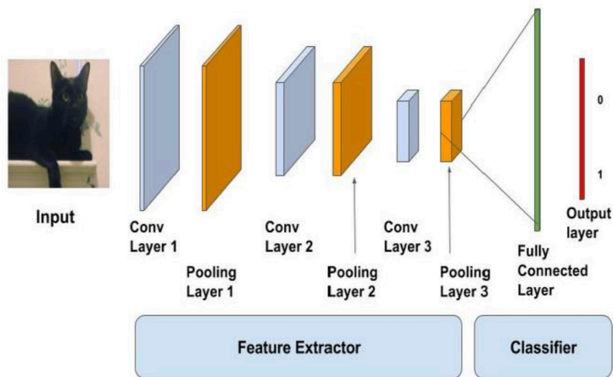
Figure 50: Transfer learning: reuse the convolutional feature extractor and retrain a new task-specific classifier on top.
