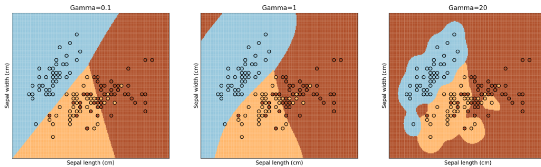
Figure 20: Decision boundaries of radial-kernel SVMs on the Iris dataset for different \gamma values.
