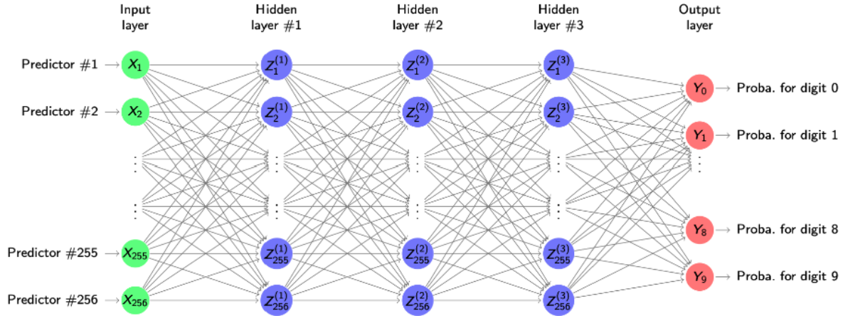
Figure 30: Fully connected deep neural network with three hidden layers of width 256 for digit classification.
