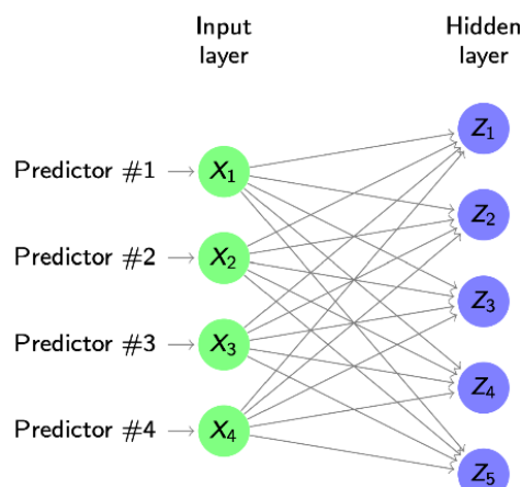
Figure 23: Single hidden layer neural network: inputs X_1, \dots, X_p are linearly combined and passed through an activation function to form hidden units Z_1, \dots, Z_m .
