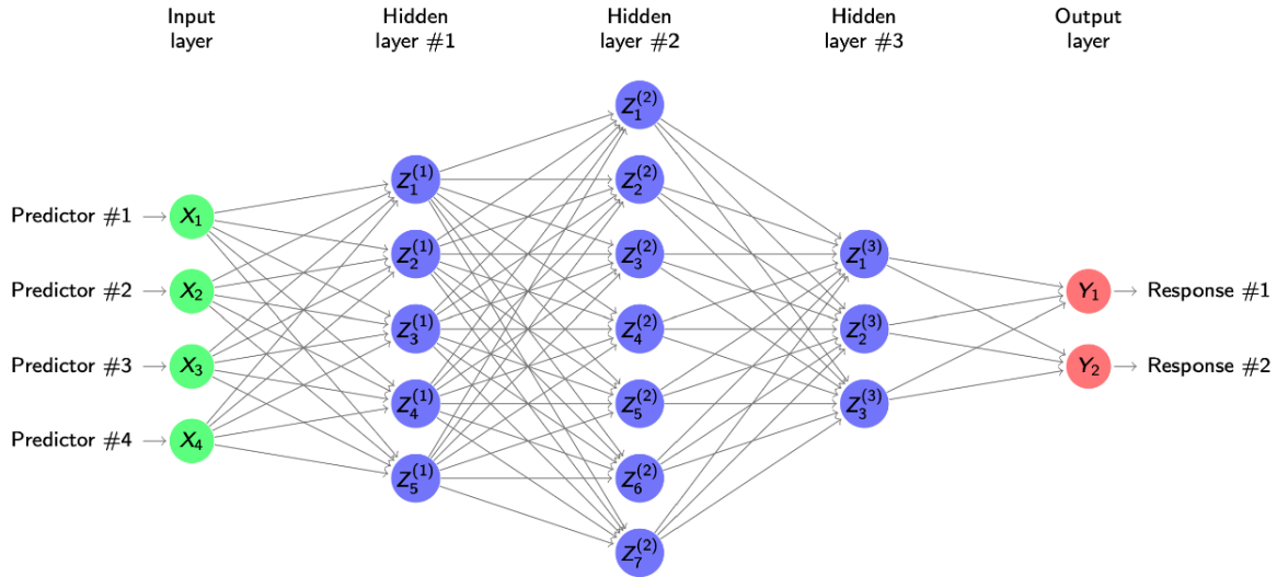
Figure 28: Deep neural network with several hidden layers between input and output: each hidden layer applies a linear transformation followed by a non-linear activation to the previous layer.
