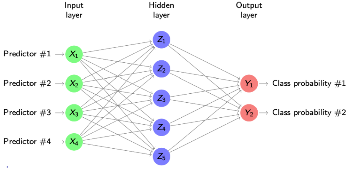
Figure 27: Single hidden layer neural network for classification: one output neuron per class, each modelling a class probability.
