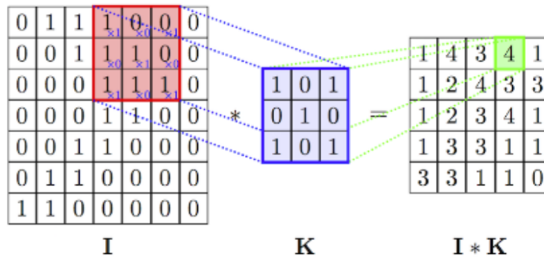
Figure 37: Illustration of a 3 \times 3 convolution: a receptive field in the input image I is combined with a filter K to produce one entry of the convolved image I * K .
