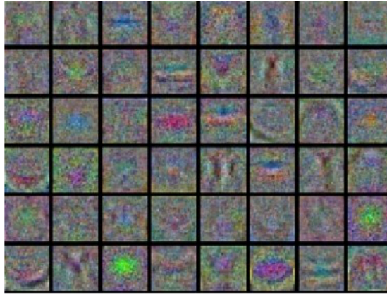
Figure 48: Example of unconverged first-layer filters that look noisy and do not exhibit clear edge or blob patterns.
