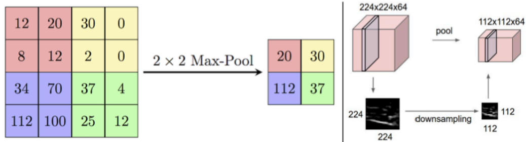
Figure 39: Detector (ReLU) and 2 \times 2 max-pooling: local downsampling of activation maps and reduction from 224 \times 224 \times 64 to 112 \times 112 \times 64 .
