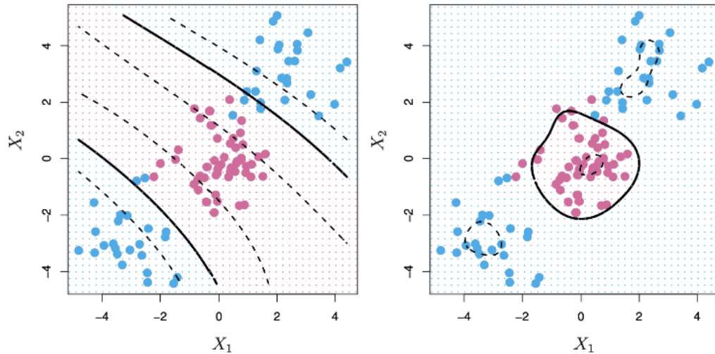
Figure 19: Polynomial and radial kernels producing different decision boundaries.
