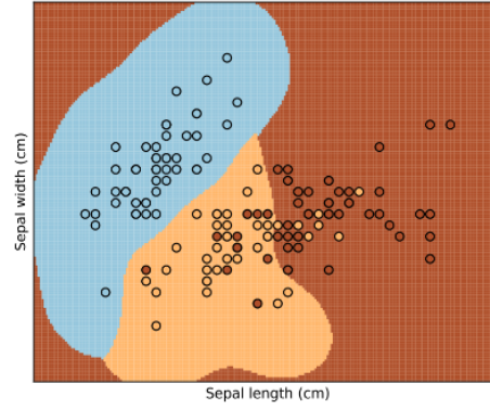
Figure 22: Optimal decision boundary obtained by tuning the parameters C and \gamma via cross-validation.
