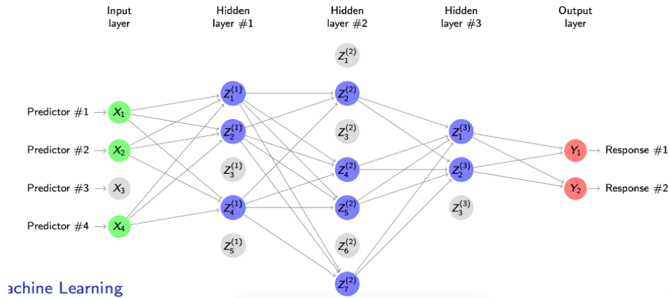
Figure 33: Dropout as an implicit ensemble: across many training steps, different thinned networks are fitted, and the final predictor behaves like an average over these models.
