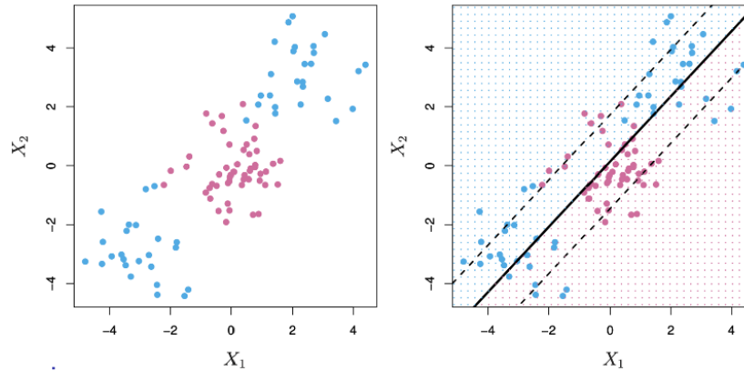
Figure 18: Illustration of the kernel trick: linear kernel case and conceptual extension to non-linear kernels.
