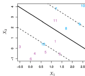
Figure 16: Soft-margin classifier with slack variables \epsilon_i and total budget b .
