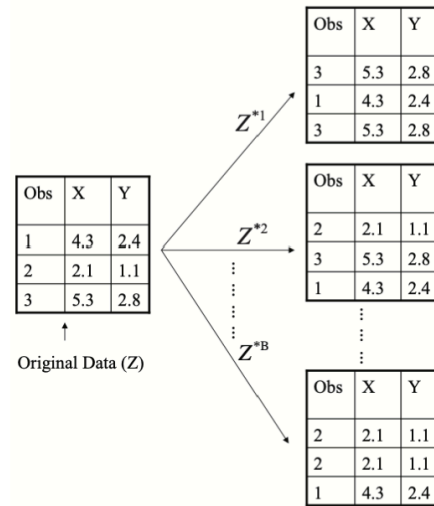
Figure 1: Bootstrap sampling
