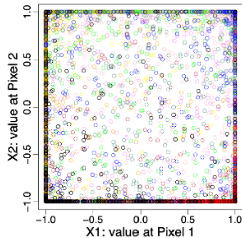
Figure 38: Ten-class classification using two pixel predictors
