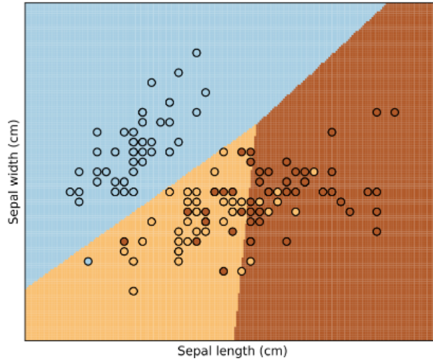
Figure 33: LDA decision regions for the Iris data using two predictors (sepal length and sepal width).
