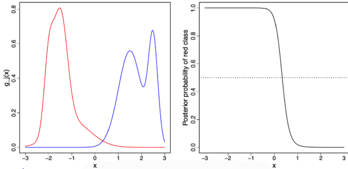
Figure 35: Even with non-Gaussian class densities (left), LDA yields smooth, stable posterior probabilities (right).
