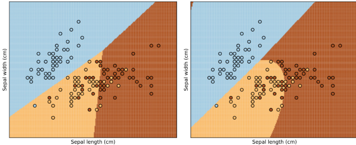
Figure 34: Comparison between LDA (left) and QDA (right) decision regions on the Iris data set.
