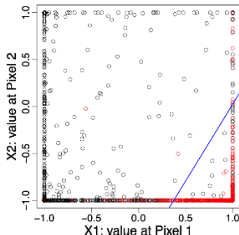
Figure 37: Two-class classification using two pixel predictors
