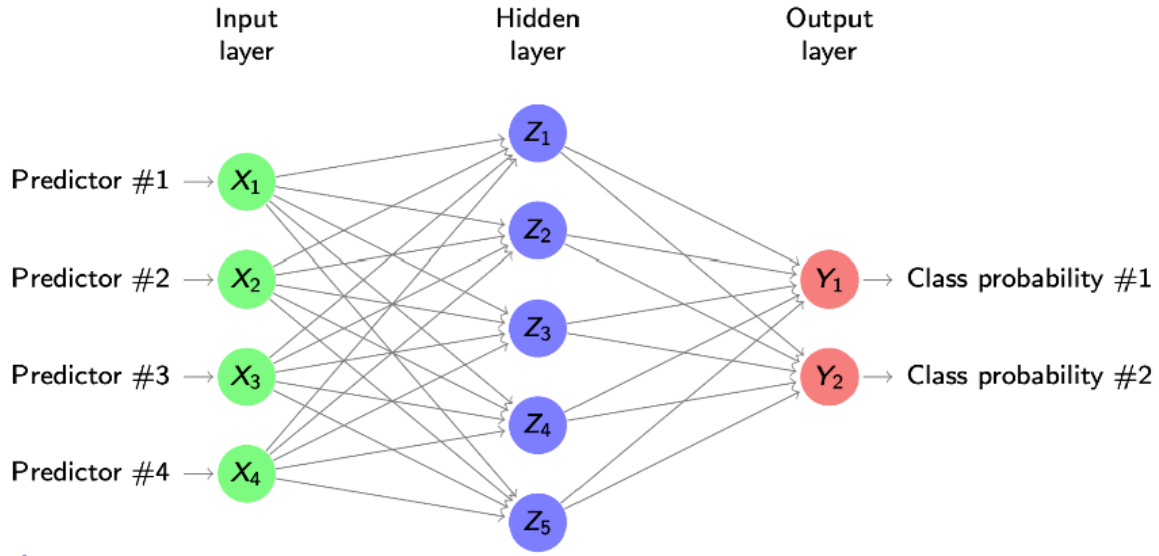
Figure 30: Single hidden layer neural network for classification: one output neuron per class, each modelling a class probability.
