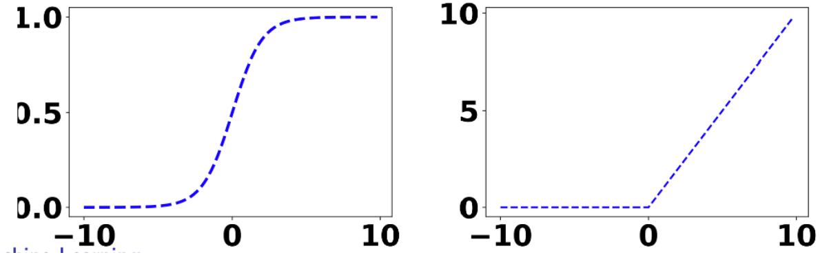
Figure 28: Sigmoid activation (left) and ReLU activation (right) as typical choices for the hidden layer non-linearity.
