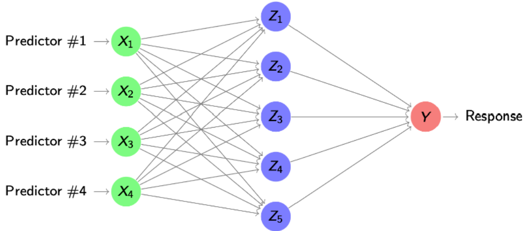
Figure 26: Single hidden layer neural network for regression: the hidden units Z_1, \dots, Z_m are combined linearly in the output neuron to produce the prediction for Y .
