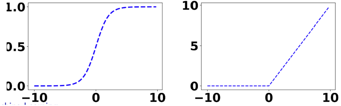
Figure 29: Sigmoid activation (left) and ReLU activation (right) as typical choices for the hidden layer non-linearity.
