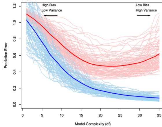
Figure 13: Training versus test error
