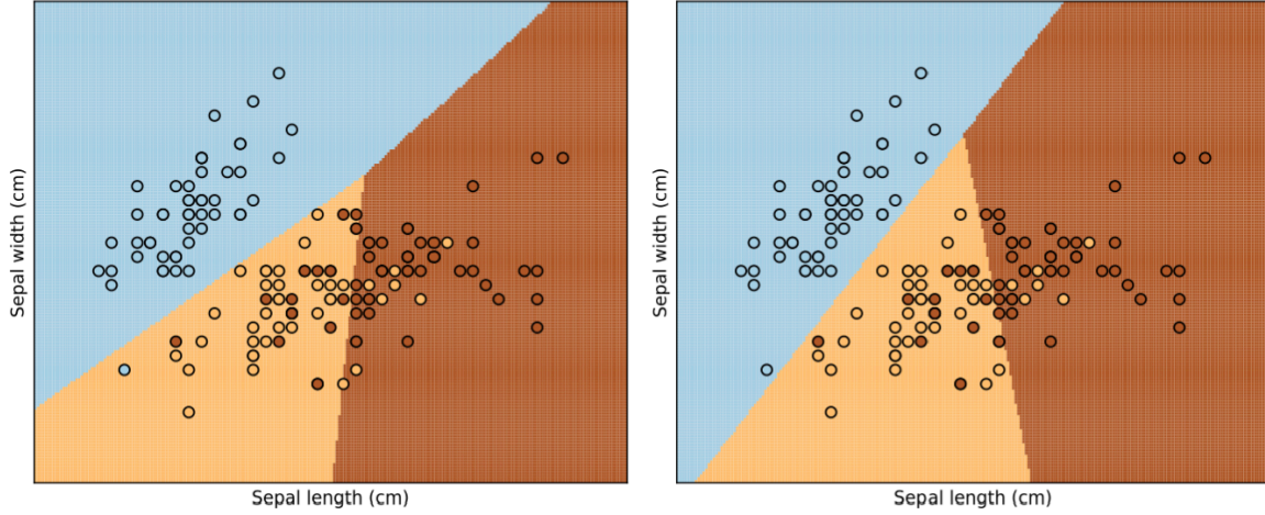
Figure 39: Decision regions obtained by multinomial logistic regression on the Iris data set.
