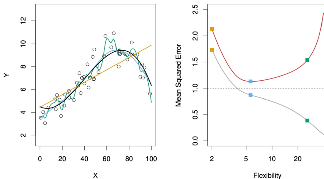
Figure 11: Training versus test errors
