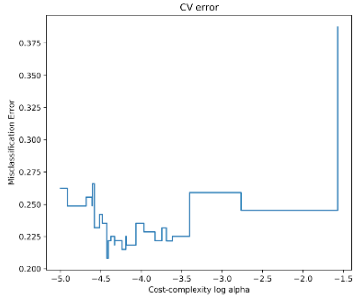
Figure 39: Cross-validation error plot
