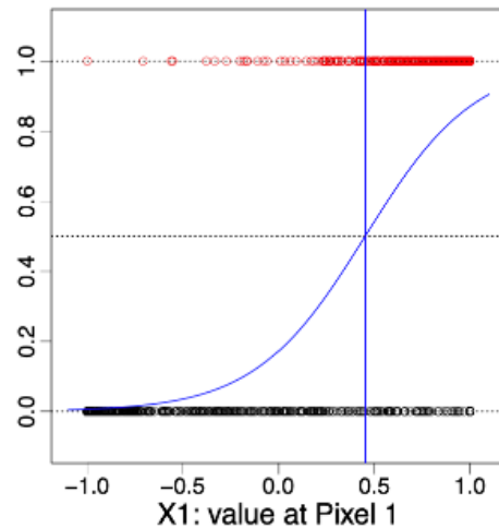
Figure 24: Two-class classification using a single pixel as predictor
