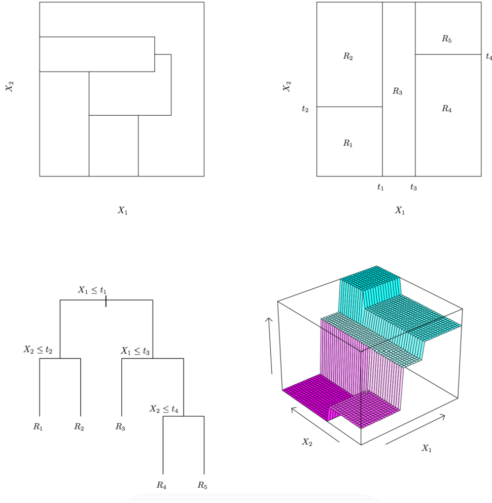
Figure 32: Two-dimensional feature space partition and corresponding regression tree
