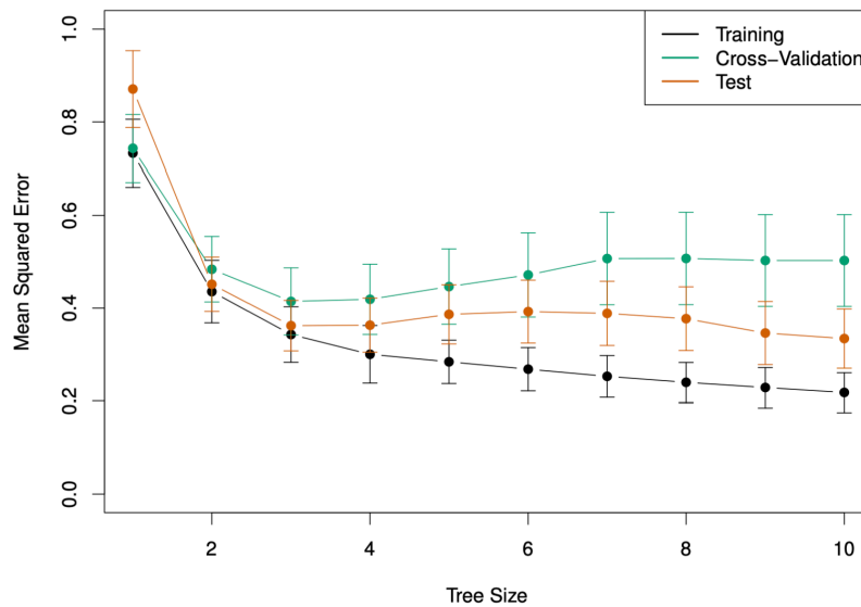
Figure 34: Cross-validation and test errors for trees of increasing size
