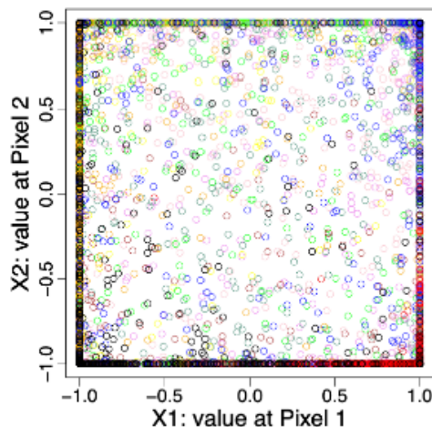
Figure 26: Ten-class classification using two pixel predictors
