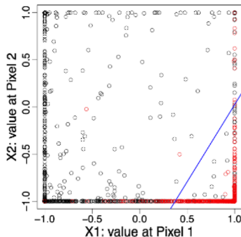
Figure 25: Two-class classification using two pixel predictors
