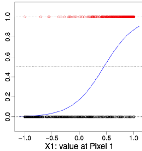
Figure 40: Two-class classification using a single pixel as predictor
