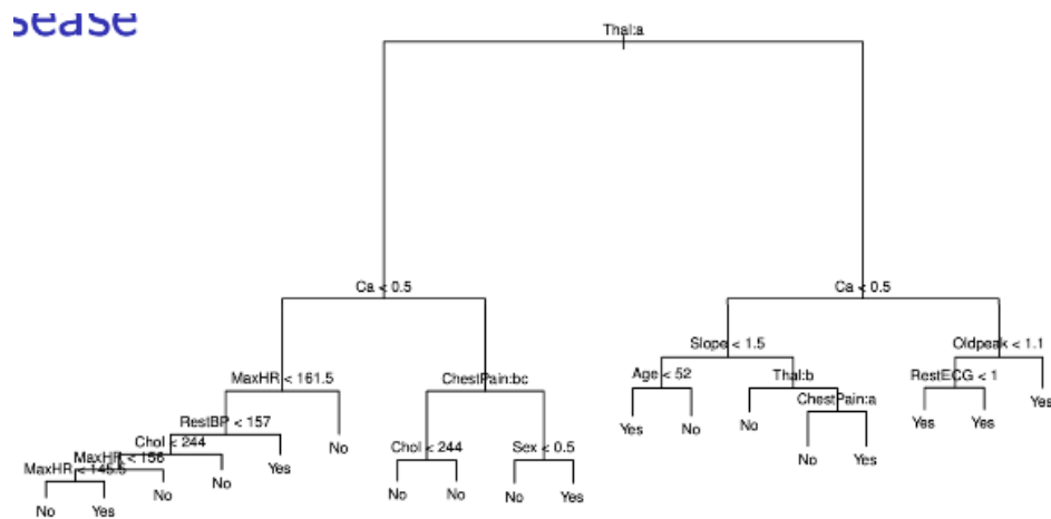
Figure 48: Unpruned tree
