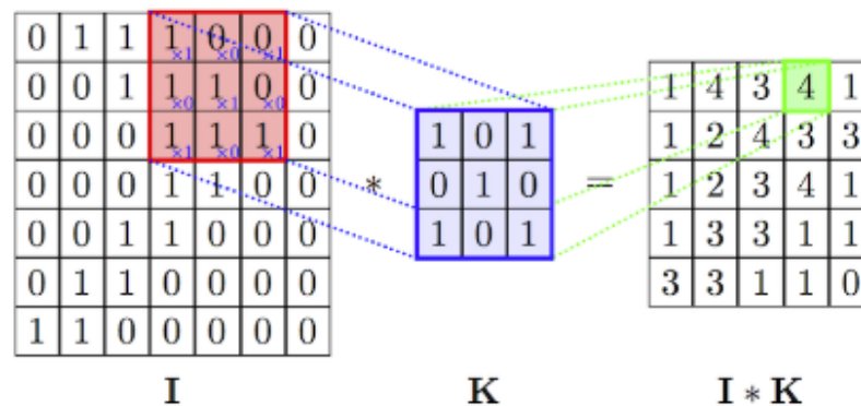
Figure 38: Illustration of a 3 \times 3 convolution: a receptive field in the input image I is combined with a filter K to produce one entry of the convolved image I * K .
