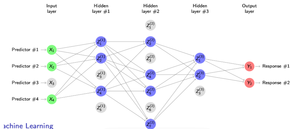
Figure 34: Dropout as an implicit ensemble: across many training steps, different thinned networks are fitted, and the final predictor behaves like an average over these models.
