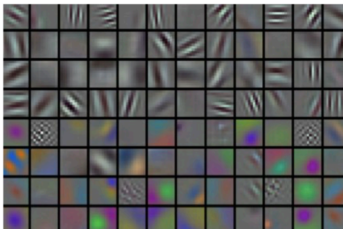
Figure 48: Typical first-layer filters of a CNN trained on natural images. Many resemble oriented edge detectors or small colour blobs.
