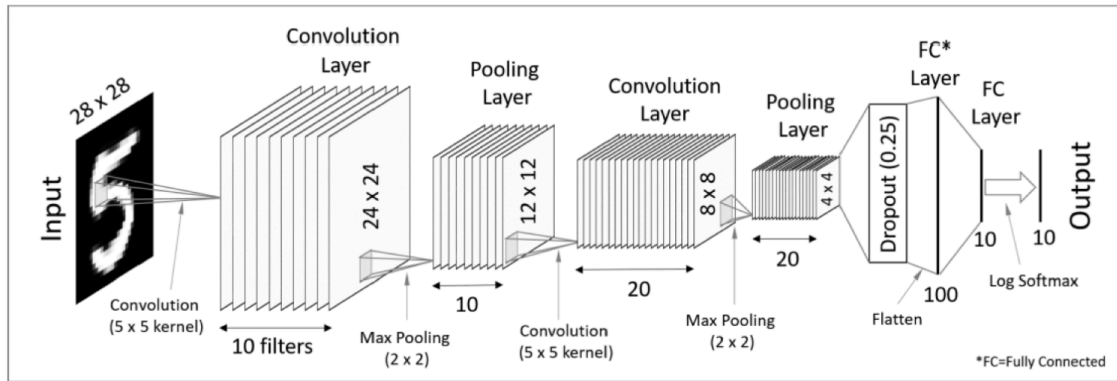
Figure 46: Example of a typical CNN architecture for MNIST digits, with two convolution–pooling blocks followed by flattening and fully connected layers.
