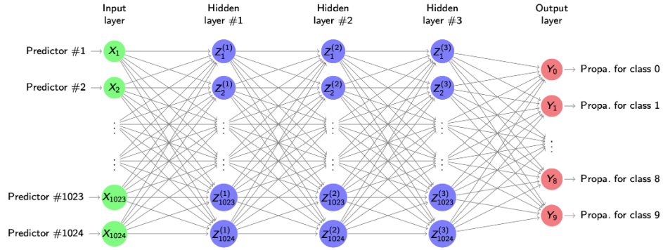
Figure 36: Dense fully connected neural network for CIFAR-10 classification
