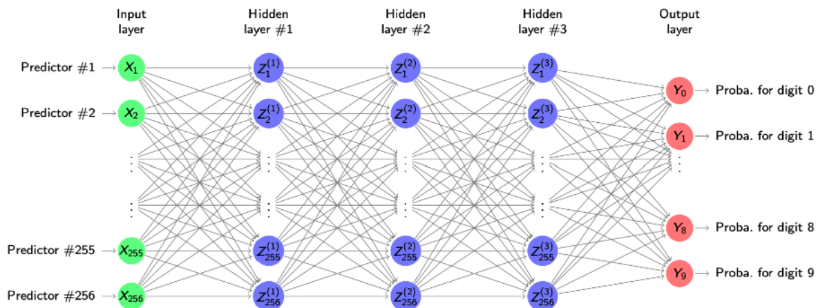
Figure 30: Fully connected deep neural network with three hidden layers of width 256 for digit classification.
