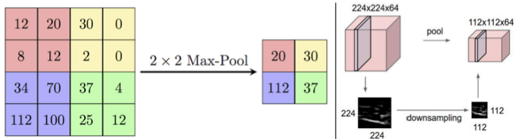
Figure 40: Detector (ReLU) and 2 \times 2 max-pooling: local downsampling of activation maps and reduction from 224 \times 224 \times 64 to 112 \times 112 \times 64 .
