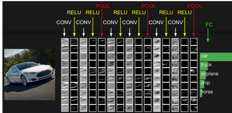
Figure 41: Several convolutional (CONV + ReLU + POOL) layers stacked before a final fully connected classifier.
