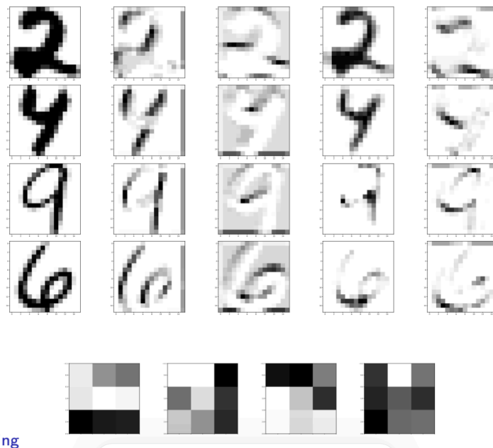
Figure 47: Activations and filters of the first convolutional layer: each row shows an input digit, the corresponding activation maps of several filters, and examples of the learned filters themselves.
