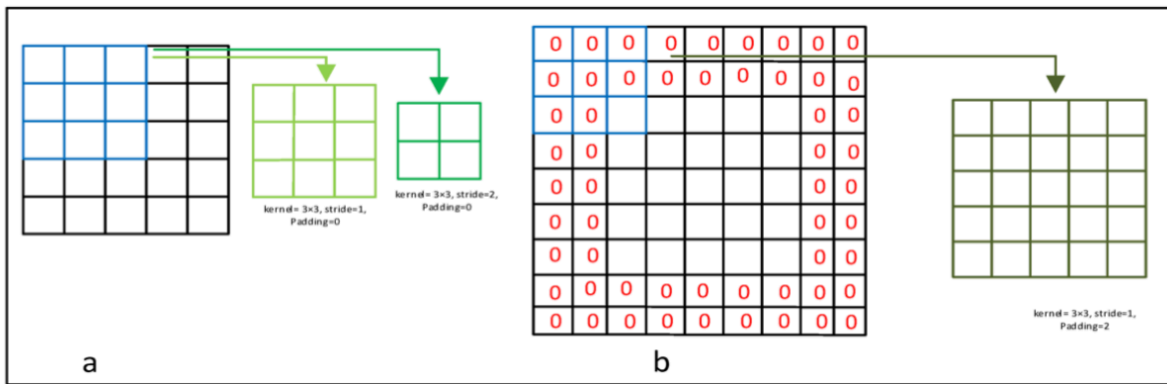
Figure 39: Convolution hyperparameters: (a) effect of stride on output size; (b) zero-padding to keep input and output sizes the same.
