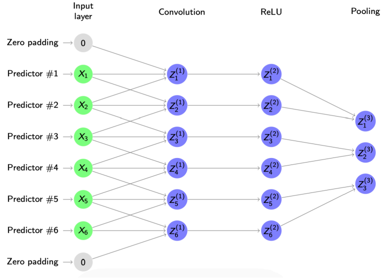
Figure 45: 1D toy example of a convolutional layer with zero-padding, convolution, ReLU and pooling, illustrating weight sharing and the small number of parameters.
