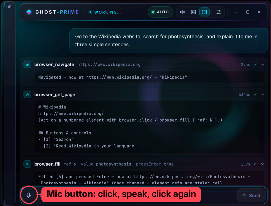
The Ghost-Prime app during the photosynthesis demo.
