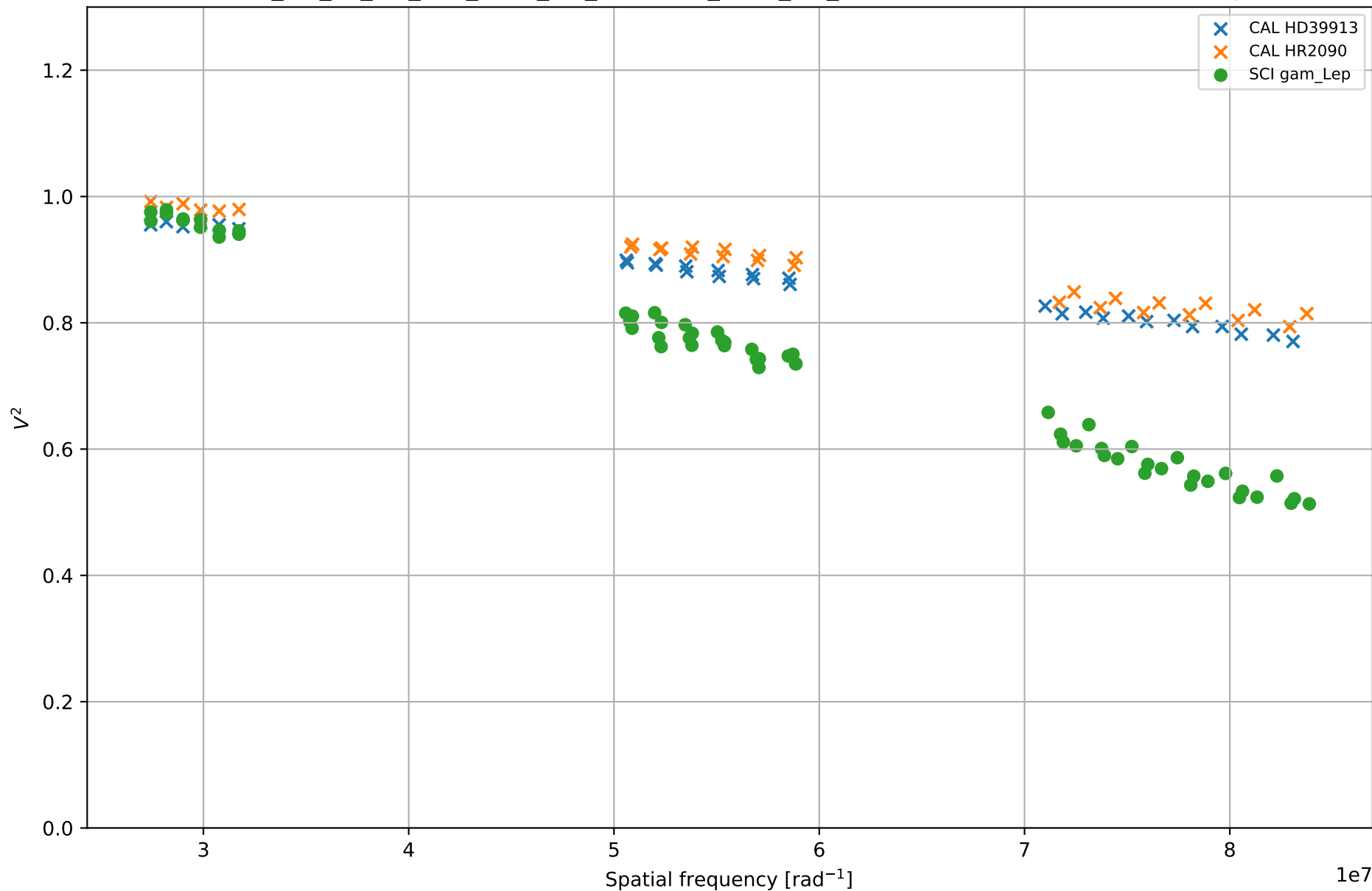
gam_Lep - calibrated experiment data GAMLEP_NO_BL_NO_CAL_P104_NO_HD38579_P106_NO_HD38295 - 2020-01-03 - bootstrap 00
