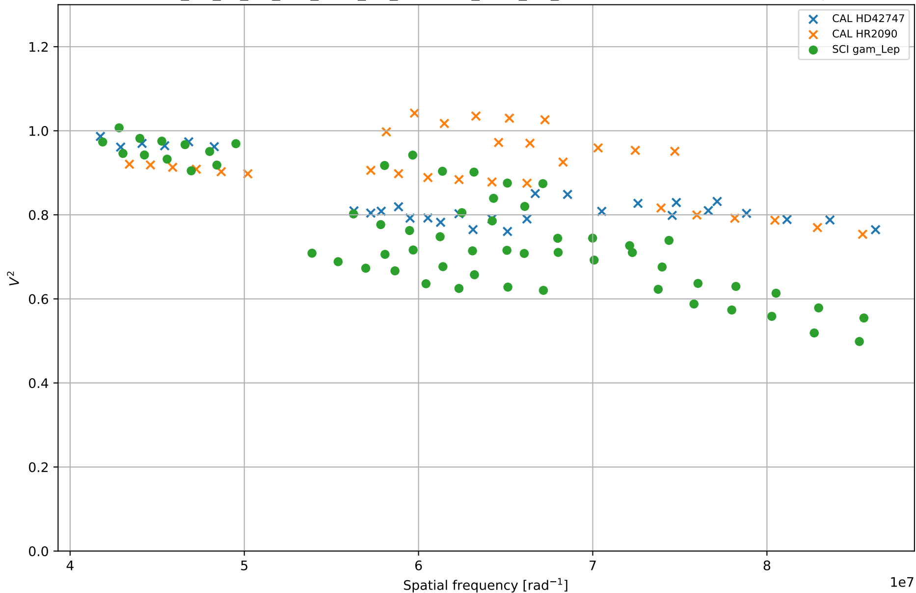
gam_Lep - calibrated experiment data GAMLEP_NO_BL_NO_CAL_P104_NO_HD38579_P106_NO_HD38295 - 2021-02-18 - bootstrap 00
