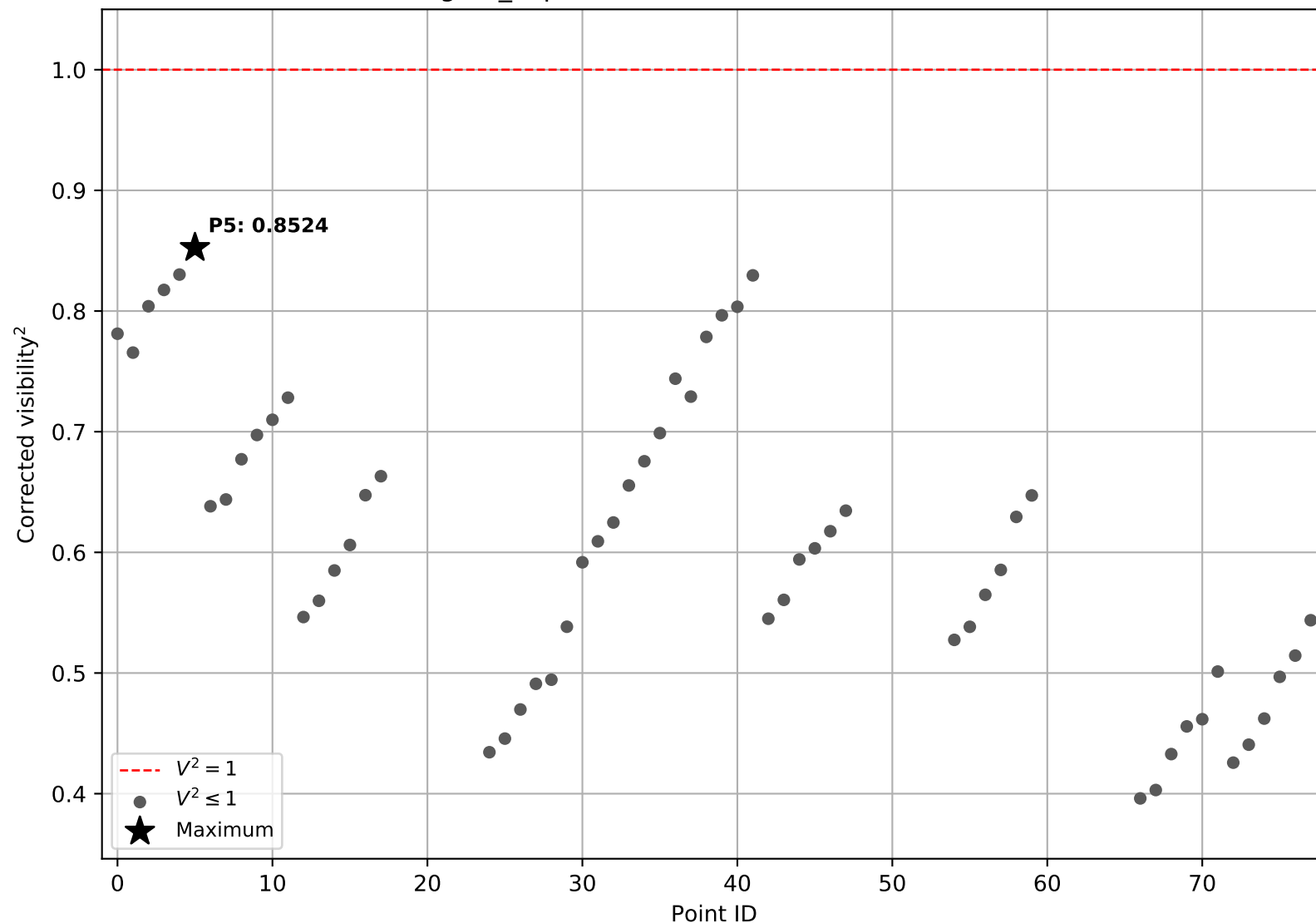
gam_Lep, faint, 106: corrected V2 values
