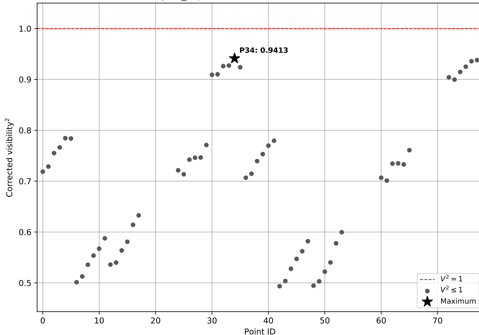
gam_Lep, faint, 104: corrected V2 values
