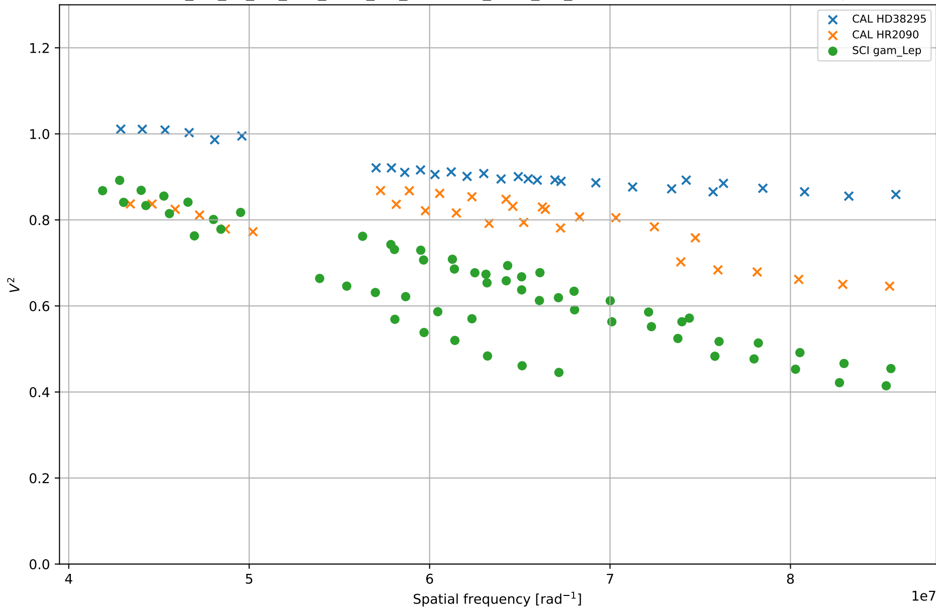
gam_Lep - calibrated experiment data GAMLEP_NO_BL_NO_CAL_P104_NO_HD39913_P106_NO_HD42747 - 2021-02-18 - bootstrap 00
