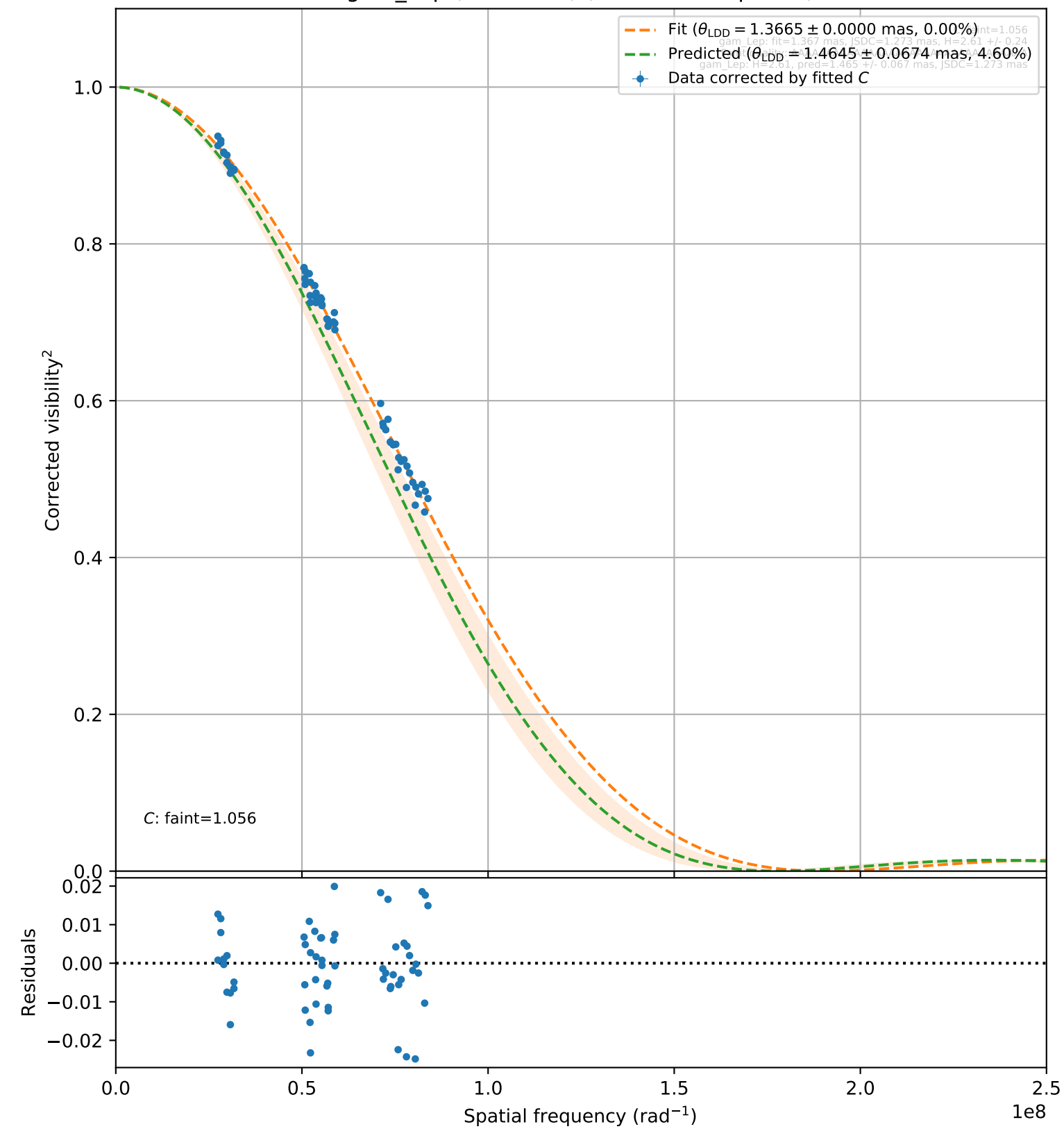
gam_Lep (faint, 104) (60 valid vis 2 points)
