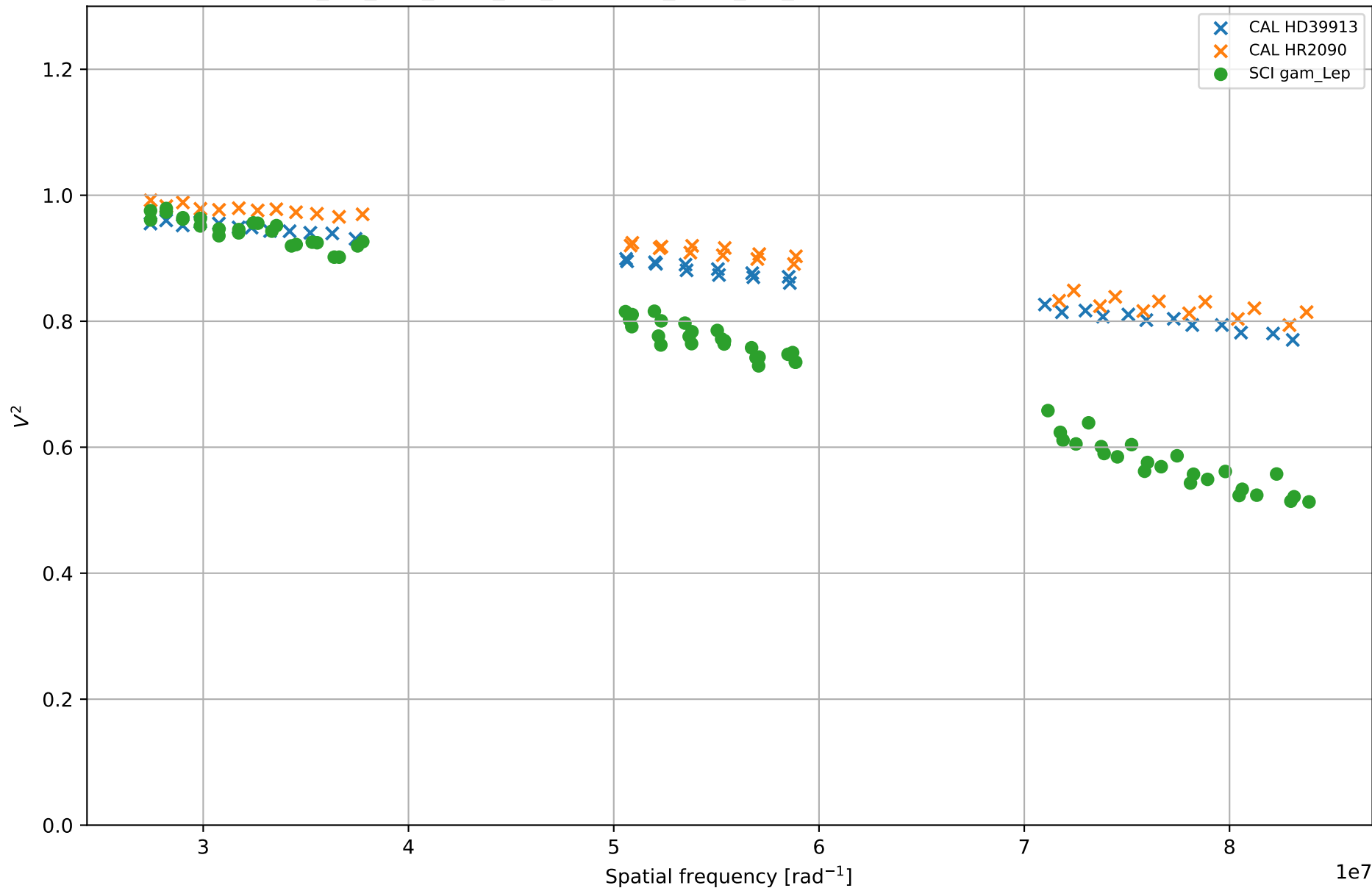
gam_Lep - calibrated experiment data GAMLEP_NO_CAL_P104_NO_HD38579_P106_NO_HD38295 - 2020-01-03 - bootstrap 00
