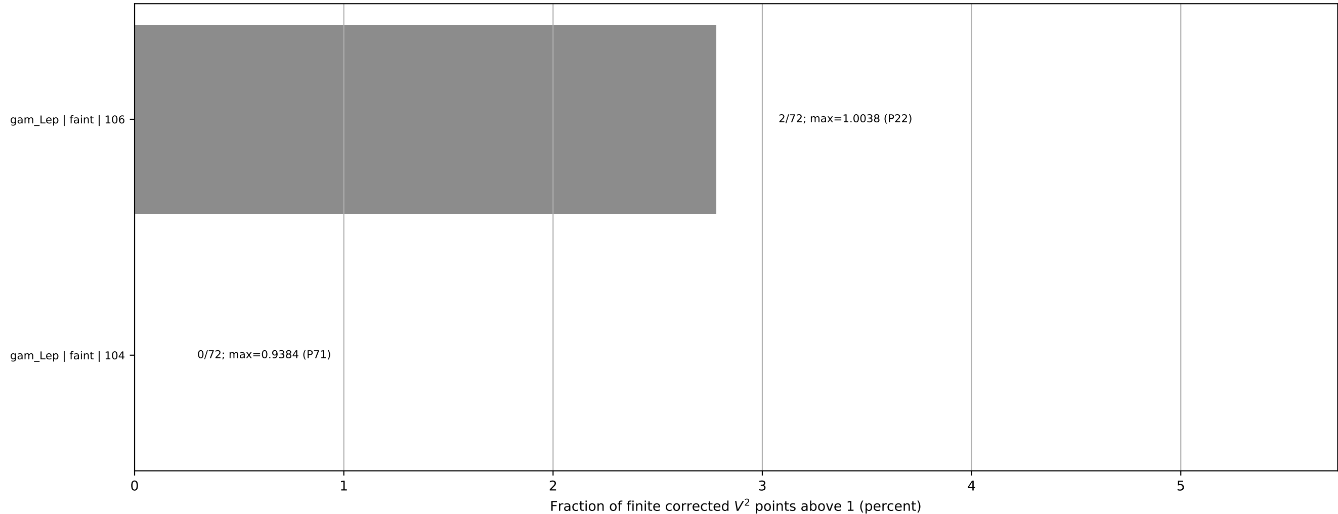
Corrected V2 > 1 overview Labels show N(V2 > 1)/N(total), maximum V2 and maximum point
