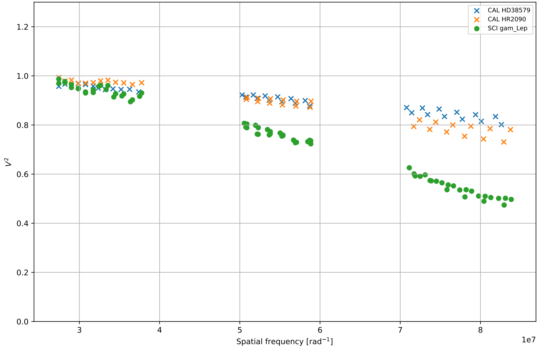
gam_Lep - calibrated experiment data GAMLEP_NO_CAL_P104_NO_HD39913_P106_NO_HD42747 - 2020-01-03 - bootstrap 00
