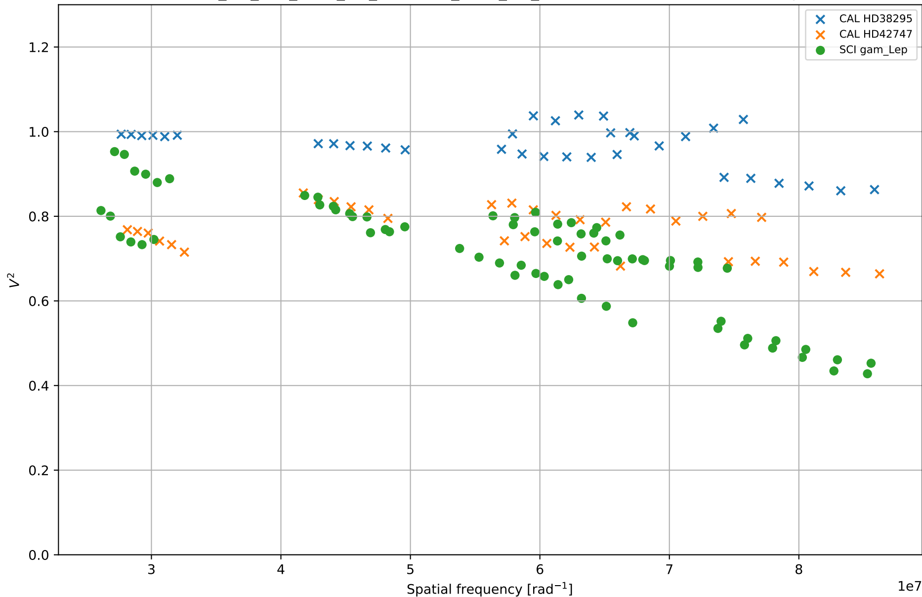
gam_Lep - calibrated experiment data GAMLEP_NO_CAL_P104_NO_HD39913_P106_NO_HR2090 - 2021-02-18 - bootstrap 00
