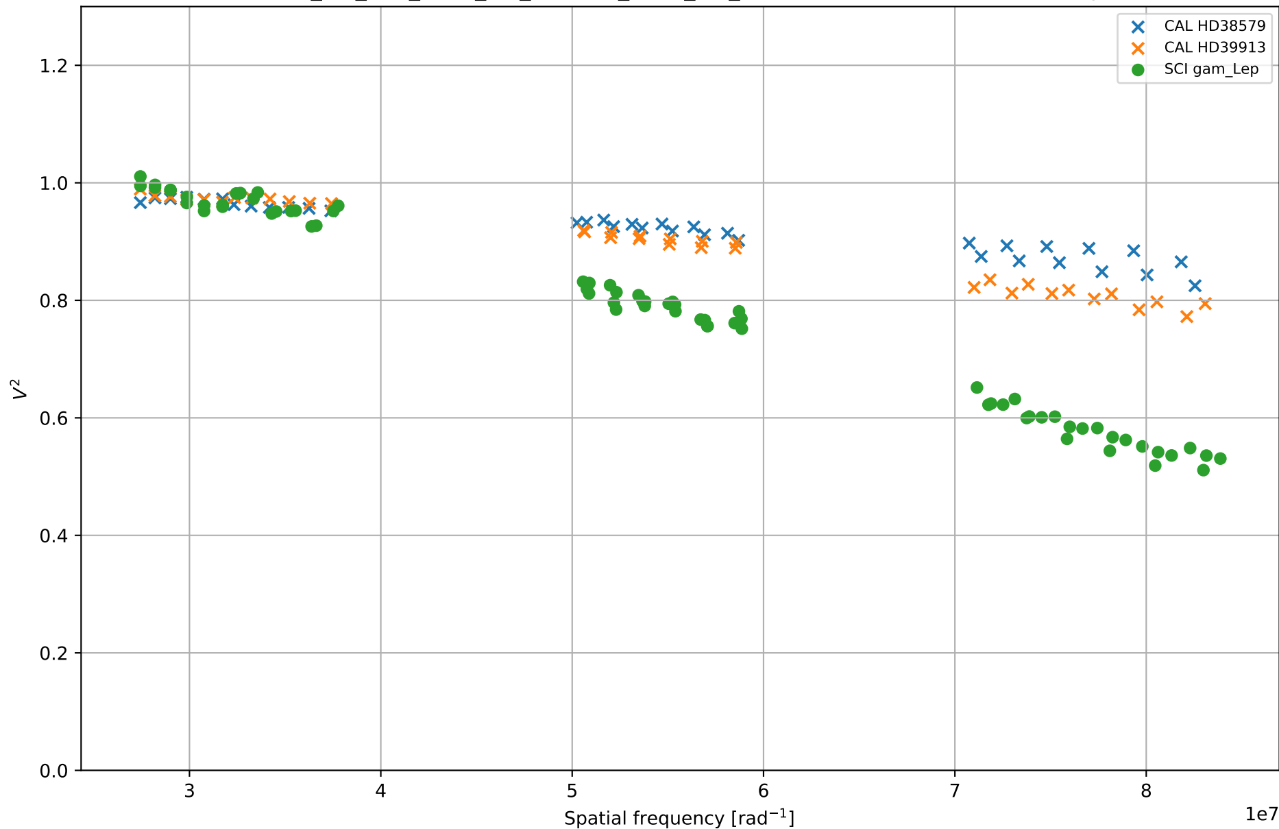
gam_Lep - calibrated experiment data GAMLEP_NO_CAL_P104_NO_HR2090_P106_NO_HR2090 - 2020-01-03 - bootstrap 00
