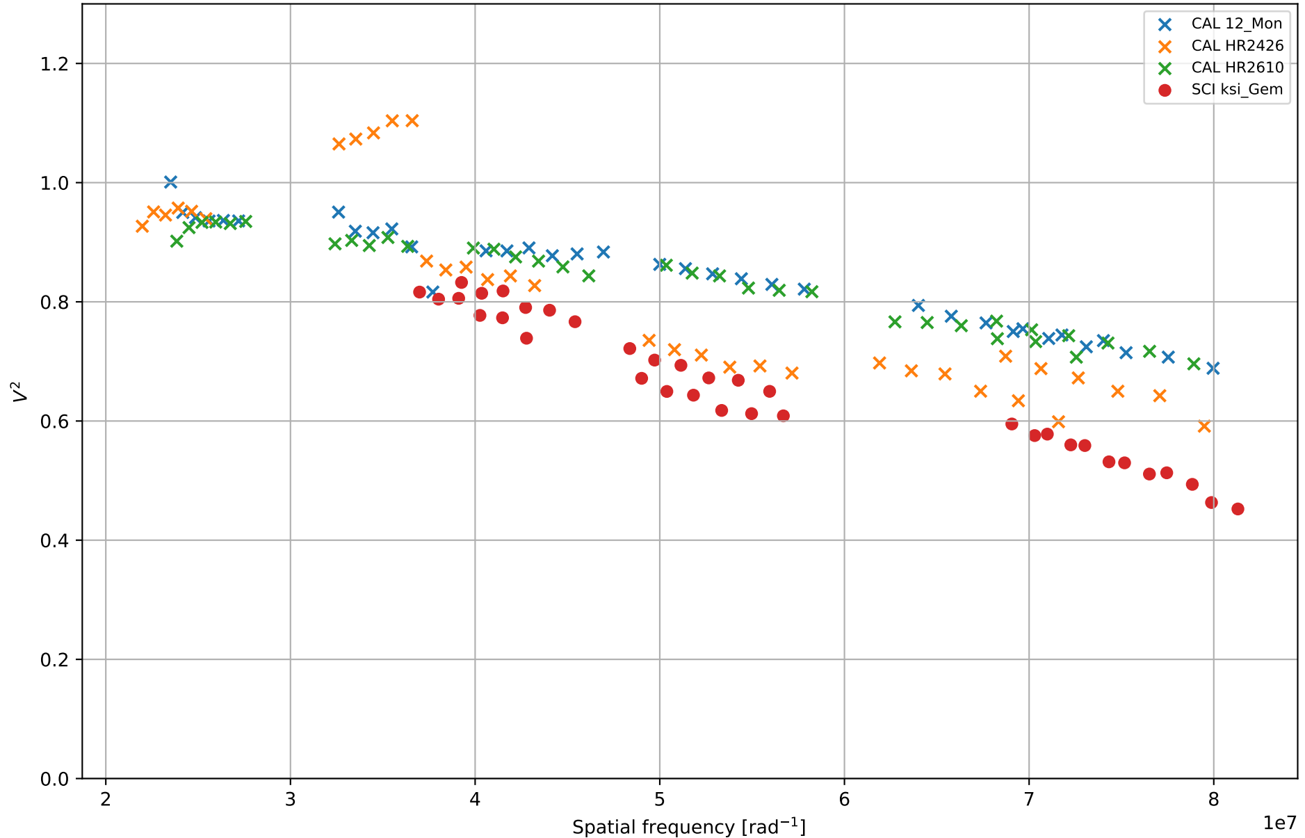
ksi_Gem - calibrated experiment data KSI GEM_NO_BL - 2022-02-26 - bootstrap 00
