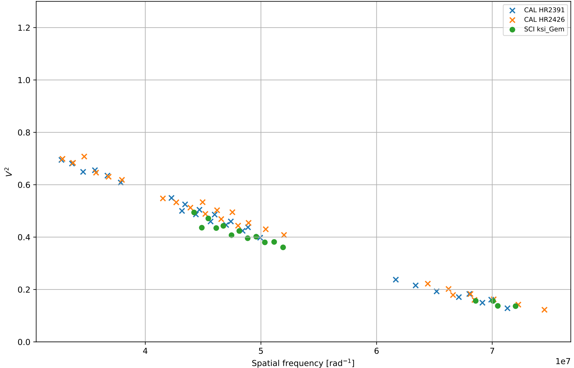
ksi_Gem - calibrated experiment data KSIGEM_NO_BL_NO_CAL_BRIGHT_NO_12MON_FAINT_NO_HR2342 - 2022-03-01 - bootstrap 00
