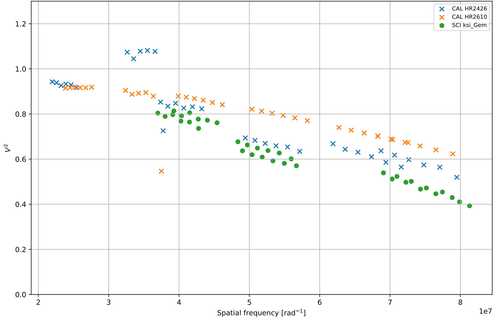
ksi_Gem - calibrated experiment data KSI GEM_NO_BL_NO_CAL_BRIGHT_NO_12MON_FAINT_NO_HR2391 - 2022-02-26 - bootstrap 00
