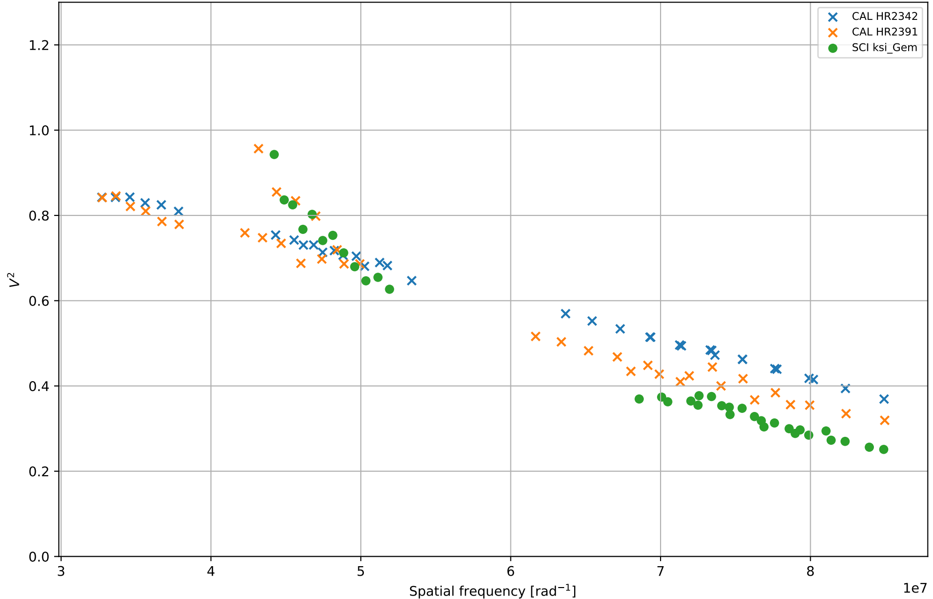
ksi_Gem - calibrated experiment data KSI GEM_NO_BL_NO_CAL_BRIGHT_NO_12MON_FAINT_NO_HR2426 - 2022-03-01 - bootstrap 00
