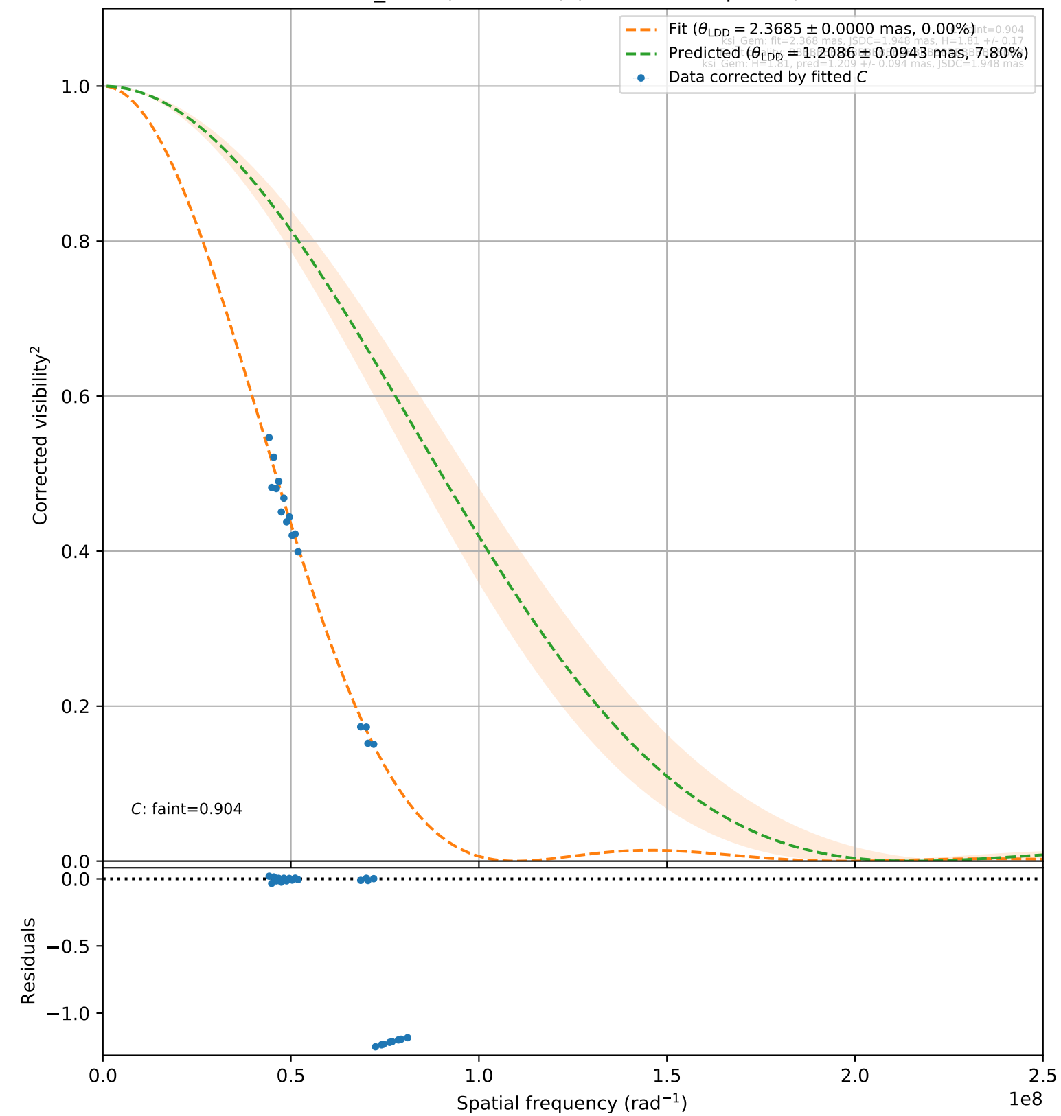
ksi_Gem (faint, 106) (24 valid vis 2 points)
