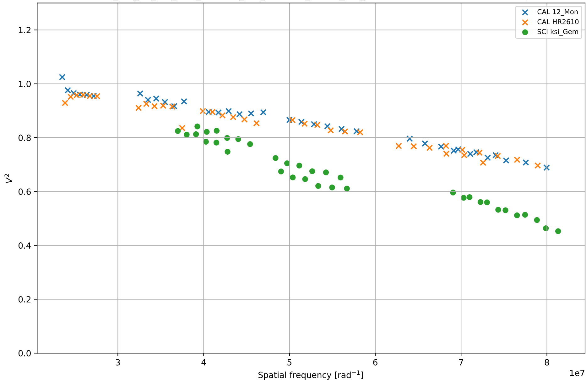
ksi_Gem - calibrated experiment data KSIGEM_NO_BL_NO_CAL_BRIGHT_NO_HR2426_FAINT_NO_HR2342 - 2022-02-26 - bootstrap 00
