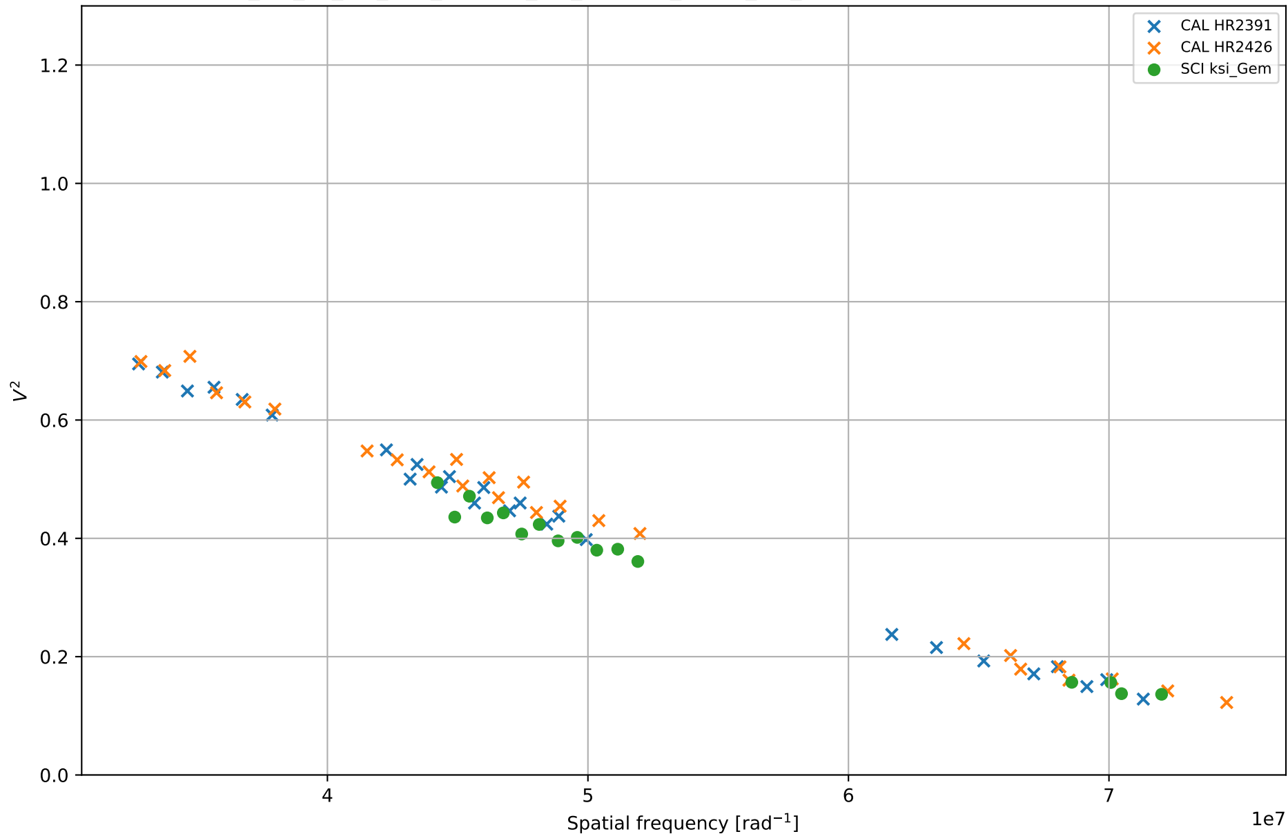
ksi_Gem - calibrated experiment data KSGEM_NO_BL_NO_CAL_BRIGHT_NO_HR2426_FAINT_NO_HR2342 - 2022-03-01 - bootstrap 00
