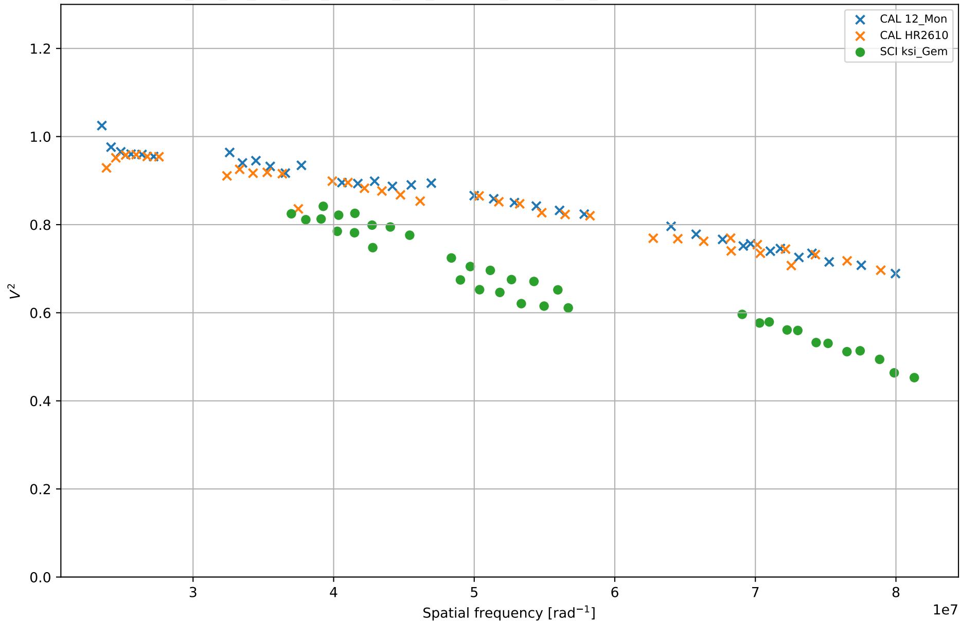
ksi_Gem - calibrated experiment data KSIGEM_NO_BL_NO_CAL_BRIGHT_NO_HR2426_FAINT_NO_HR2391 - 2022-02-26 - bootstrap 00
