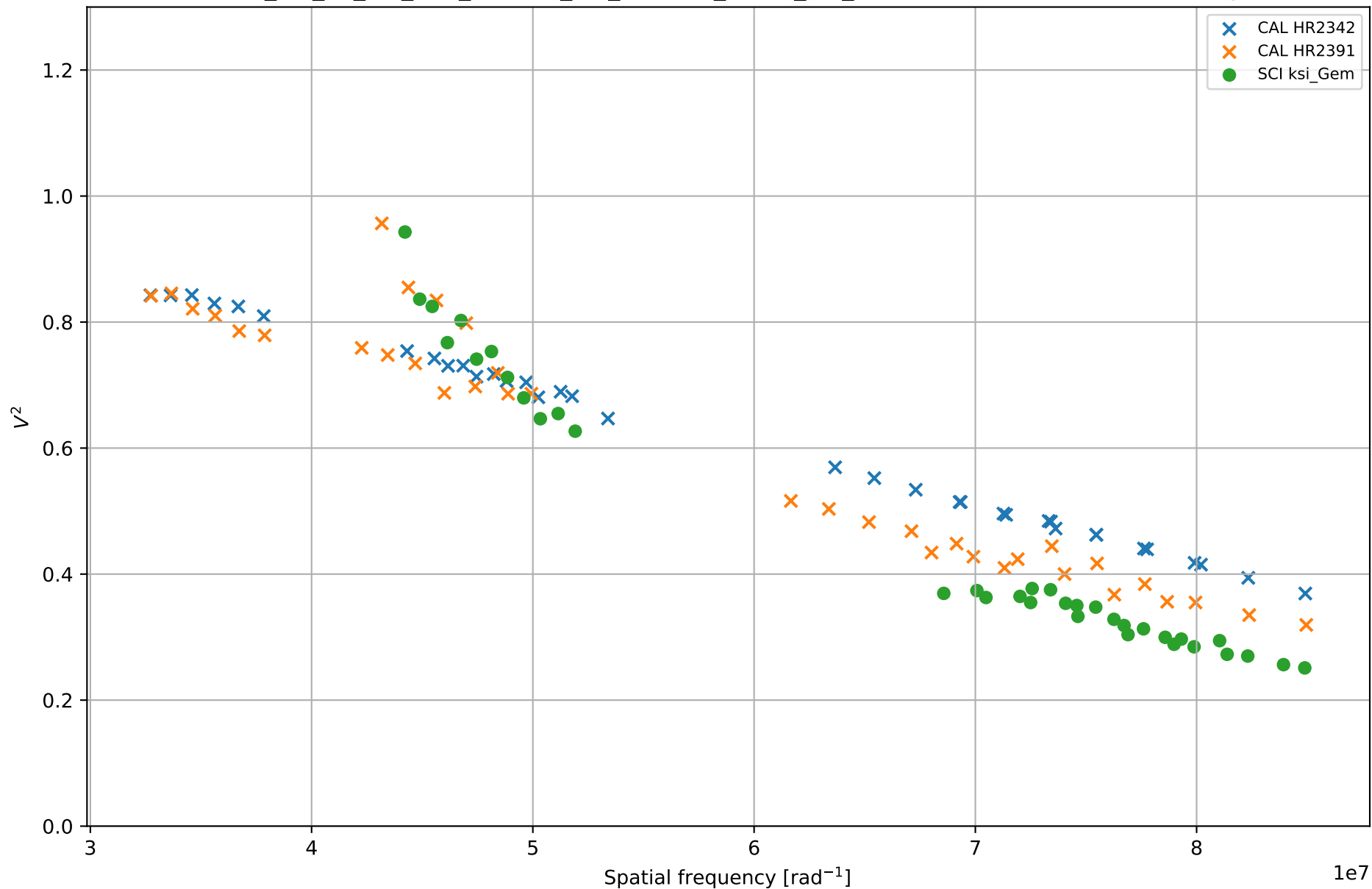
ksi_Gem - calibrated experiment data KSIGEM_NO_BL_NO_CAL_BRIGHT_NO_HR2426_FAINT_NO_HR2426 - 2022-03-01 - bootstrap 00
