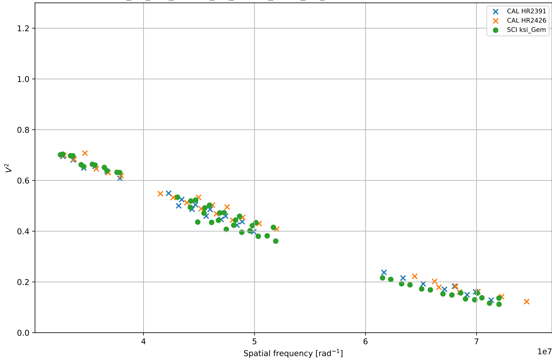
ksi_Gem - calibrated experiment data KSIGEM_NO_CAL_BRIGHT_NO_12MON_FAINT_NO_HR2342 - 2022-03-01 - bootstrap 00
