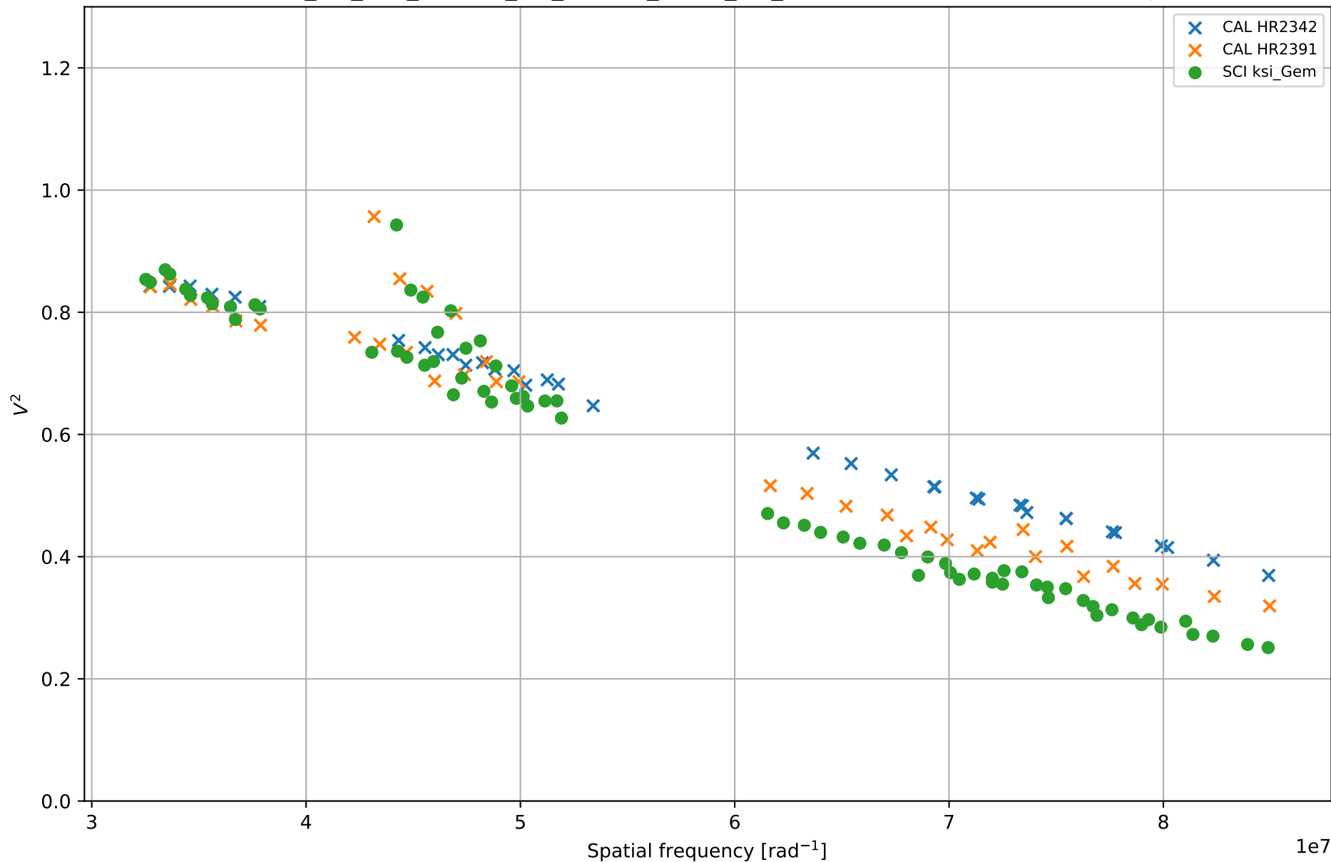
ksi_Gem - calibrated experiment data KSI GEM_NO_CAL_BRIGHT_NO_12MON_FAINT_NO_HR2426 - 2022-03-01 - bootstrap 00
