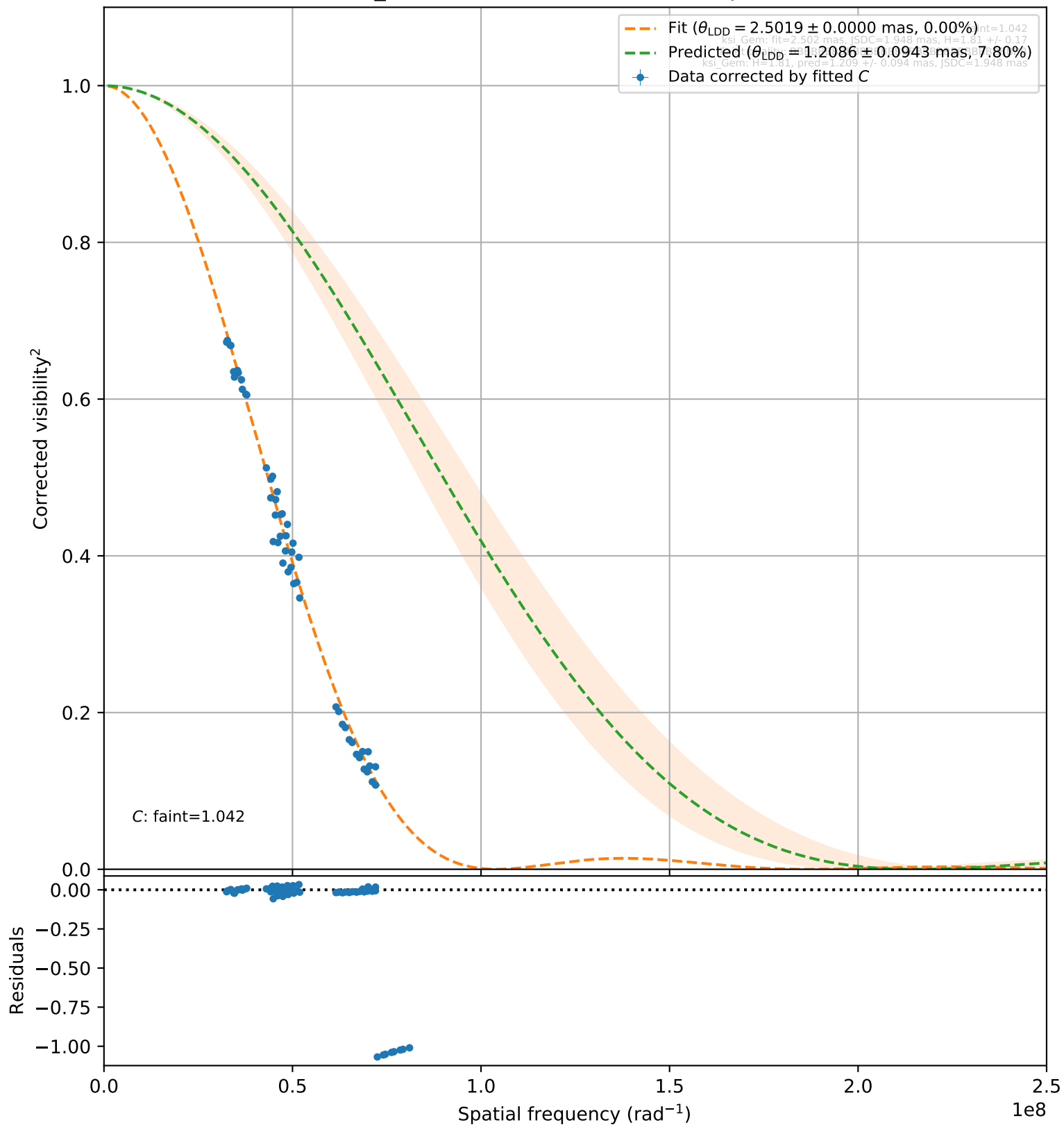
ksi_Gem (faint, 106) (60 valid vis 2 points)
