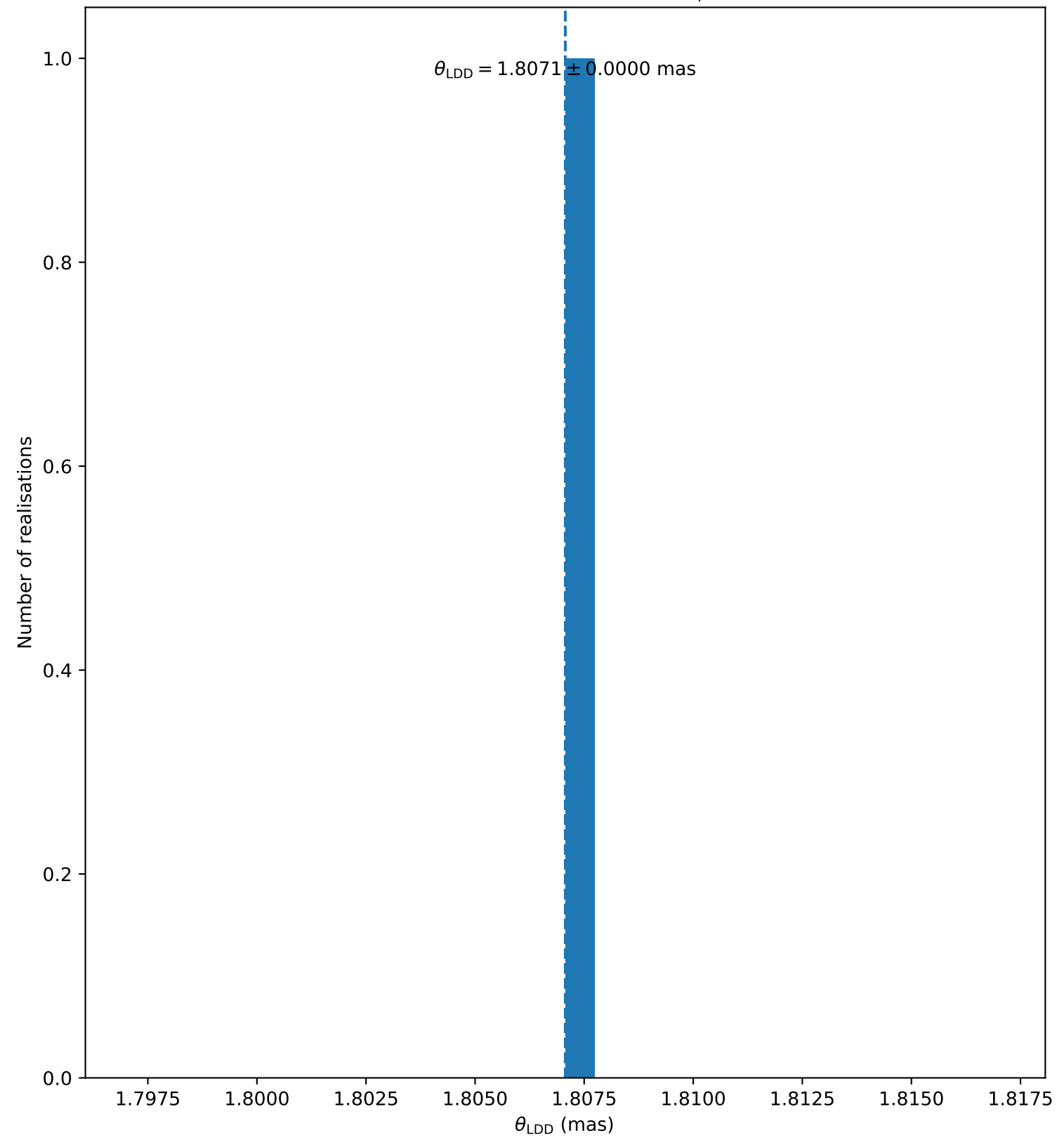
ksi_Gem (faint, 106) ( N_{\text{bootstrap}} = 1 )
