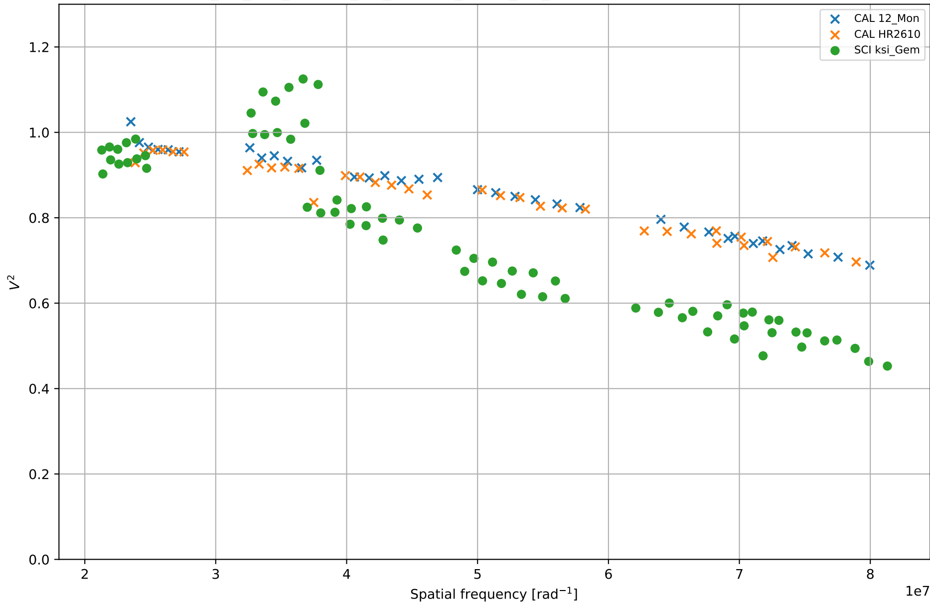
ksi_Gem - calibrated experiment data KSGEM_NO_CAL_BRIGHT_NO_HR2426_FAINT_NO_HR2426 - 2022-02-26 - bootstrap 00
