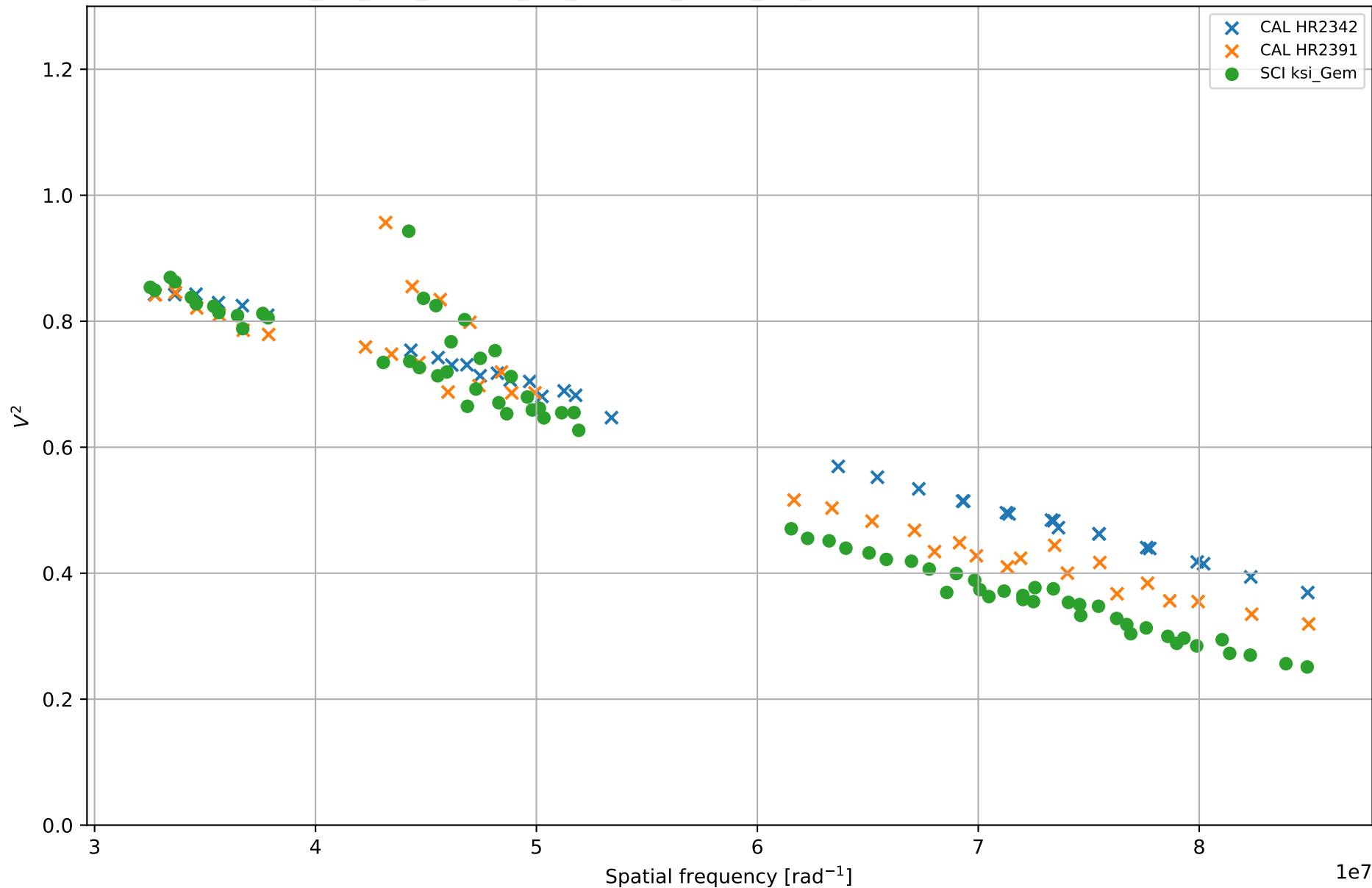
ksi_Gem - calibrated experiment data KSGEM_NO_CAL_BRIGHT_NO_HR2426_FAINT_NO_HR2426 - 2022-03-01 - bootstrap 00
