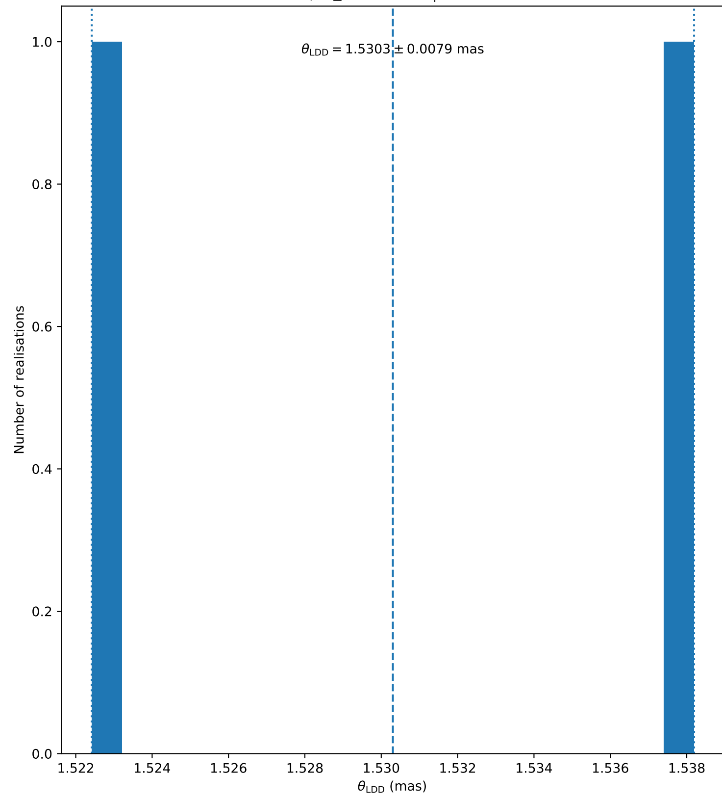
pi3_Ori ( N_{\text{bootstrap}} = 2 )
