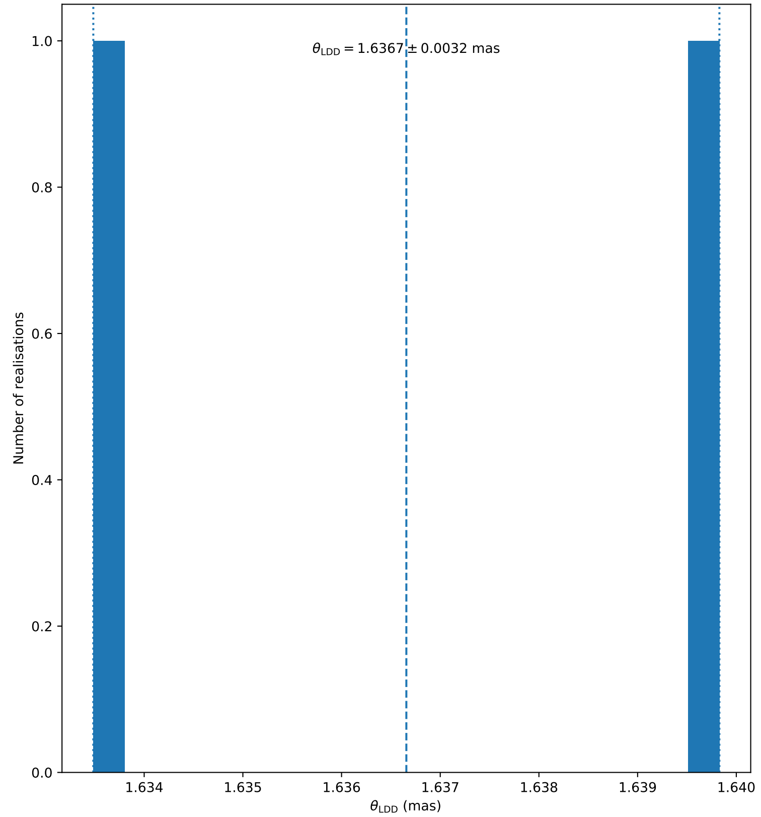
rho_Pup ( N_{\text{bootstrap}} = 2 )
