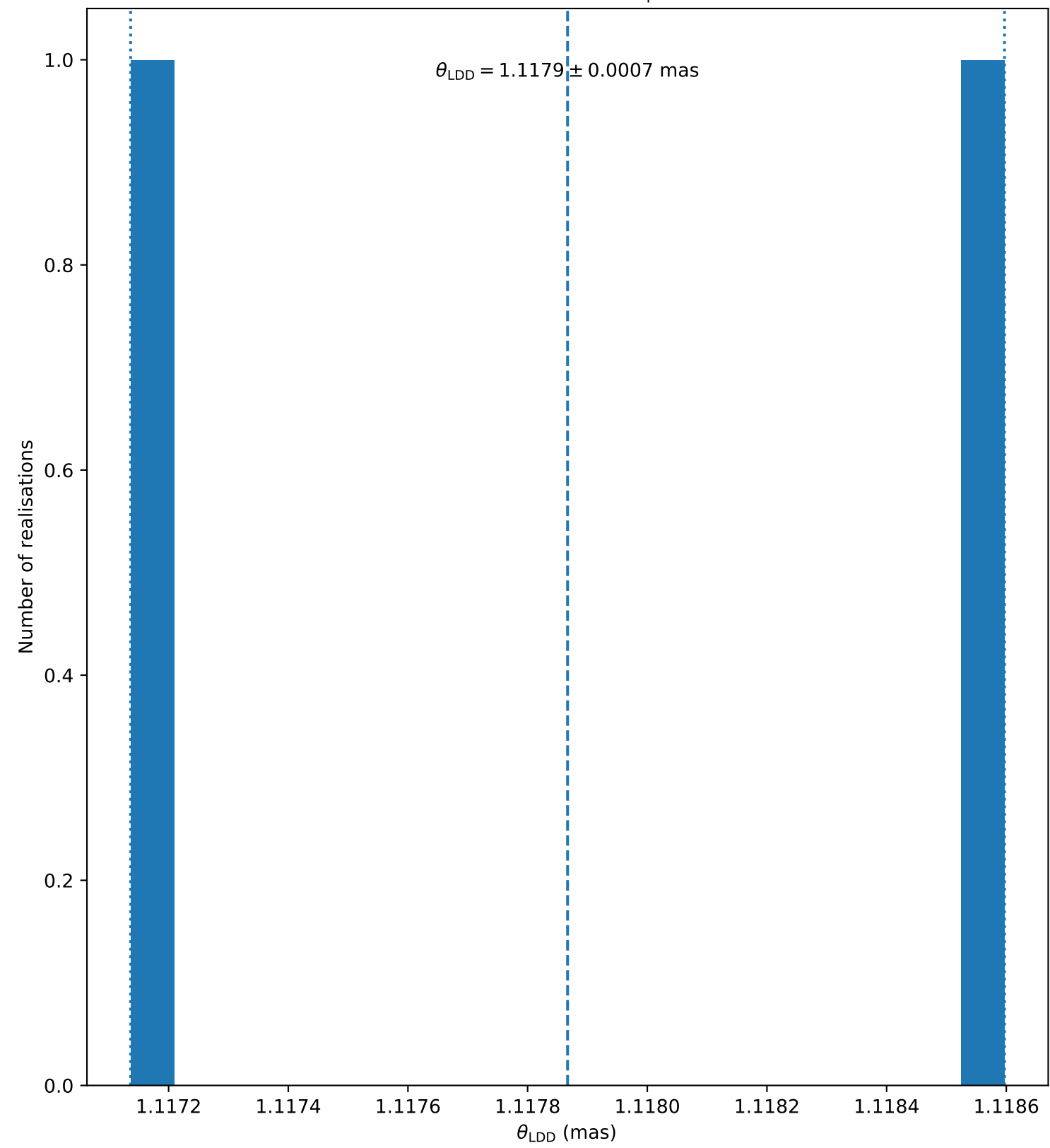
HD124850 ( N_{\text{bootstrap}} = 2 )
