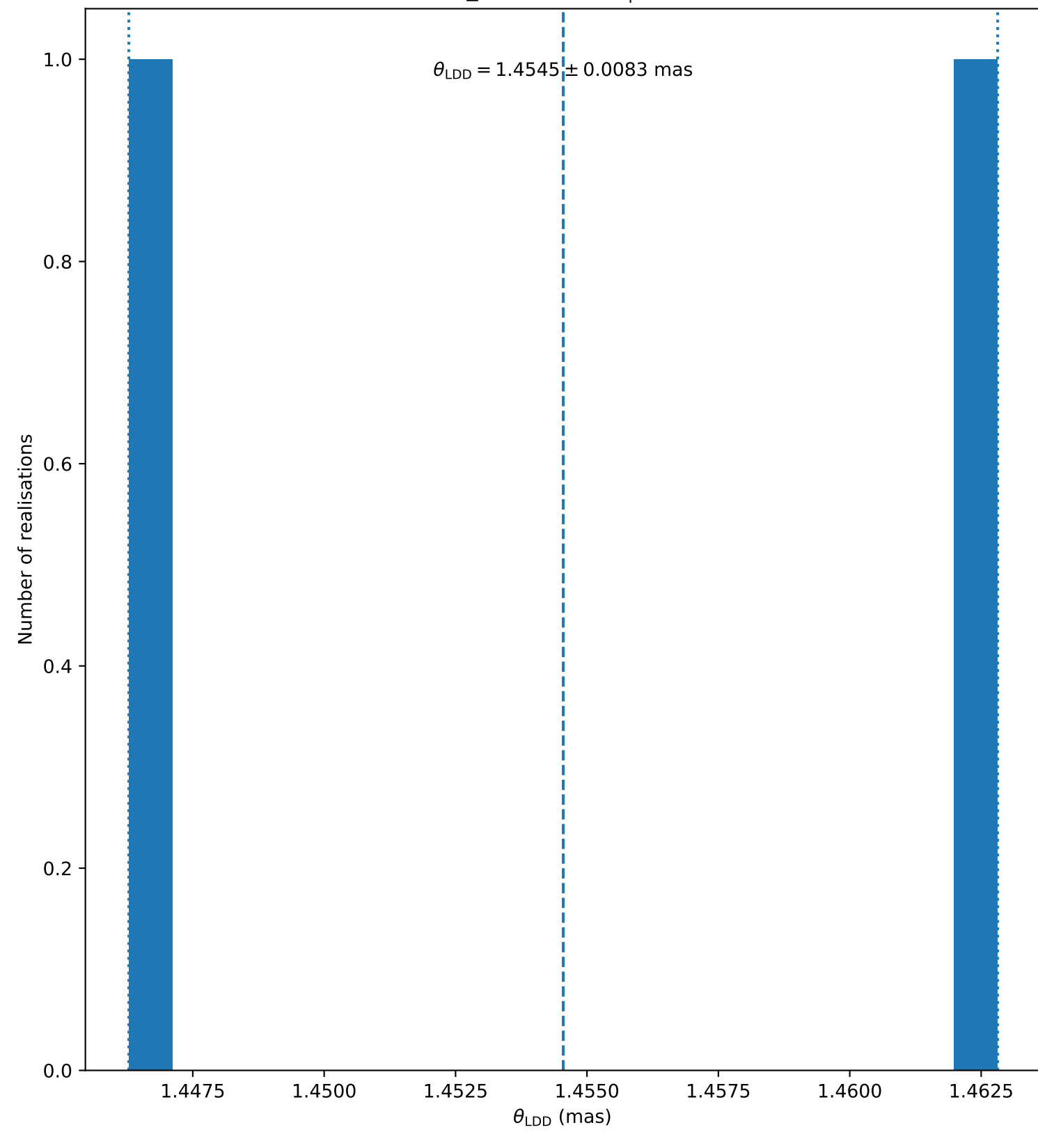
ksi_Gem ( N_{\text{bootstrap}} = 2 )
