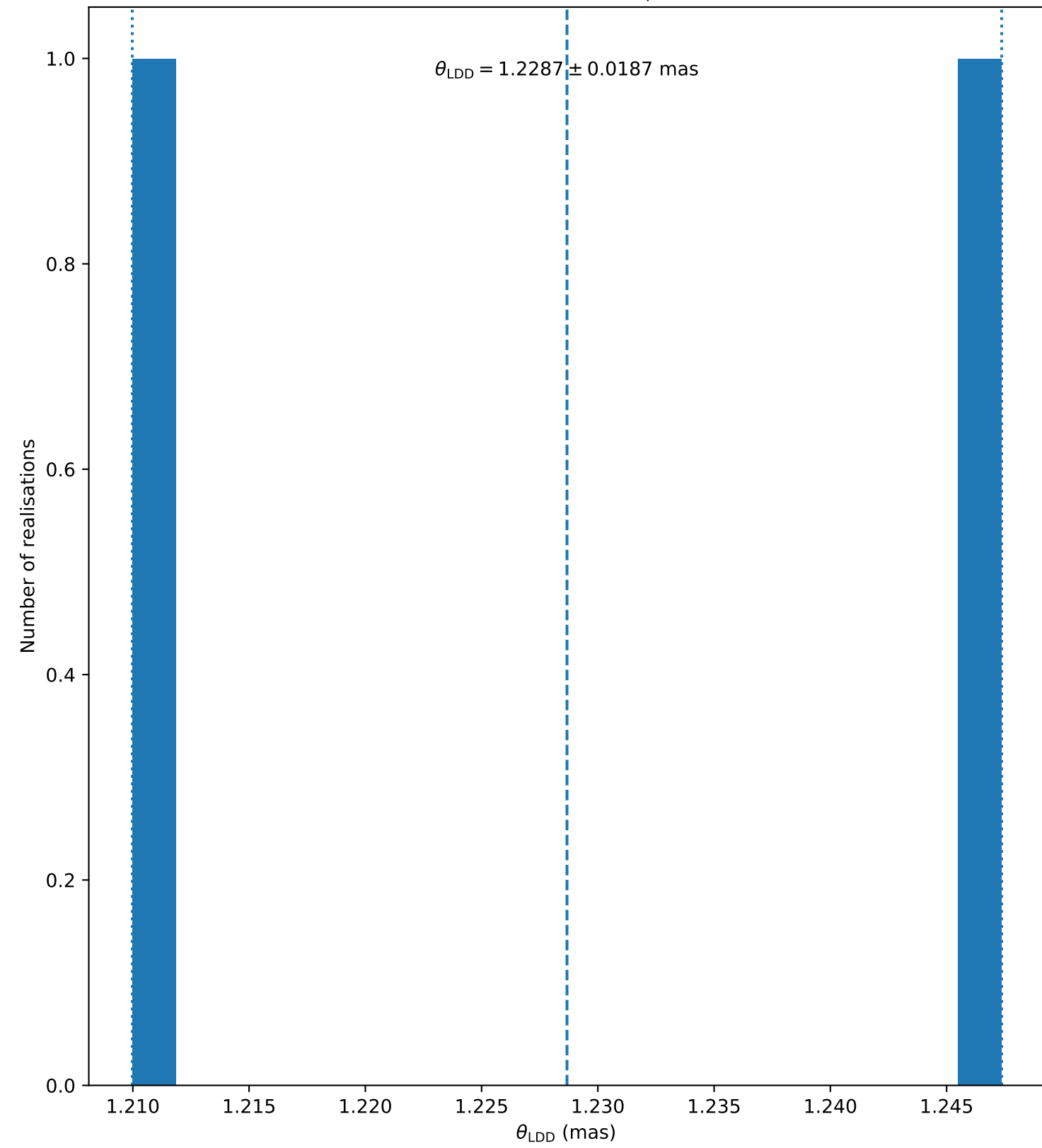
HD142860 ( N_{\text{bootstrap}} = 2 )
