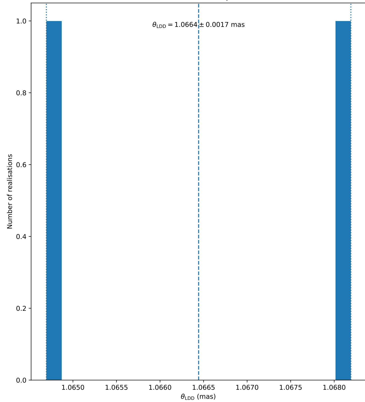
HD141004 ( N_{\text{bootstrap}} = 2 )
