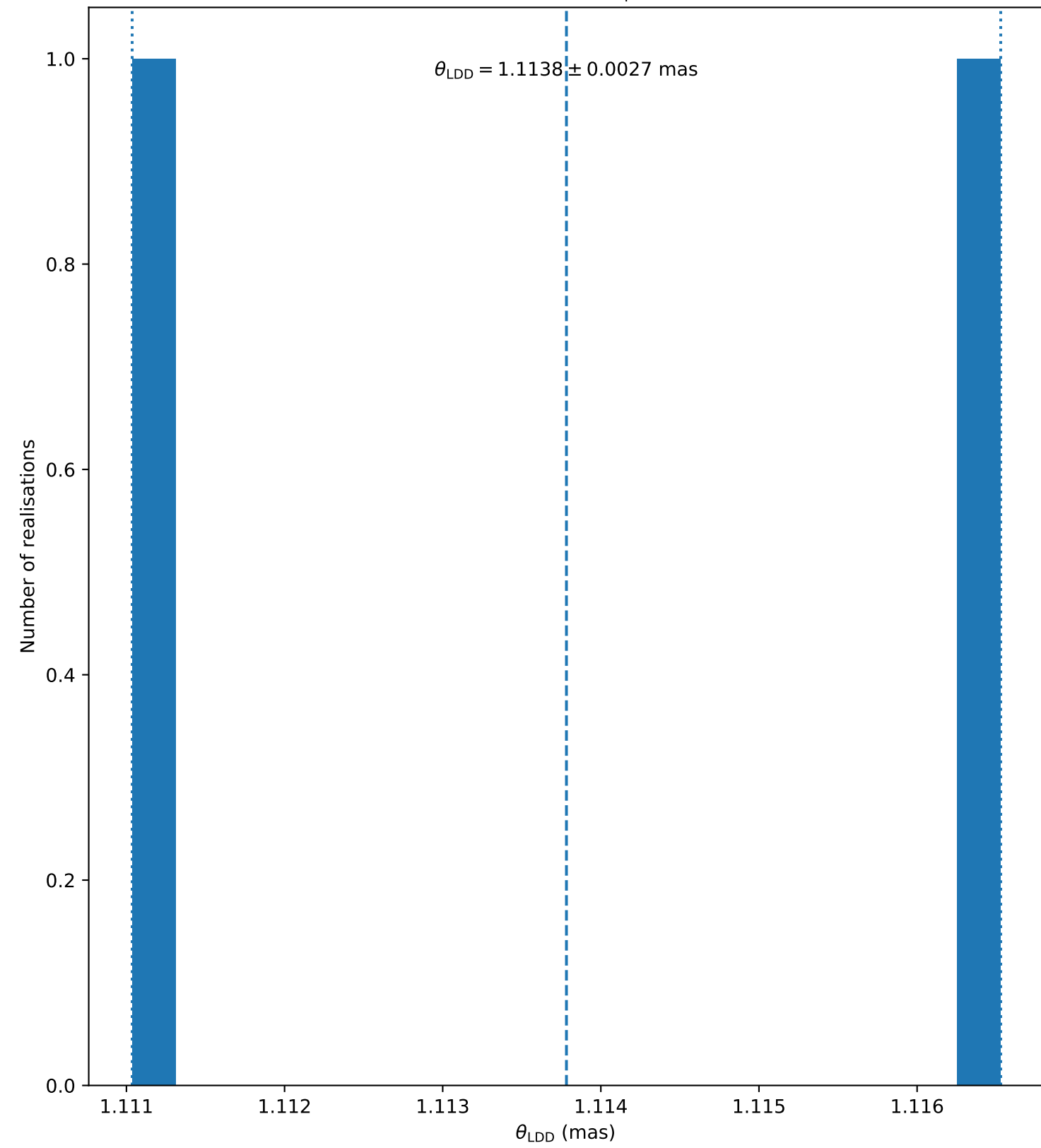
iot_Psc ( N_{\text{bootstrap}} = 2 )
