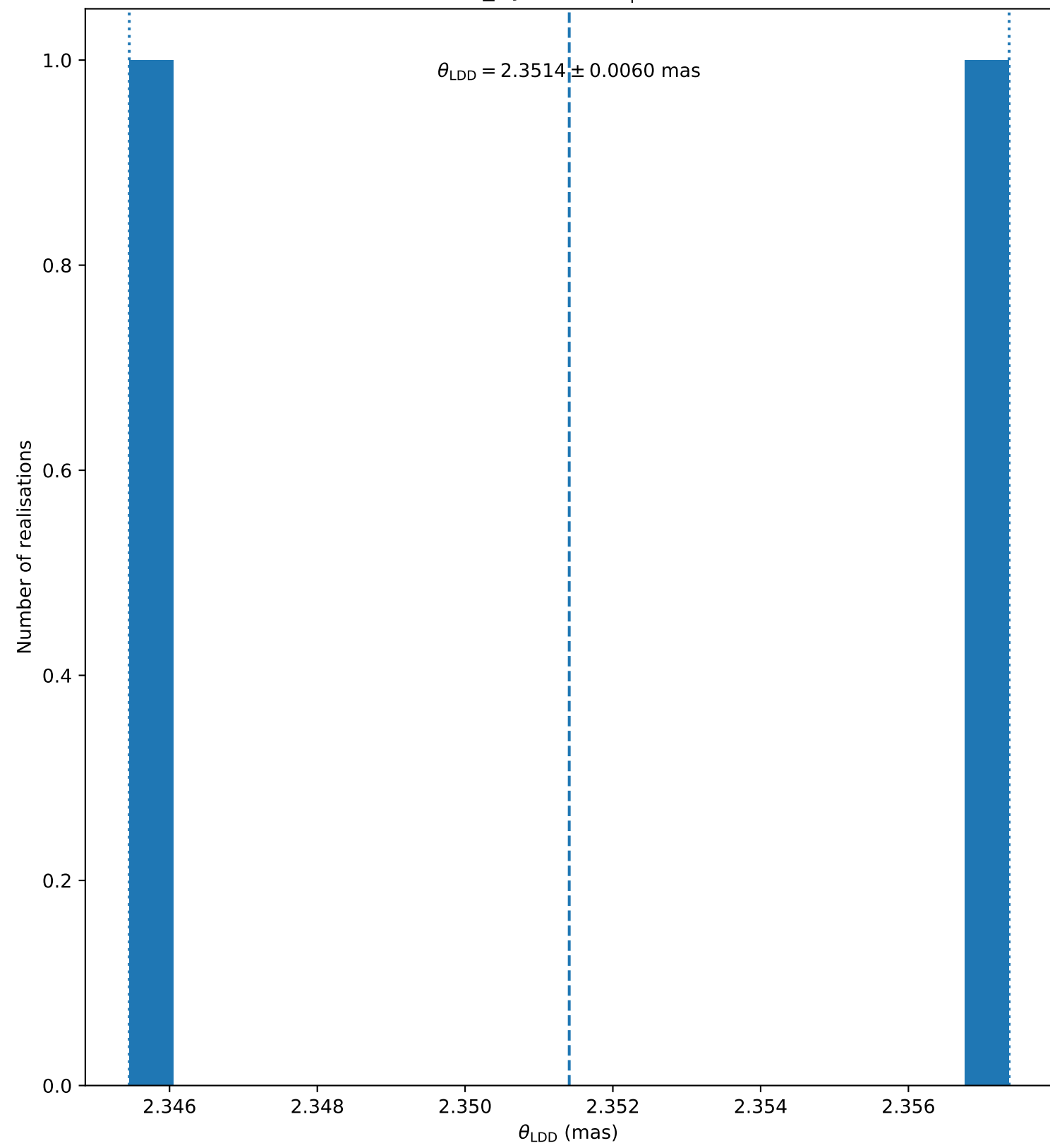
bet_Hyi ( N_{\text{bootstrap}} = 2 )
