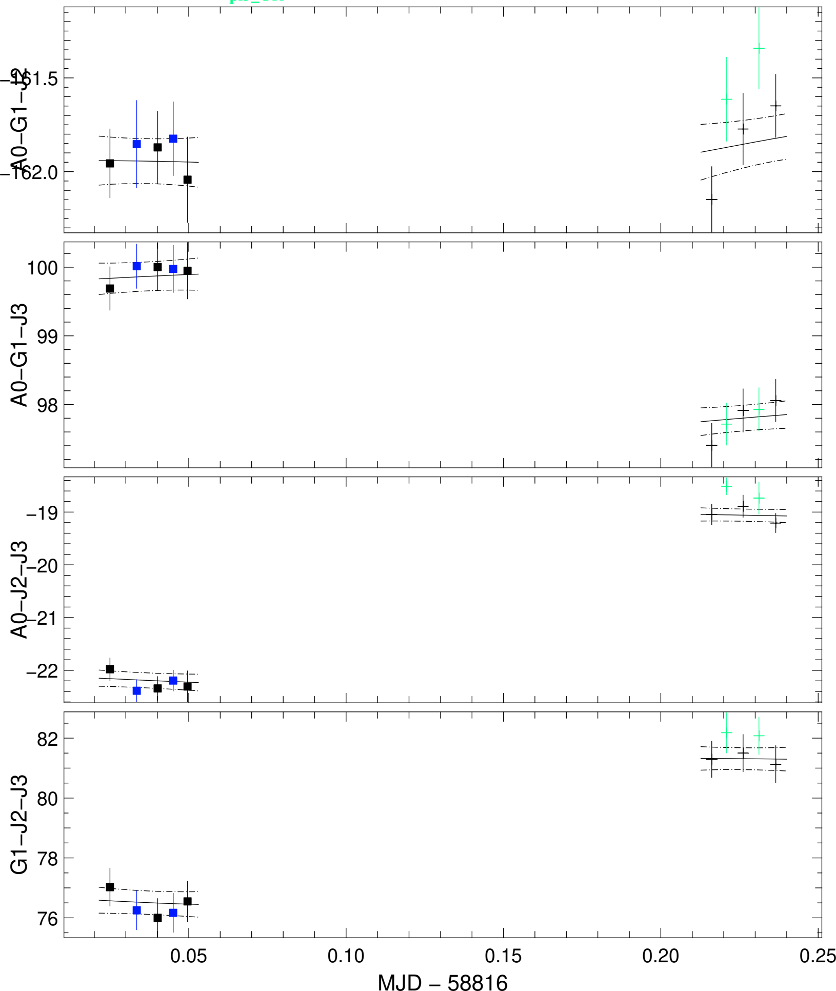
Transfer-Function t3Phi (black) and Scientific t3Phi (colors) averaged in the range [[1.637,1.715],[2.04,2.25]]\mu\text{m}
