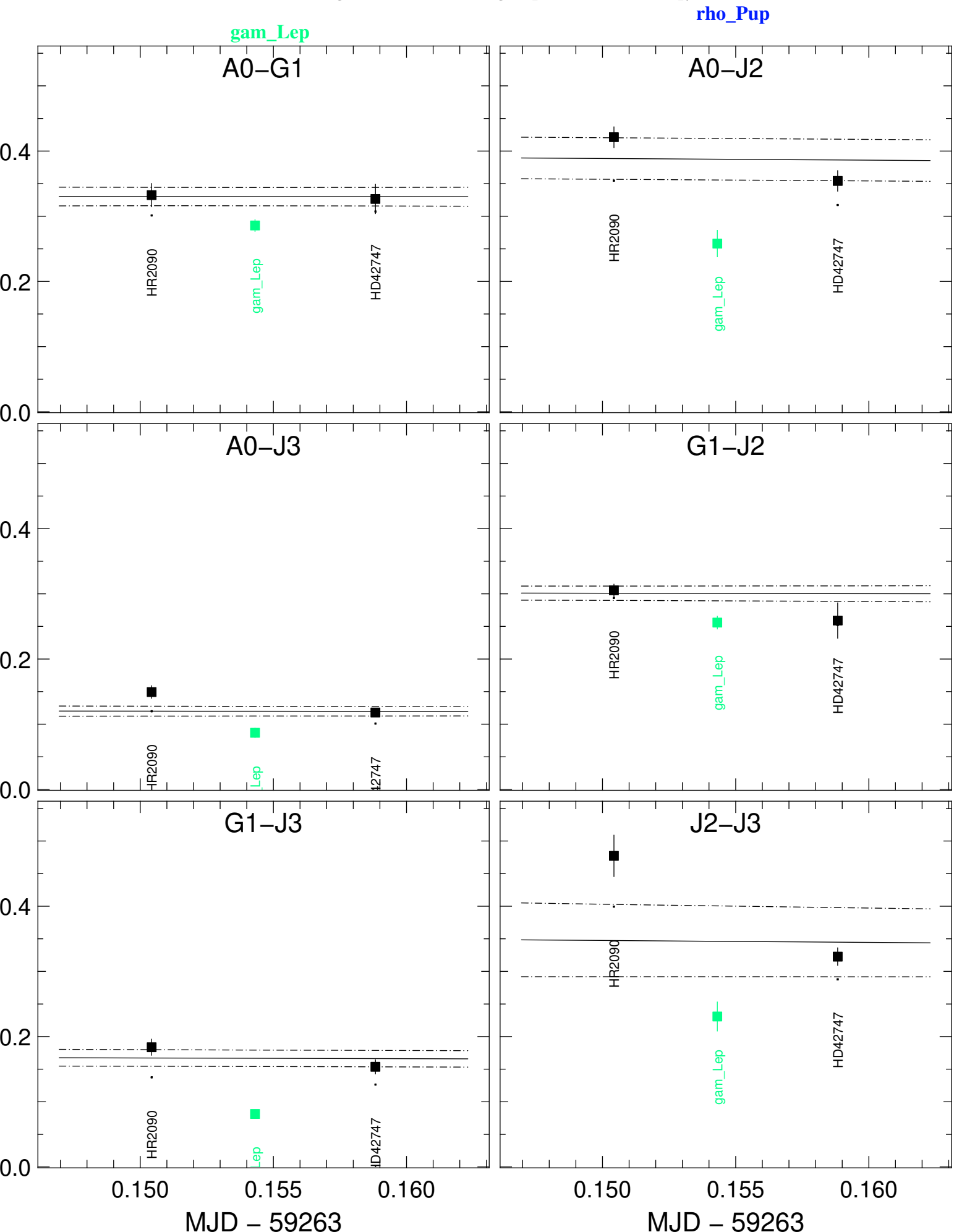
Transfer-Function vis2 (black) and Scientific vis2 (colors) averaged in the range [1.533,1.533] \mu m
