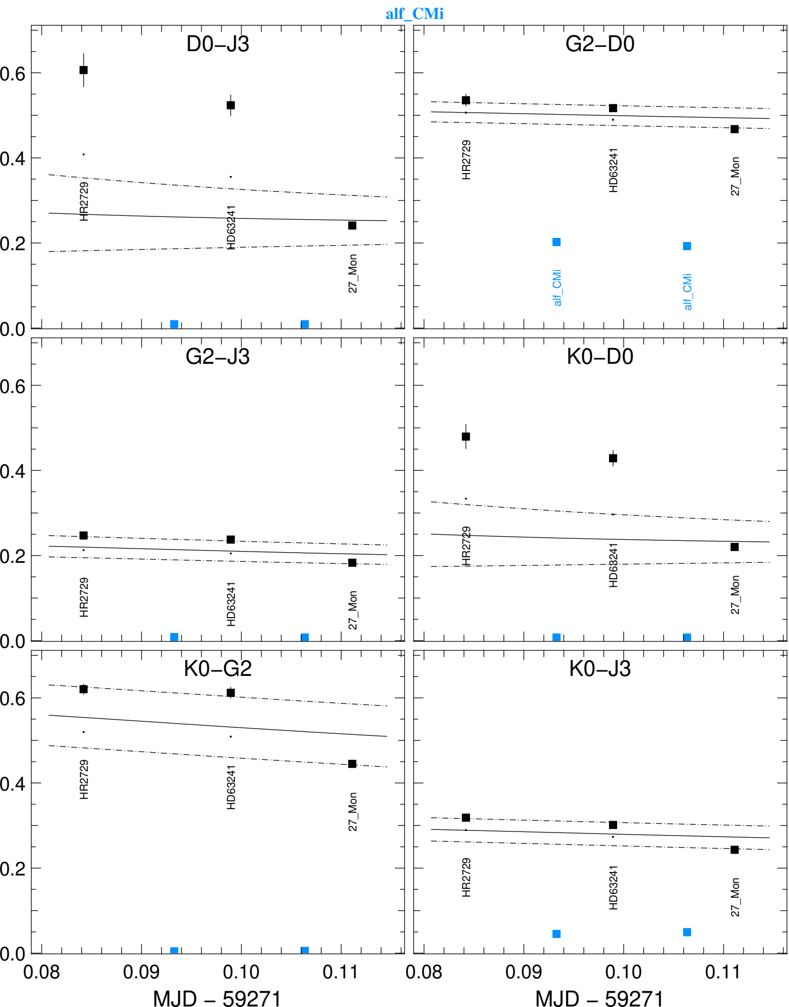
Transfer-Function vis2 (black) and Scientific vis2 (colors) averaged in the range [1.581, 1.581]\mu\text{m}
