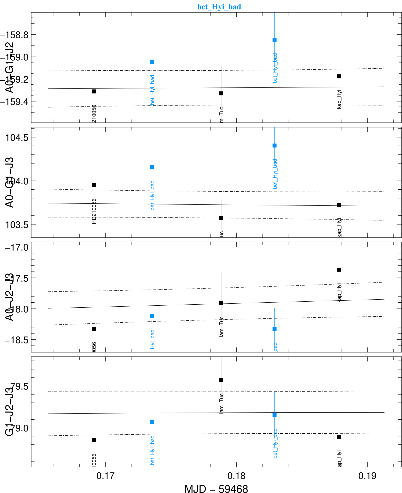
Transfer-Function t3Phi (black) and Scientific t3Phi (colors) averaged in the range [1.581,1.581] \mu m
