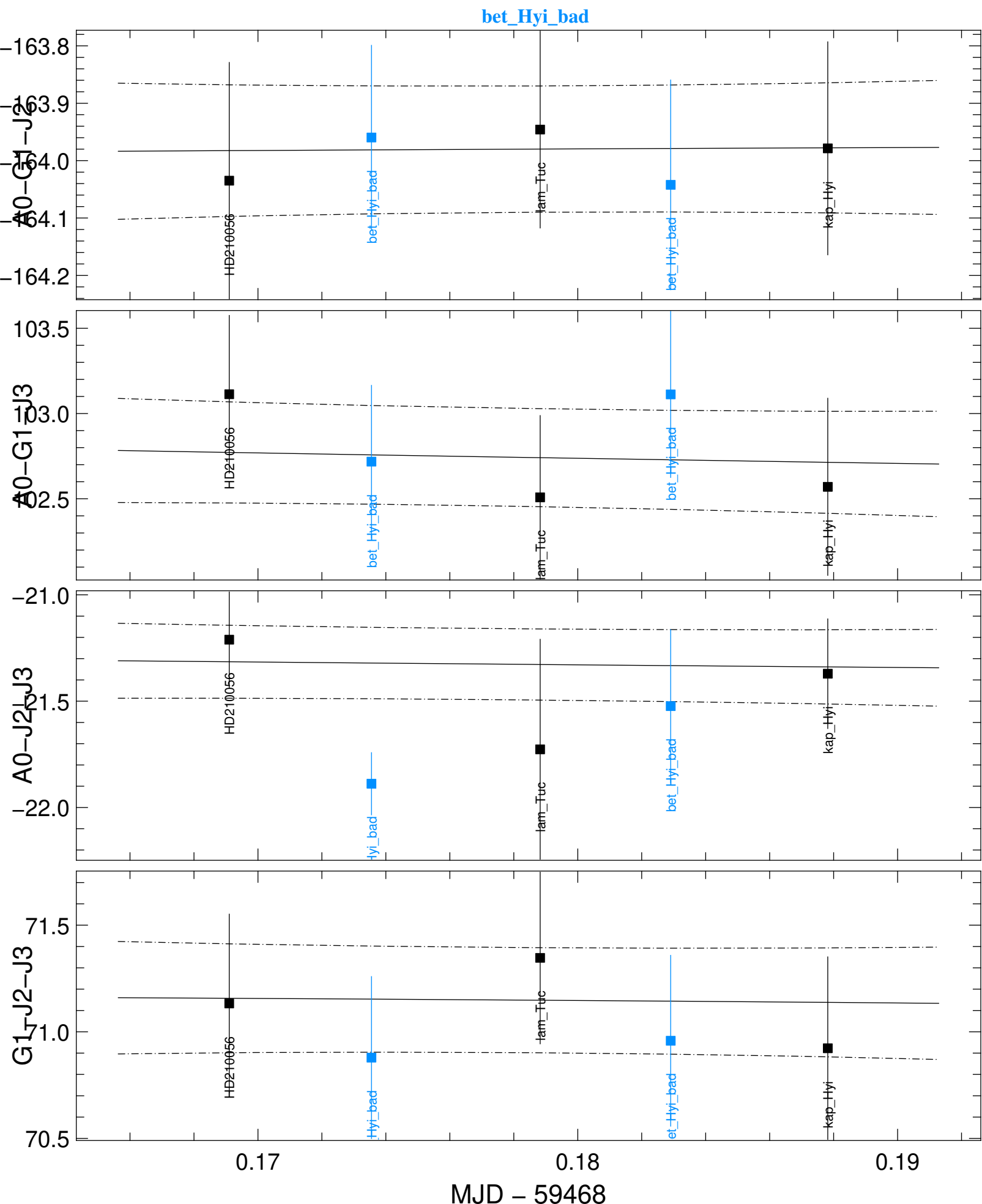
Transfer-Function t3Phi (black) and Scientific t3Phi (colors) averaged in the range [1.629,1.629] \mu\text{m}
