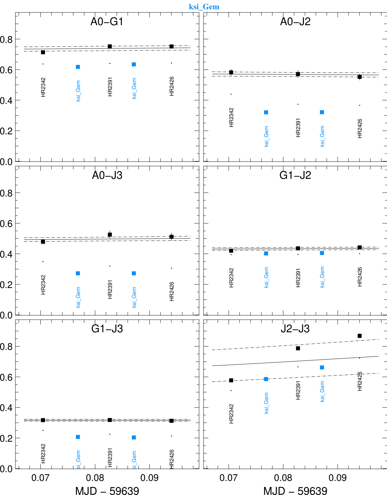
Transfer-Function vis2 (black) and Scientific vis2 (colors) averaged in the range [1.773, 1.773]\mu\text{m}
