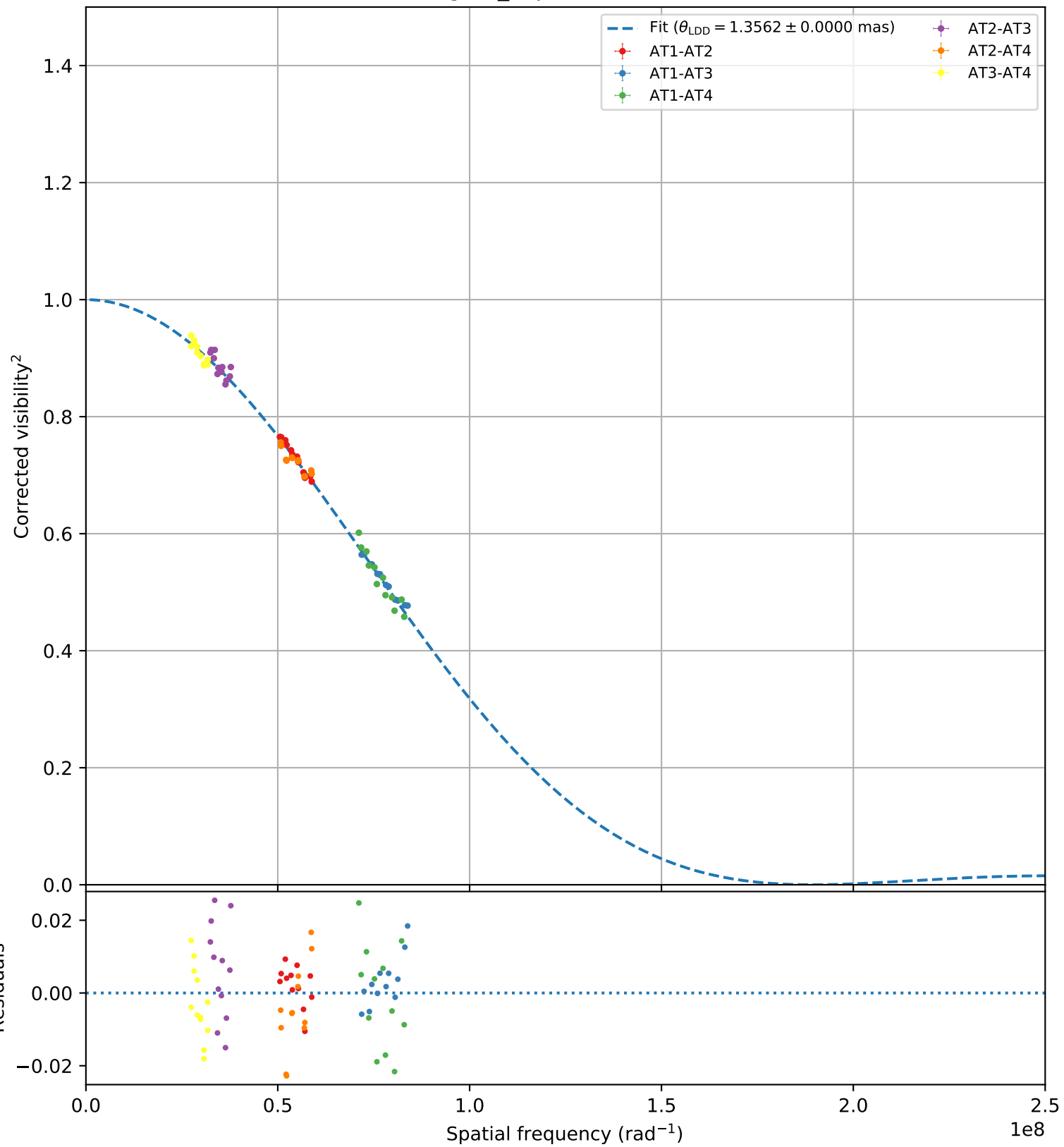
gam_Lep (faint, 104)
