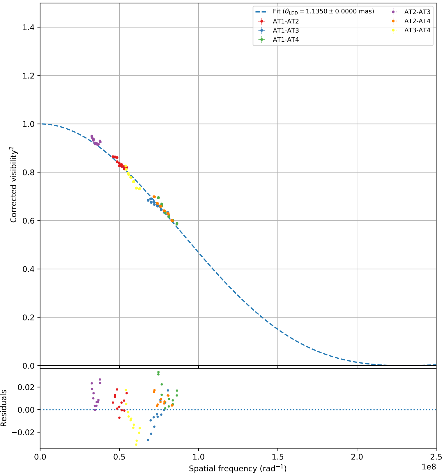
HD124850 (faint, 105)
