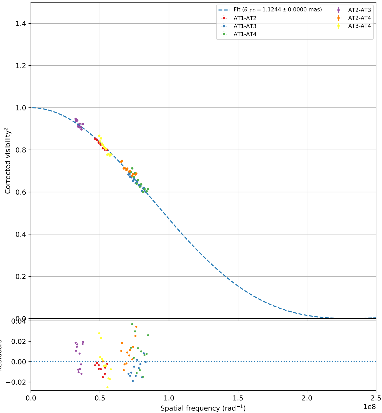
iot_Psc (bright, 104)
