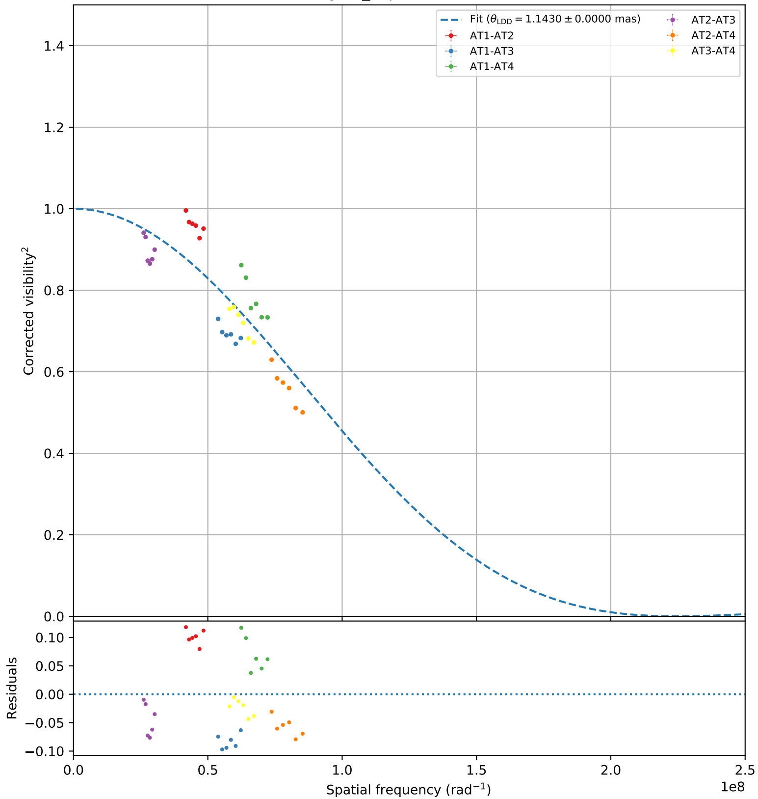
gam_Lep (faint, 106)
