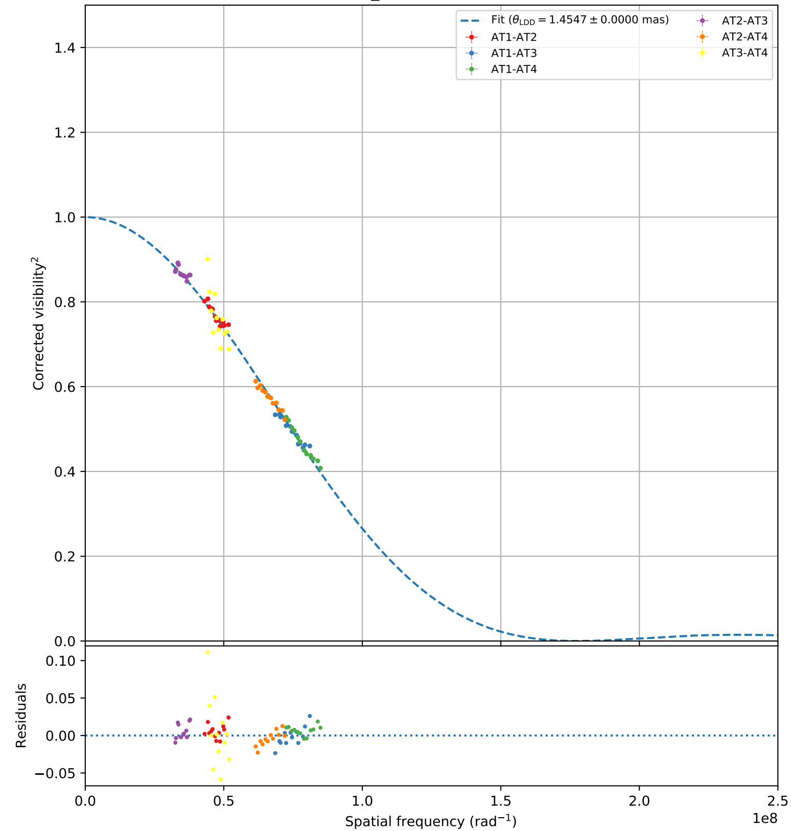
ksi_Gem (faint, 106)
