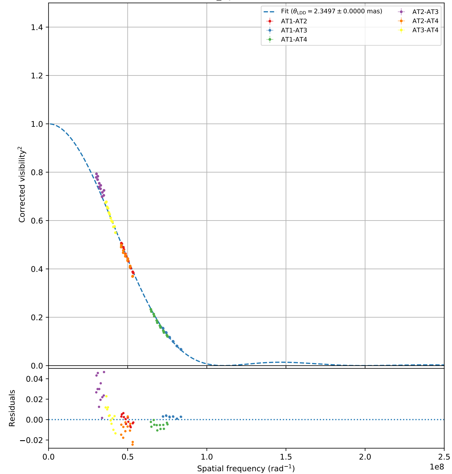
bet_Hyi (faint, 106)
