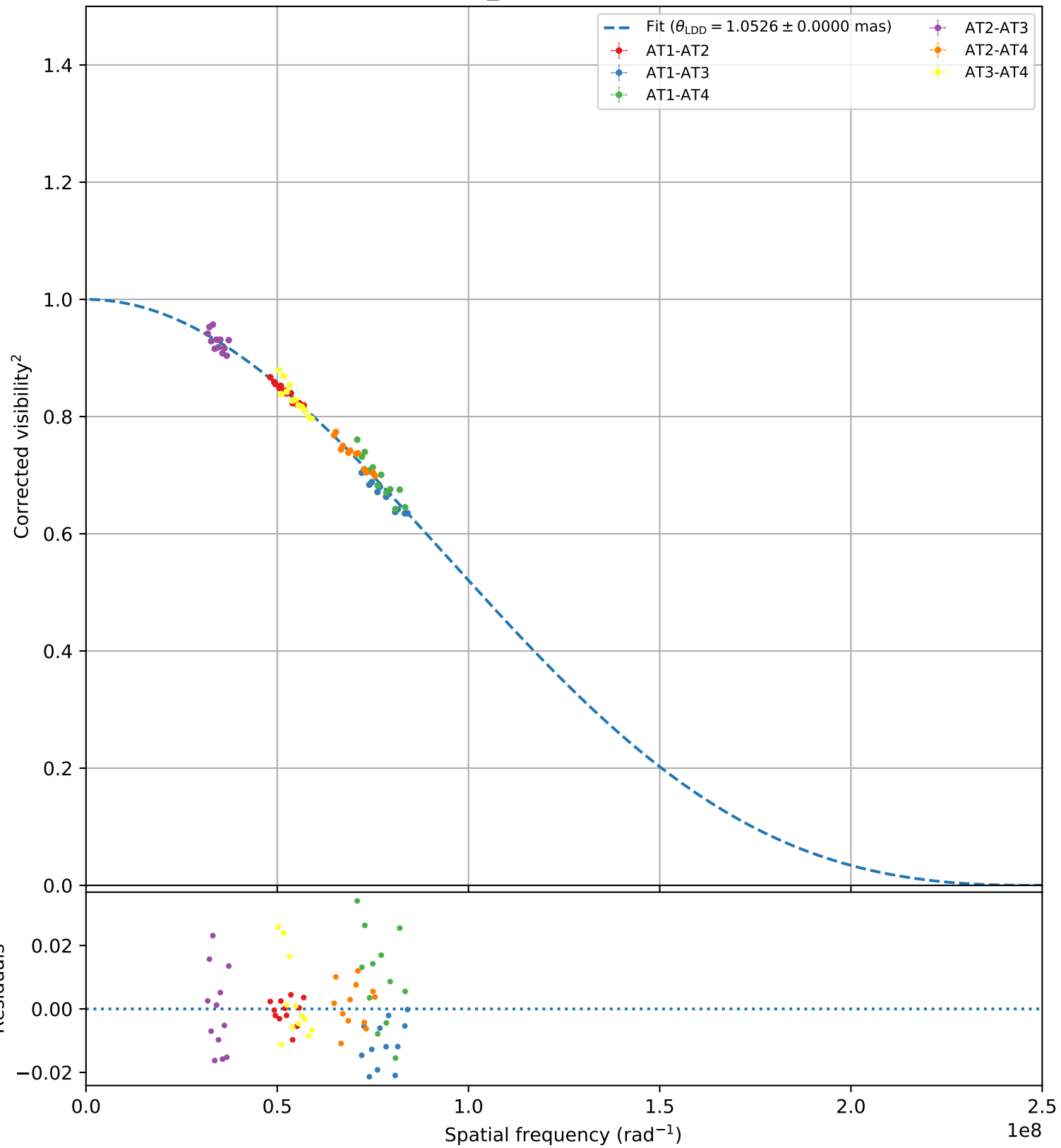
iot_Psc (faint, 104)
