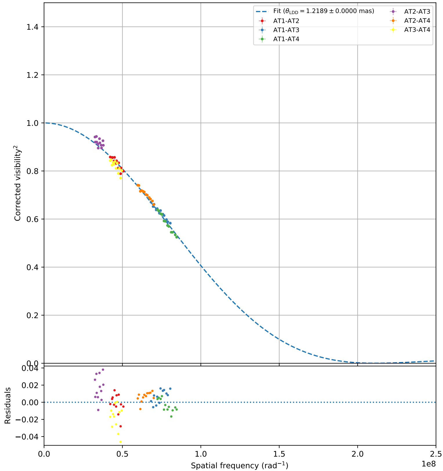
HD142860 (faint, 105)
