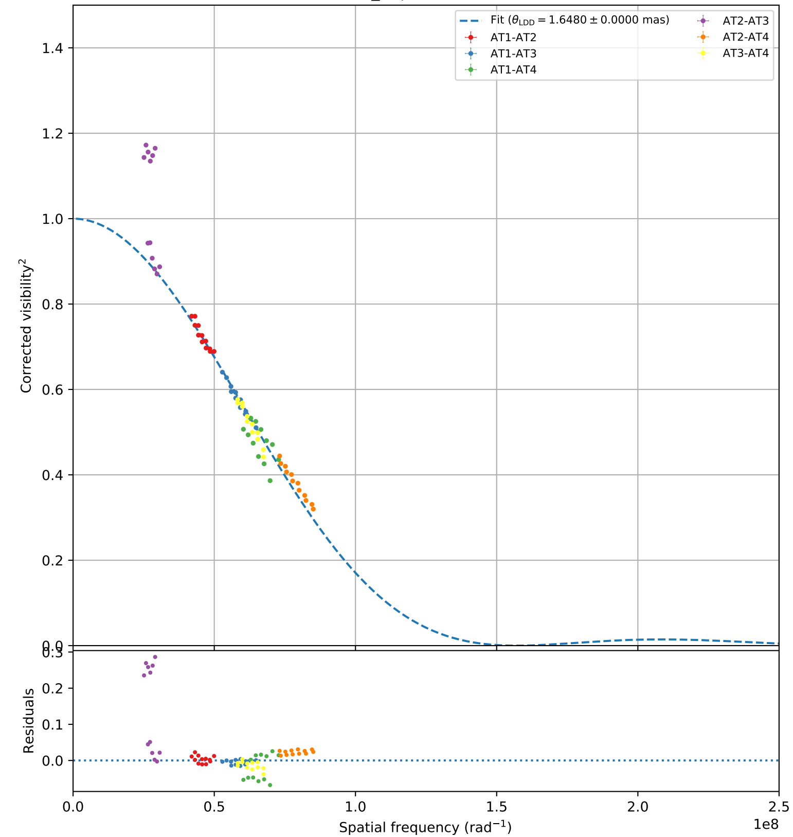
rho_Pup (faint, 106)
