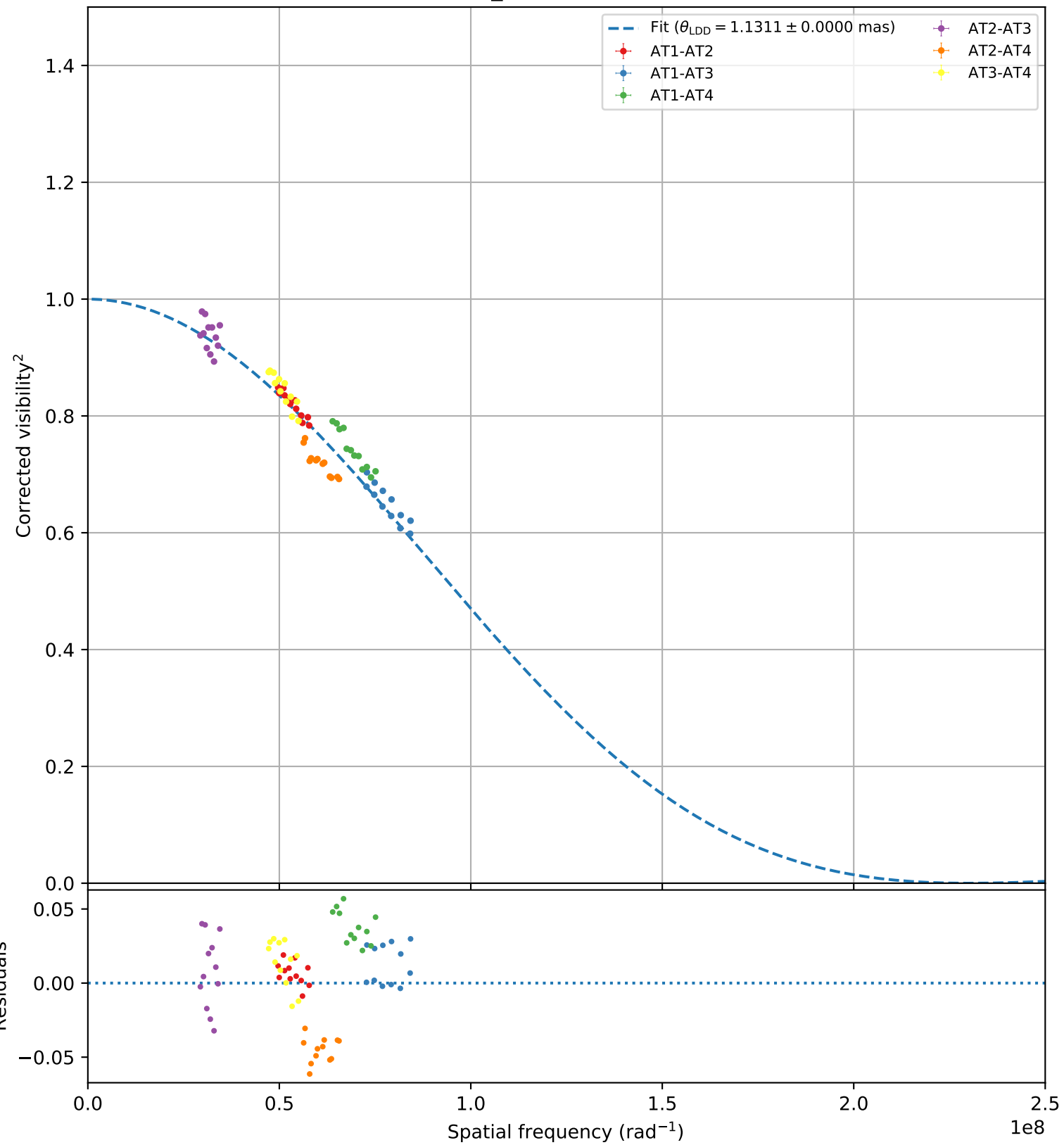
zet_Tuc (faint, 104)
