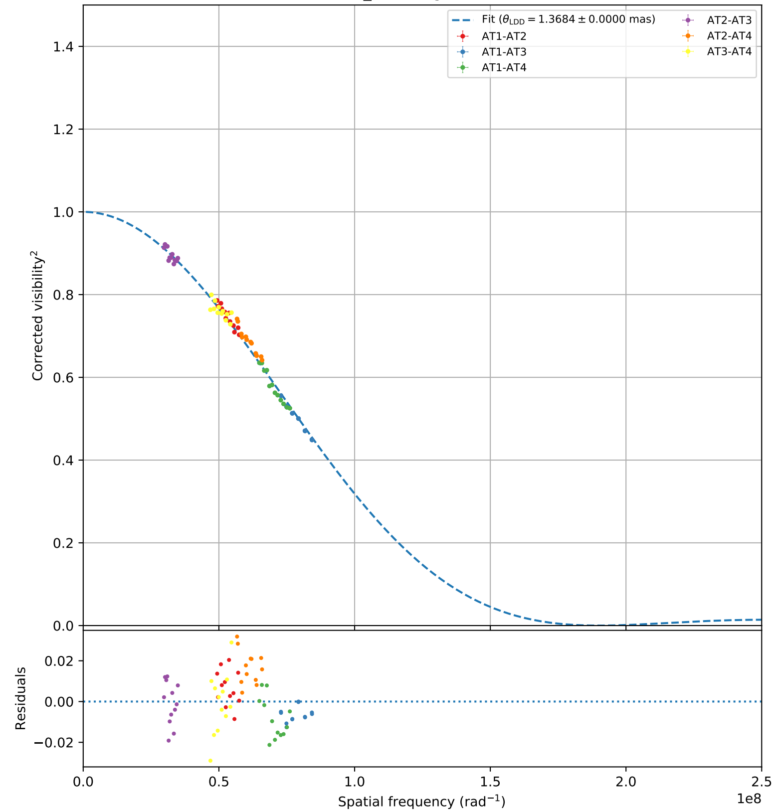
zet_Tuc (bright, 104)
