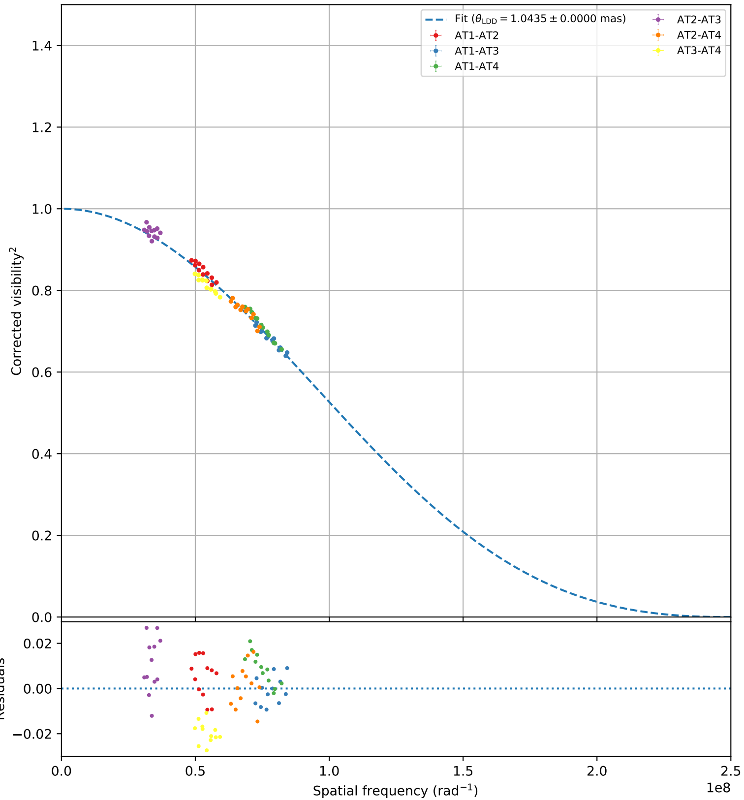
HD141004 (faint, 105)
