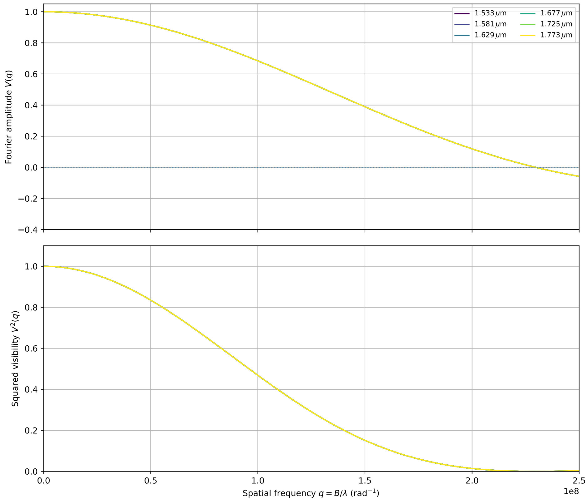
HD124850: fitted \theta_{\text{LDD}} = 1.1334 \pm 0.0000 mas
