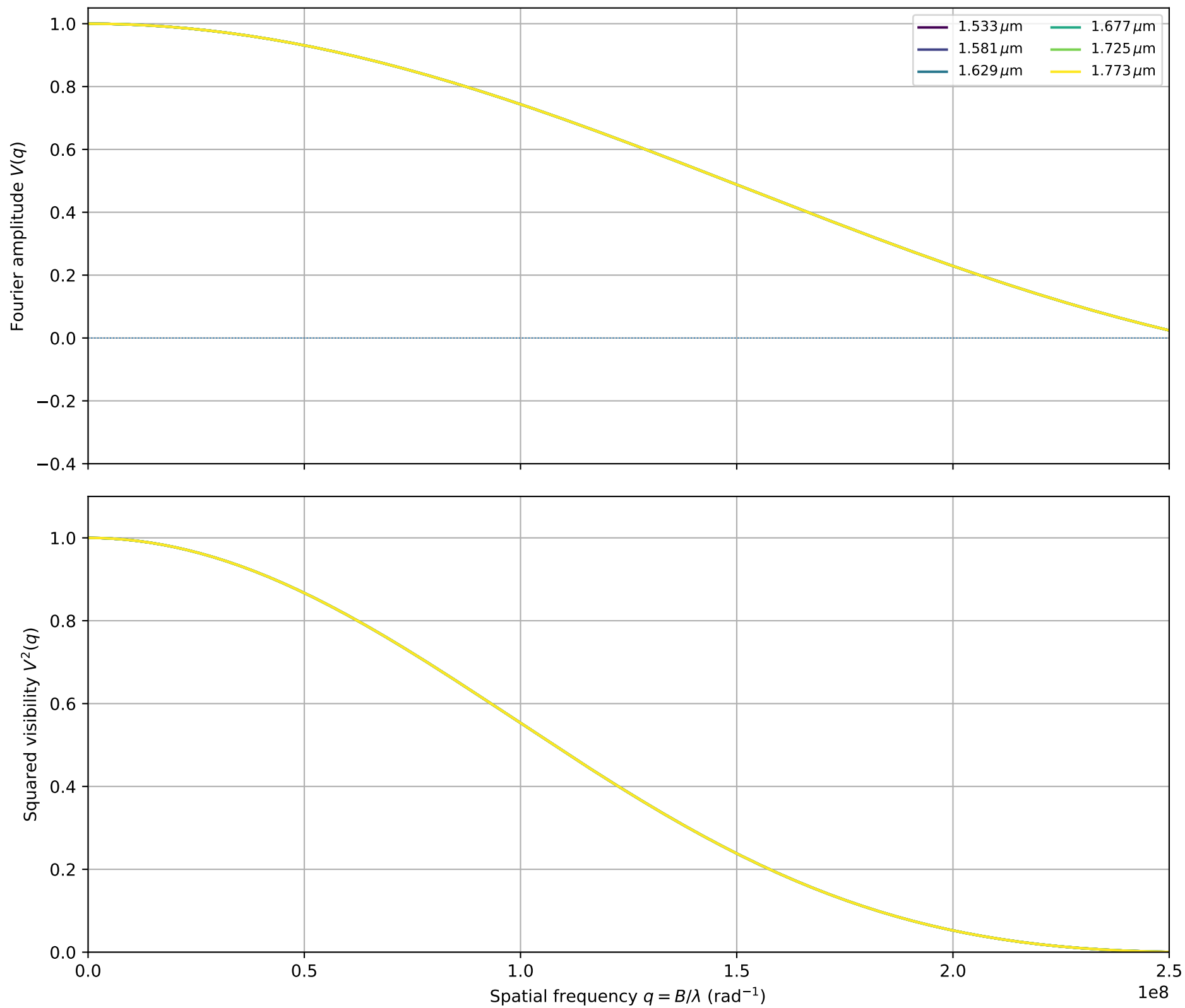
HR_2998: fitted \theta_{\text{LDD}} = 1.0062 \pm 0.0000 mas
