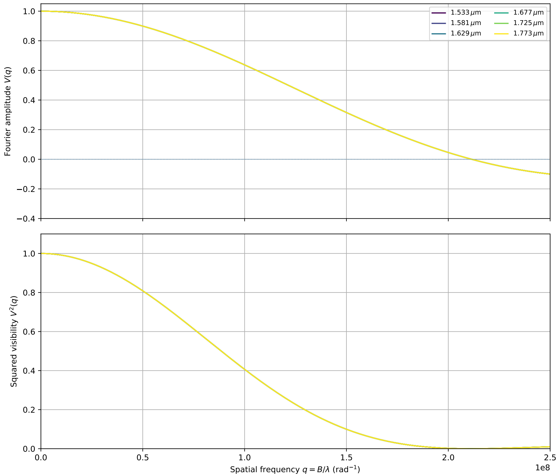
HD142860: fitted \theta_{\text{LDD}} = 1.2189 \pm 0.0000 mas
