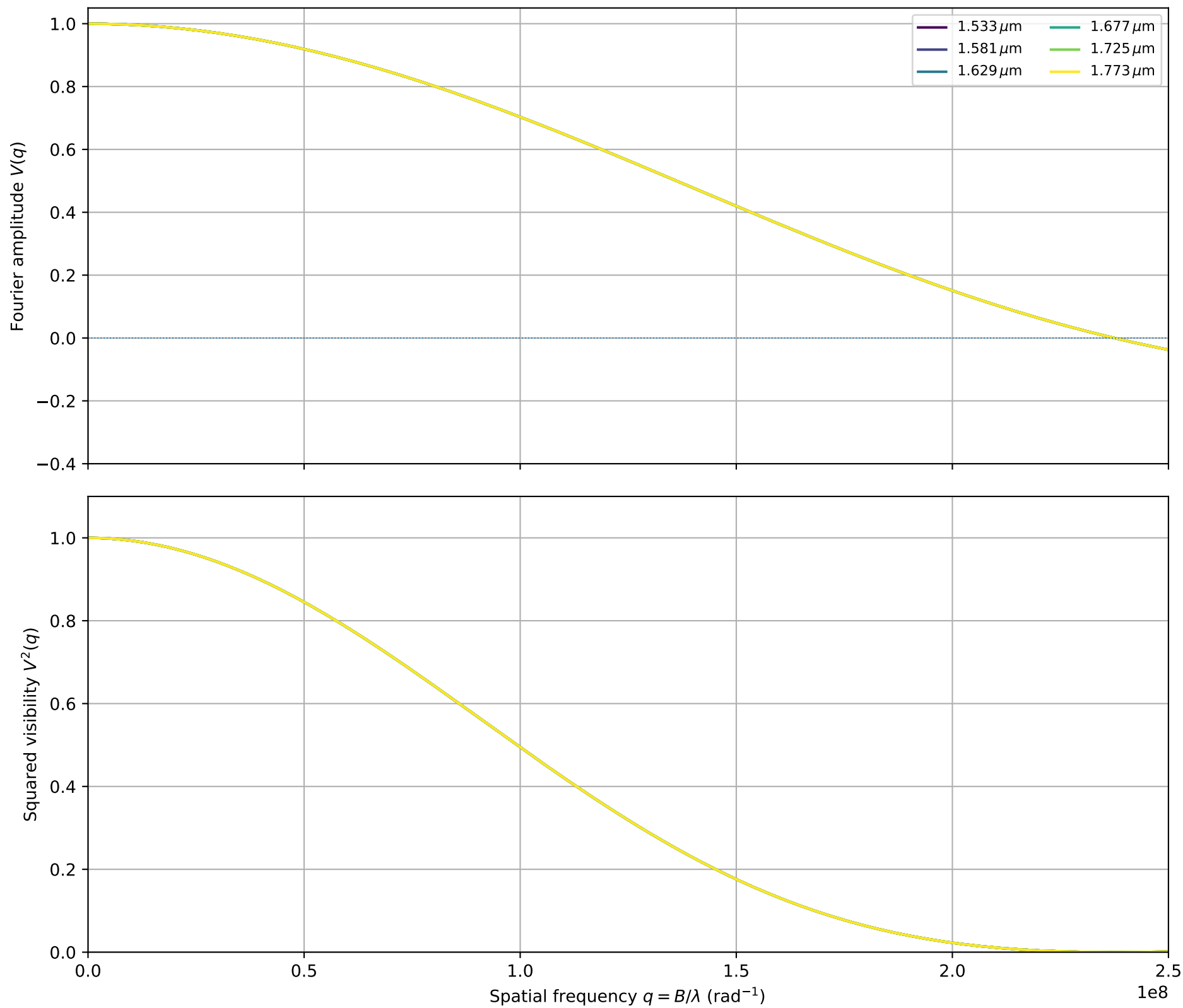
HD141004: fitted \theta_{\text{LDD}} = 1.0905 \pm 0.0000 mas
