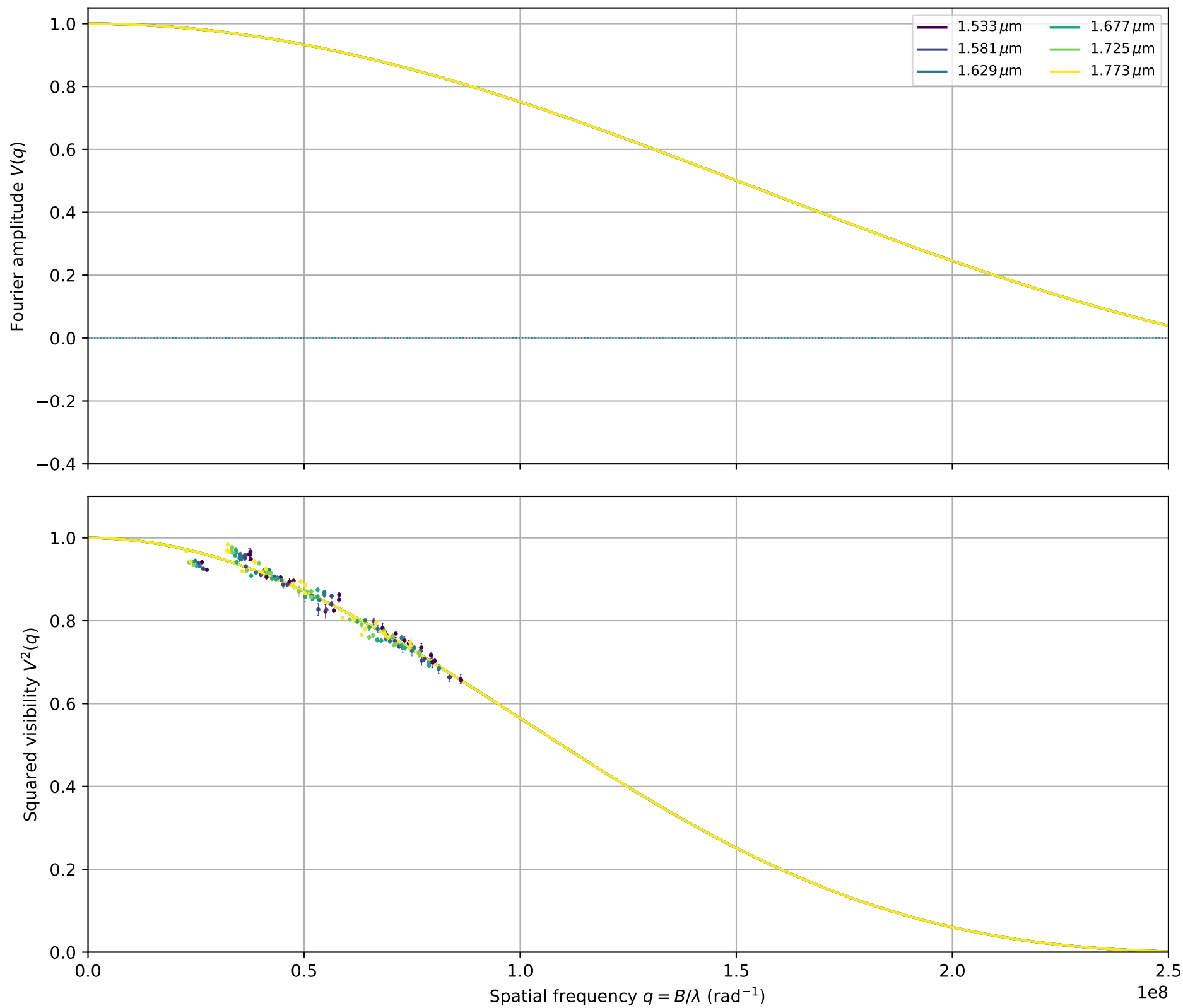
HR_2998: fitted \theta_{\text{LDD}} = 0.9917 \pm 0.0107 mas
