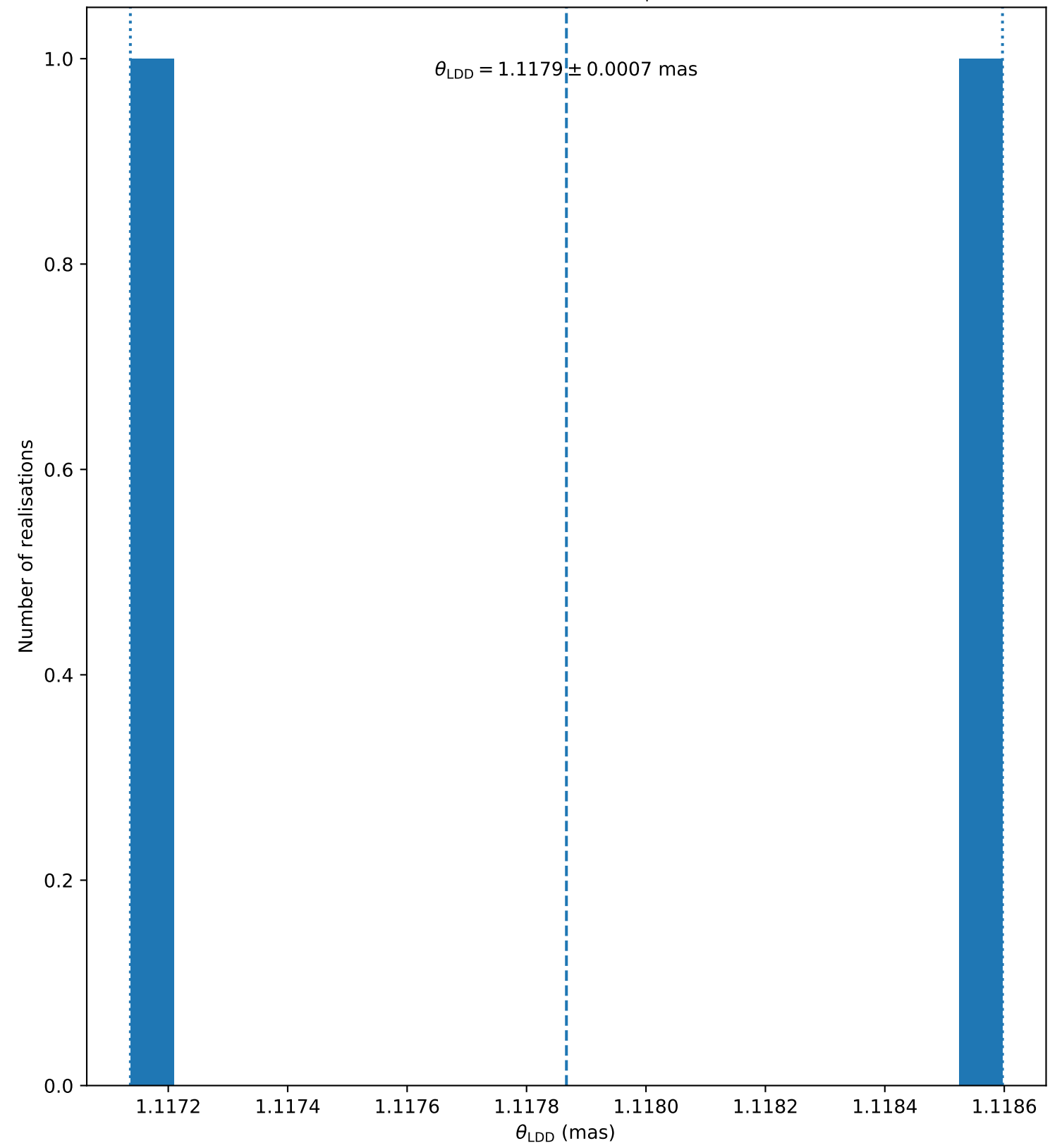
HD124850 ( N_{\text{bootstrap}} = 2 )
