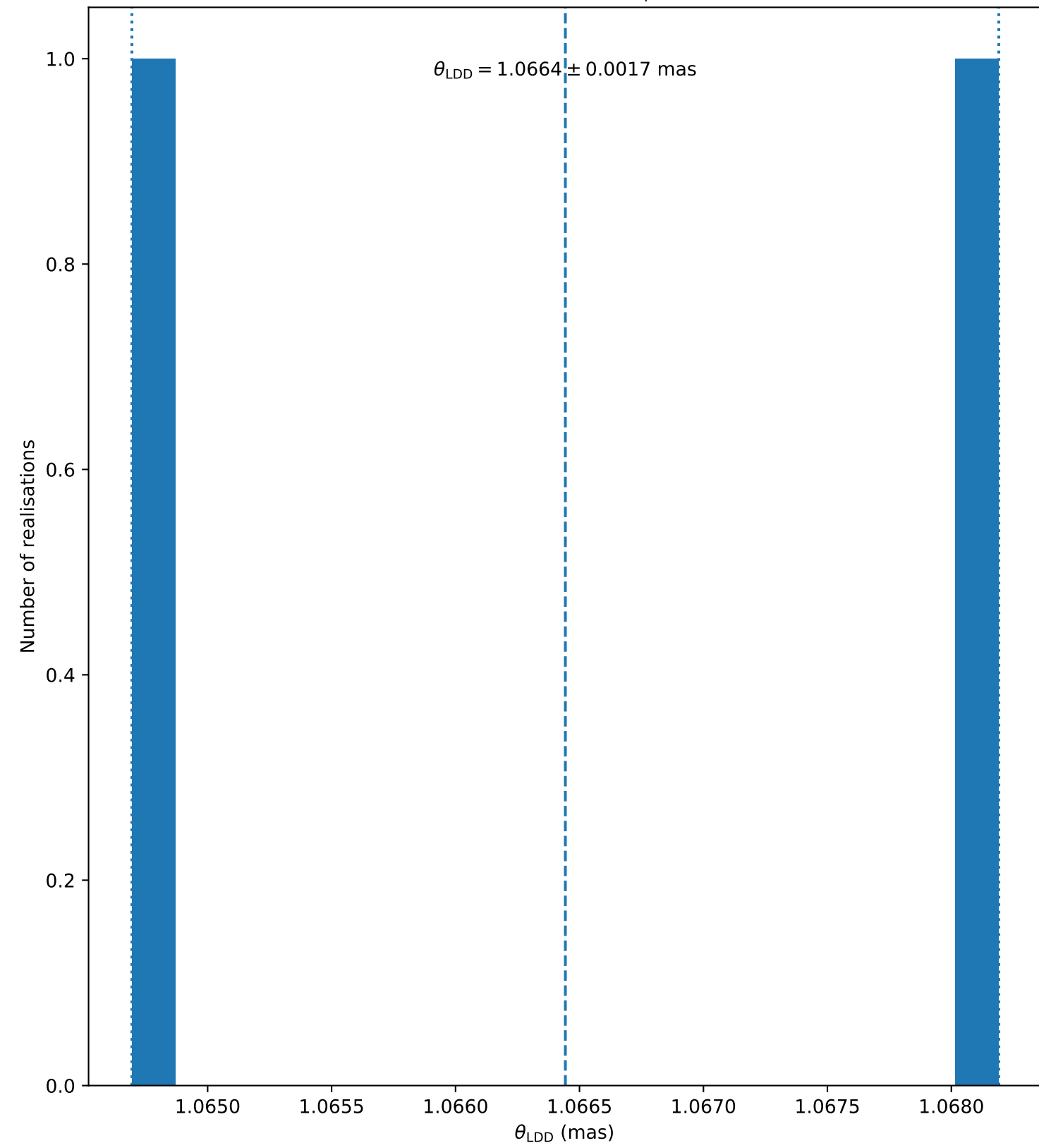
HD141004 ( N_{\text{bootstrap}} = 2 )
