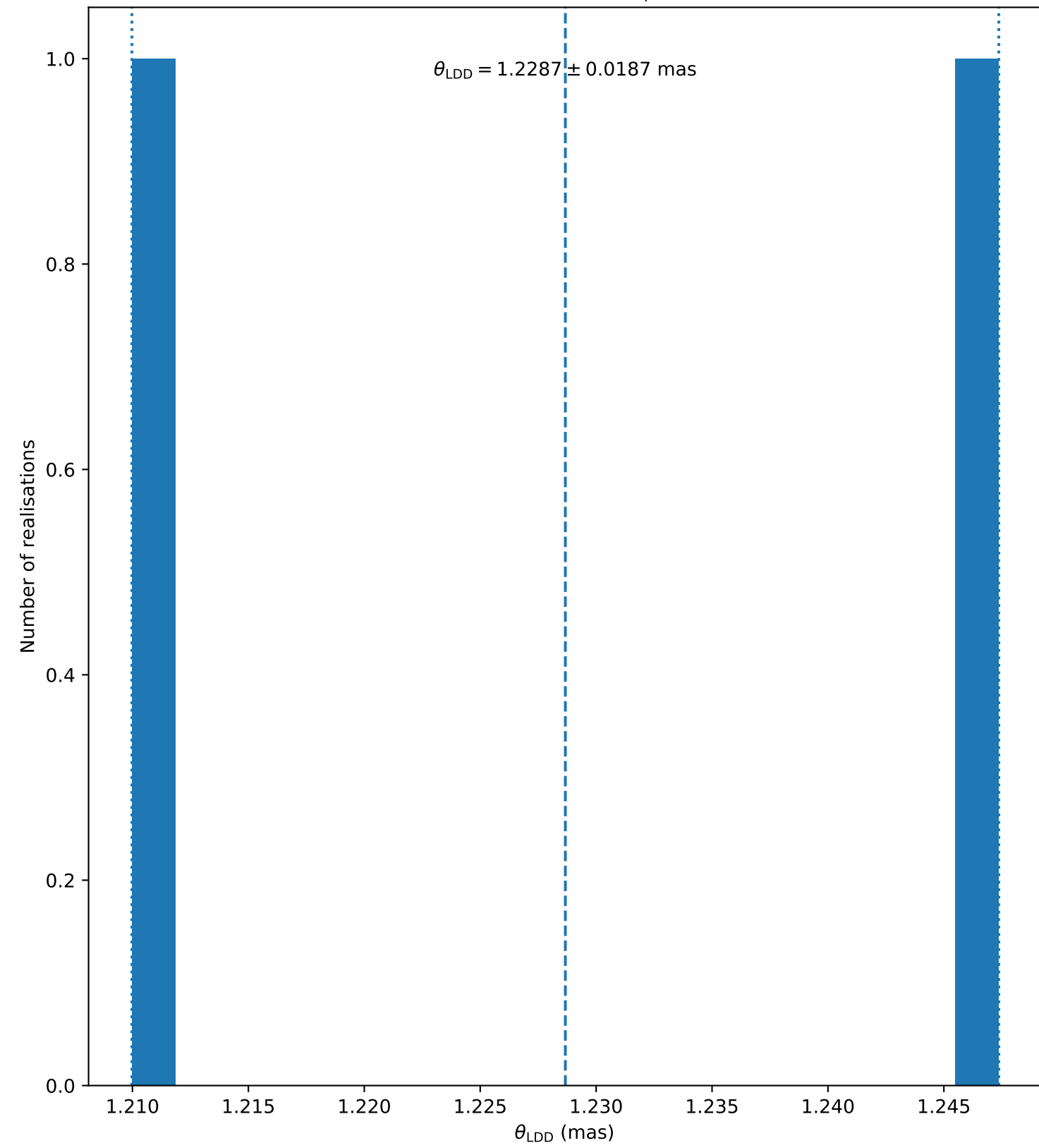
HD142860 ( N_{\text{bootstrap}} = 2 )
