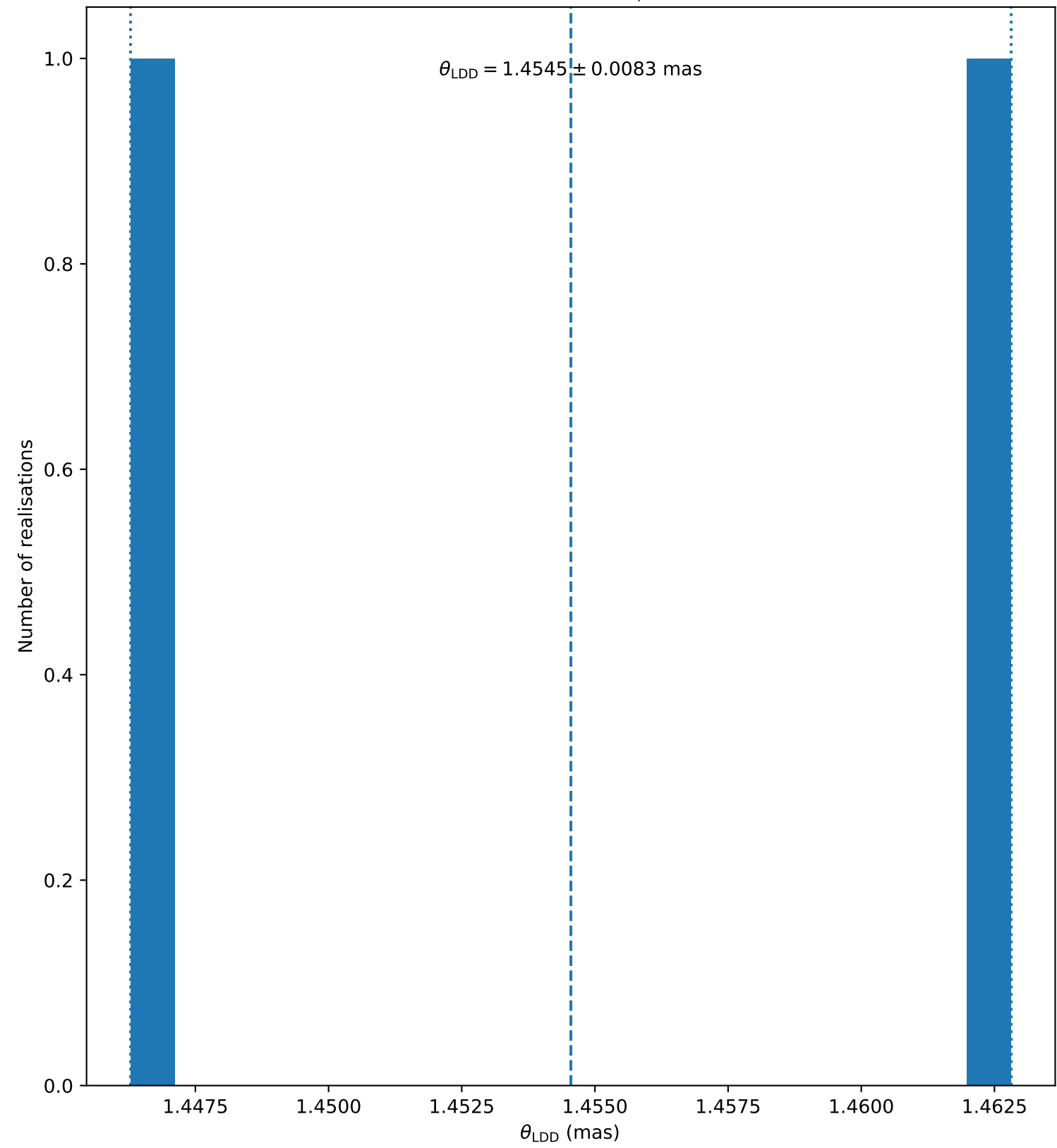
ksi_Gem ( N_{\text{bootstrap}} = 2 )
