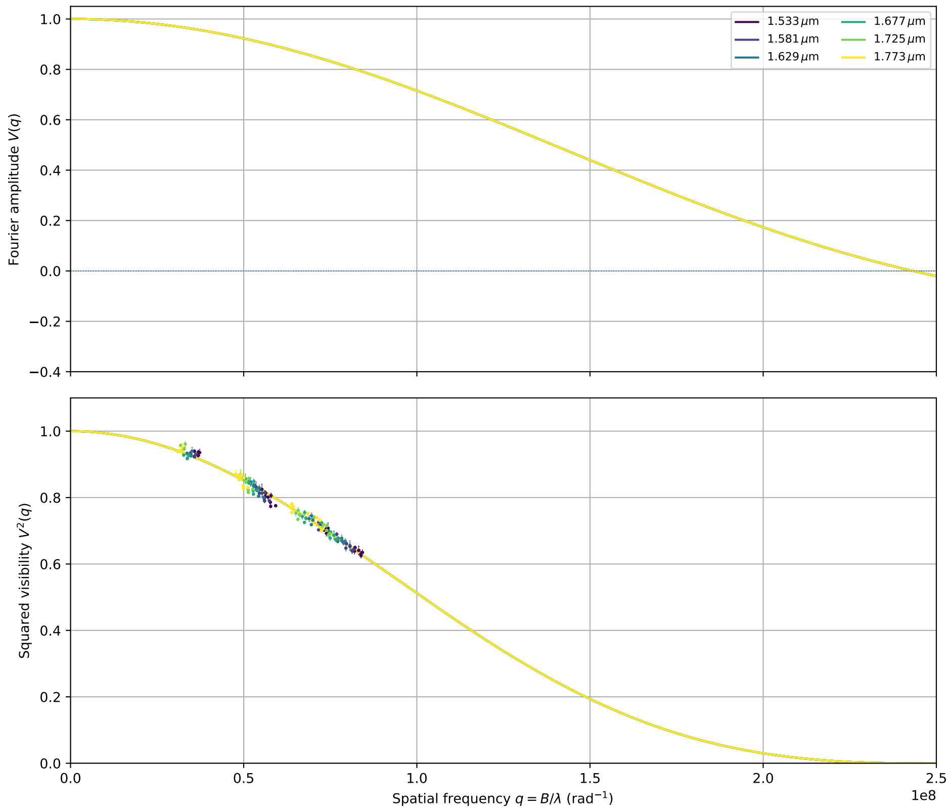
HD141004: fitted \theta_{\text{LDD}} = 1.0664 \pm 0.0017 mas
