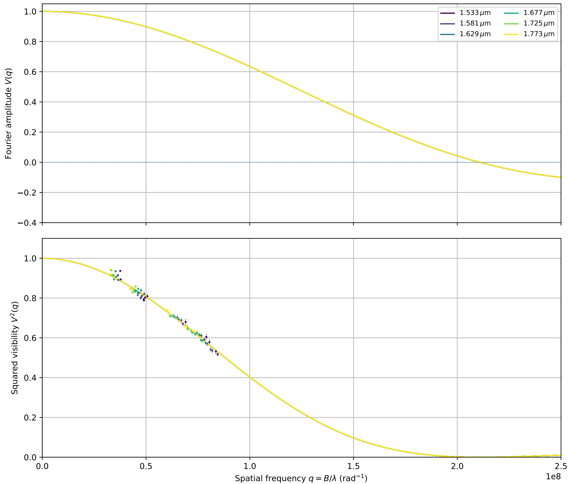
HD142860: fitted \theta_{\text{LDD}} = 1.2287 \pm 0.0187 mas
