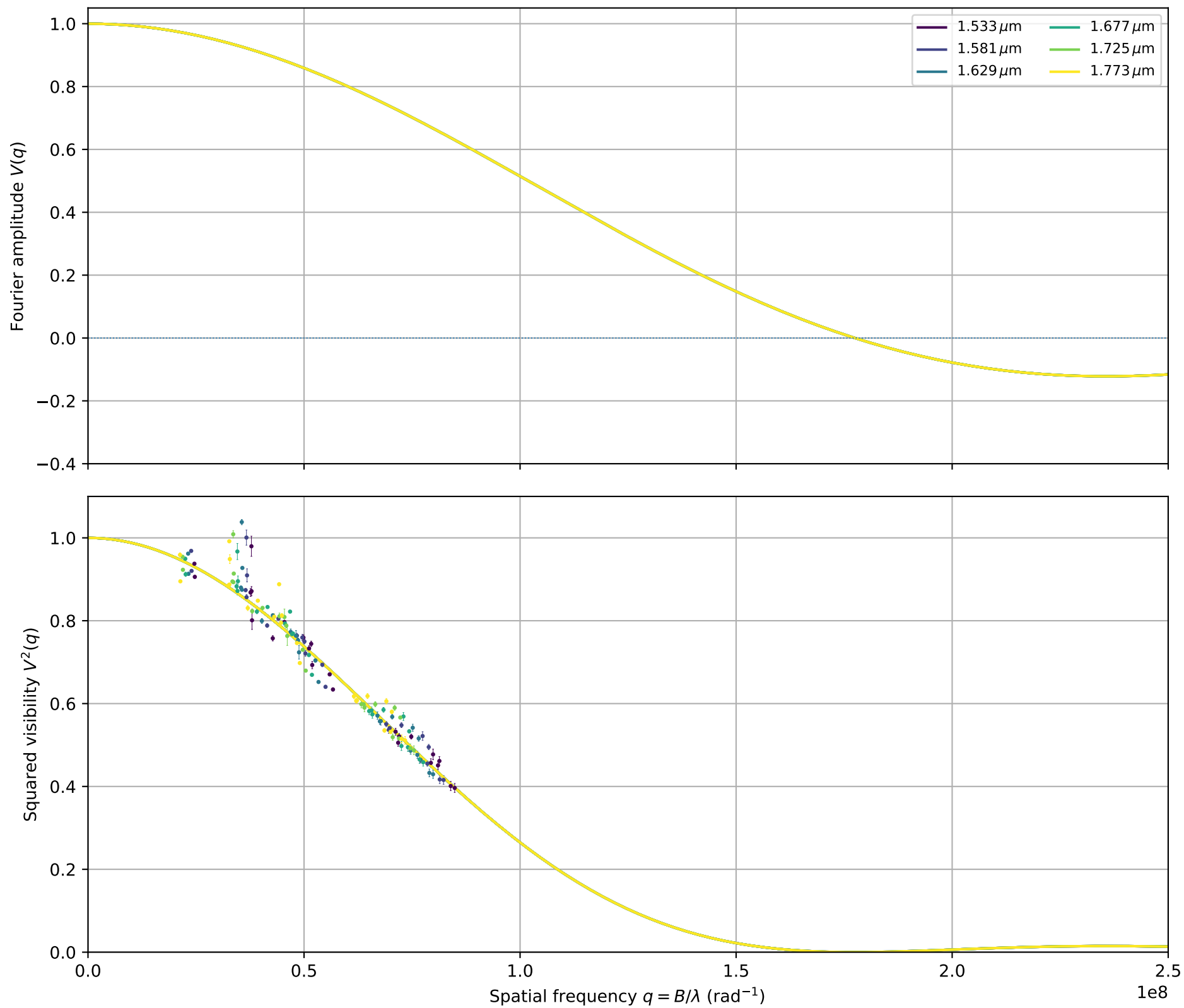
ksi_Gem: fitted \theta_{\text{LDD}} = 1.4545 \pm 0.0083 mas
