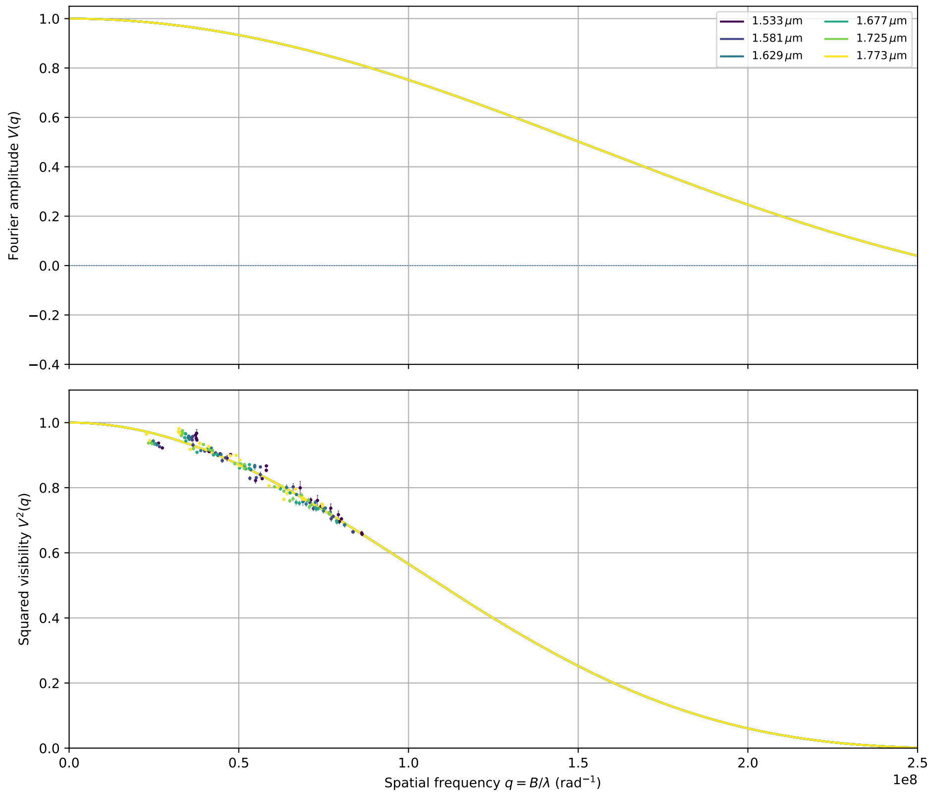
HR_2998: fitted \theta_{\text{LDD}} = 0.9888 \pm 0.0085 mas
