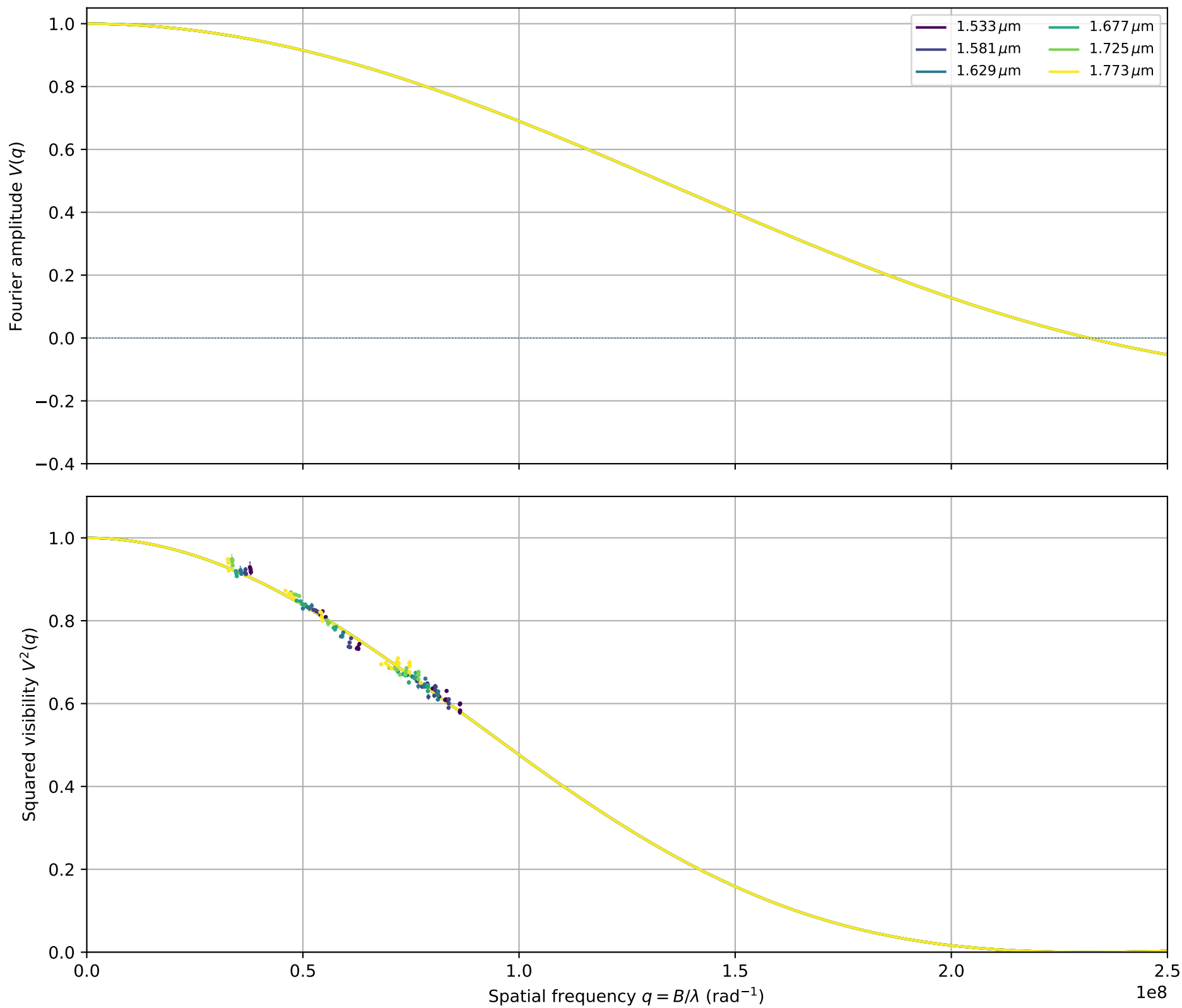
HD124850: fitted \theta_{\text{LDD}} = 1.1179 \pm 0.0007 mas
