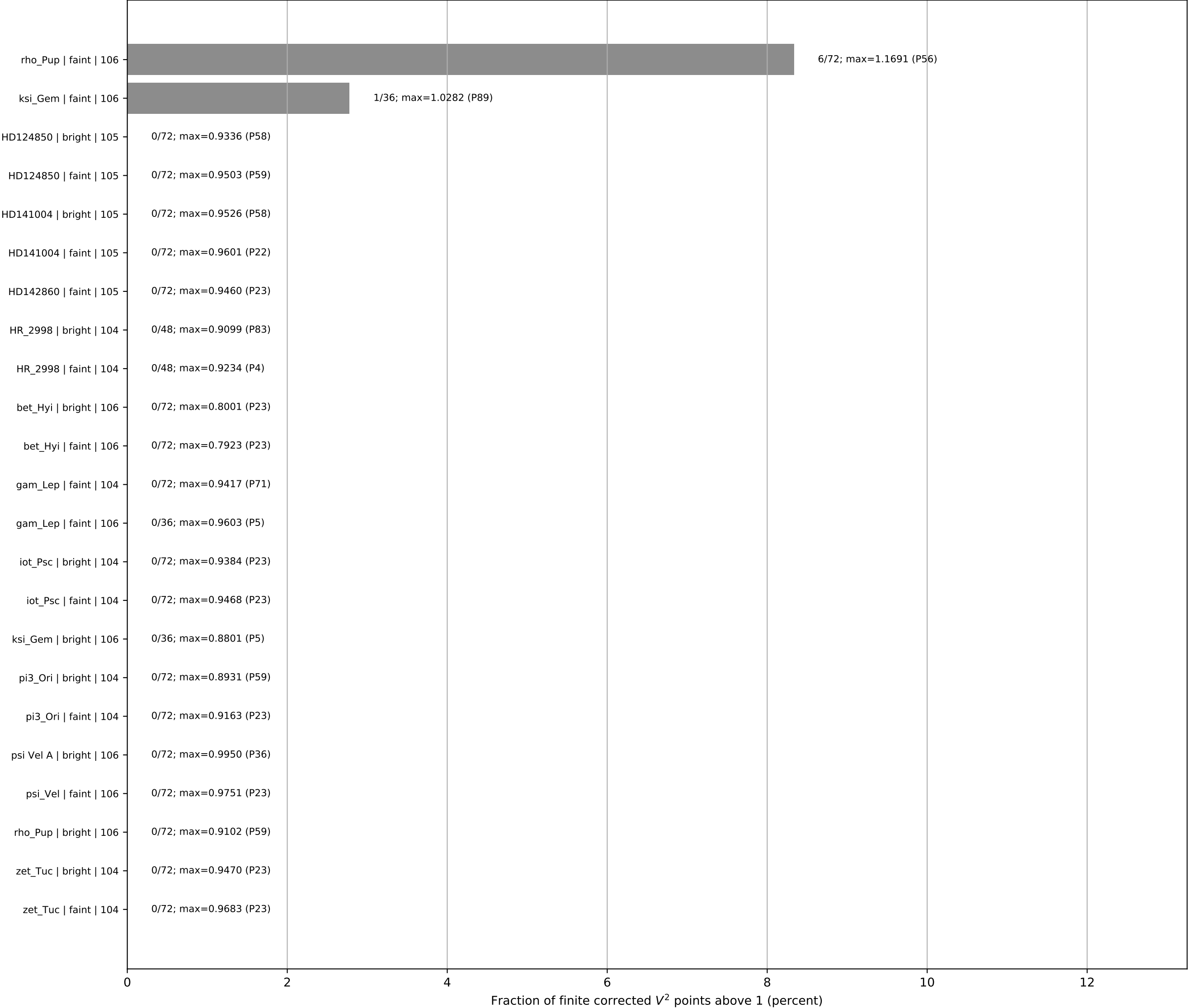
Corrected V^2 > 1 overview Labels show N(V^2 > 1)/N(\text{total}) , maximum V^2 and maximum point
