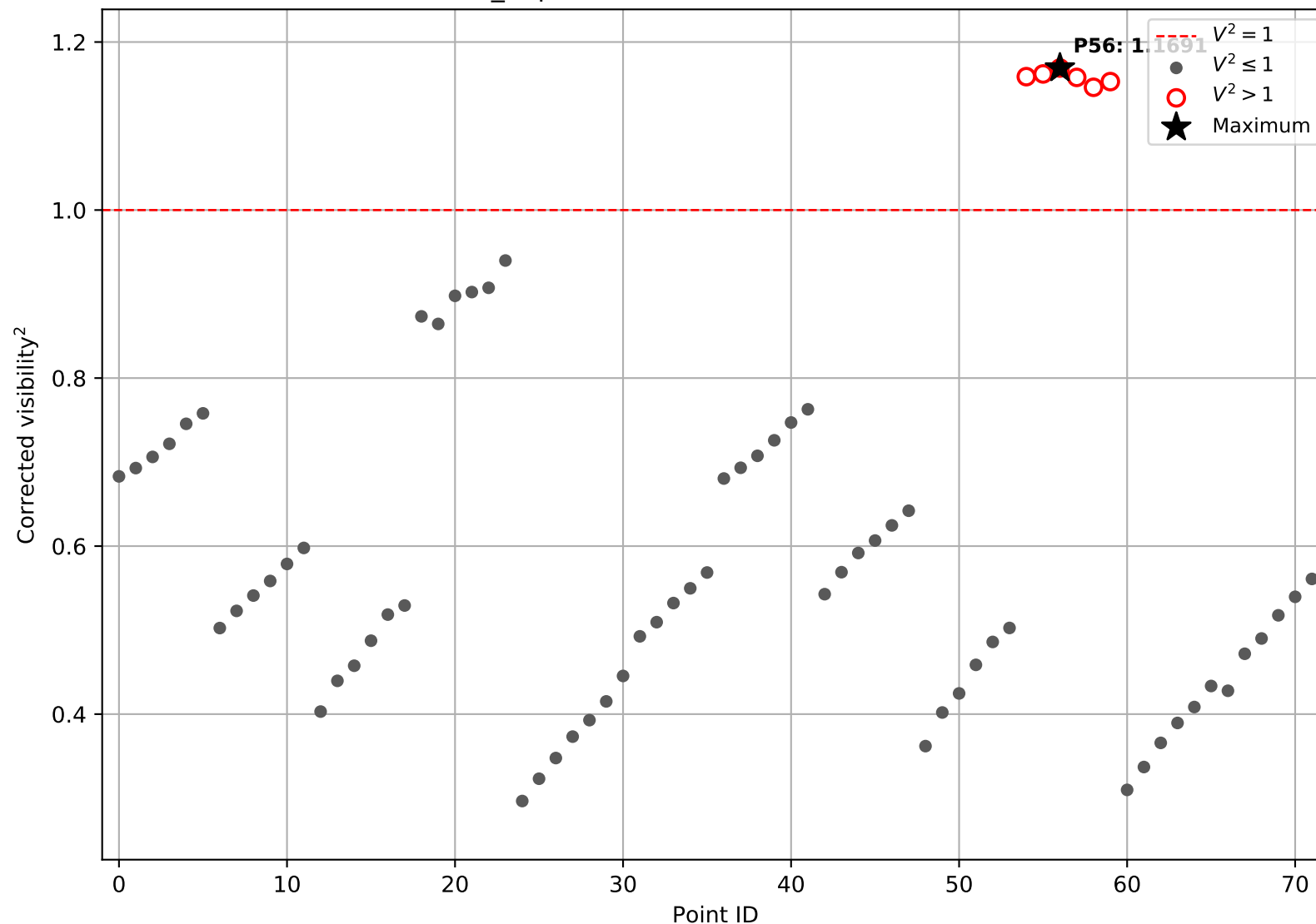
rho_Pup, faint, 106: corrected V2 values
